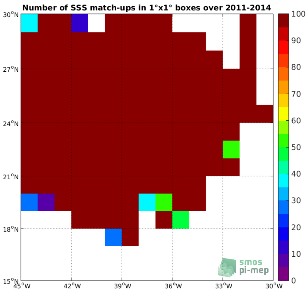
Figure 3: Number of SSS match-ups between Surface drifters SSS and the SMOS-L3-CATDS-CECOS-LOCEAN-V3-18DAYS-25KM SSS product for the SPURS 1 Pi-MEP region over 1°x1° boxes and for the full satellite product period.
