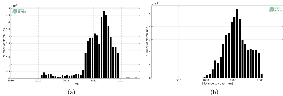
Figure 1: Number of match-ups between Surface drifters and SMOS-L3-CATDS-CECOS-LOCEAN-V3-18DAYS-25KM SSS as a function of time (a) and as function of the distance to coast (b) over the SPURS 1 Pi-MEP region and for the full satellite product period.
