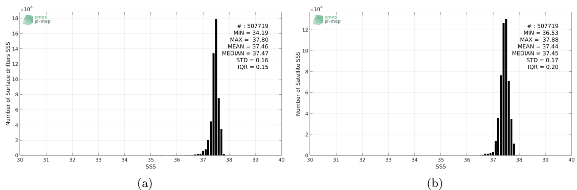
Figure 2: Histograms of SSS from Surface drifters (a) and SMOS-L3-CATDS-CECOS-LOCEAN-V3-18DAYS-25KM (b) considering all match-up pairs per bins of 0.1 over the SPURS 1 Pi-MEP region and for the full satellite product period.
