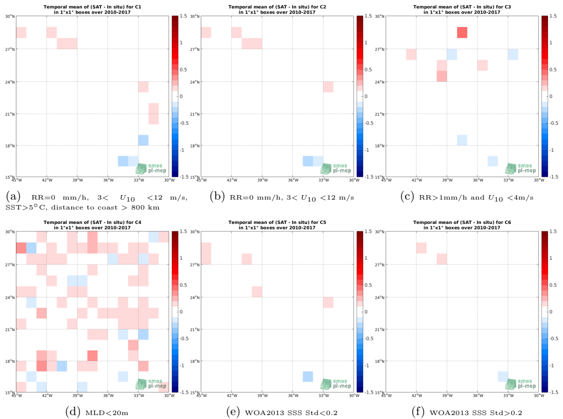
Figure 12: Temporal mean gridded over spatial boxes of size 1^\circ \times 1^\circ of \Delta SSS (SMOS-L3-CATDS-CECOS-LOCEAN-V3-18DAYS-25KM - Argo) for 6 different subdatasets corresponding to:RR=0 mm/h, 3 < U_{10} < 12 m/s, SST >5^\circ C, distance to coast > 800 km (a), RR=0 mm/h, 3 < U_{10} < 12 m/s (b), RR >1 mm/h and U_{10} < 4 m/s (c),MLD <20 m (d),WOA2013 SSS Std <0.2 (e),WOA2013 SSS Std >0.2 (f).
