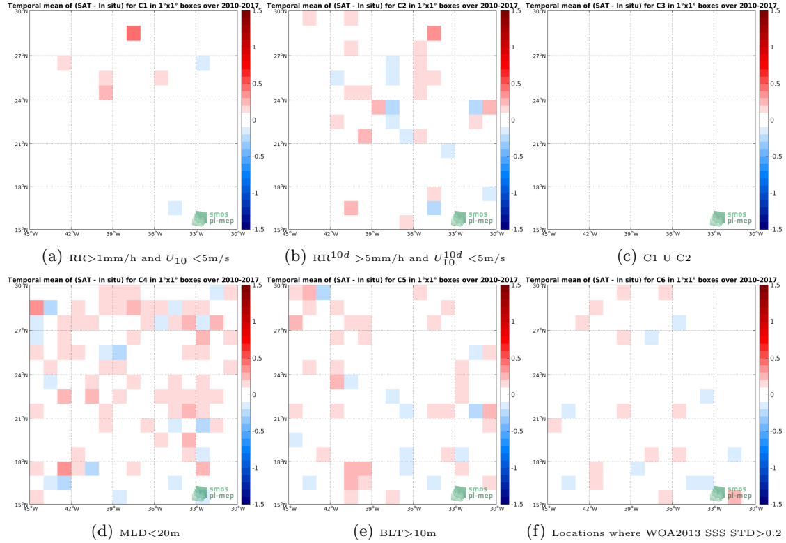
Figure 12: Temporal mean gridded over spatial boxes of size 1^\circ \times 1^\circ of \Delta\text{SSS} (SMOS-L3-CATDS-CECOS-LOCEAN-V3-18DAYS-25KM - Argo) for 6 different subdatasets corresponding to: \text{RR} > 1\text{mm/h} and U_{10} < 5\text{m/s} (a), \text{RR}^{10d} > 5\text{mm/h} and U_{10}^{10d} < 5\text{m/s} (b), C1 U C2 (c), \text{MLD} < 20\text{m} (d), \text{BLT} > 10\text{m} (e), Locations where WOA2013 SSS STD > 0.2 (f).
