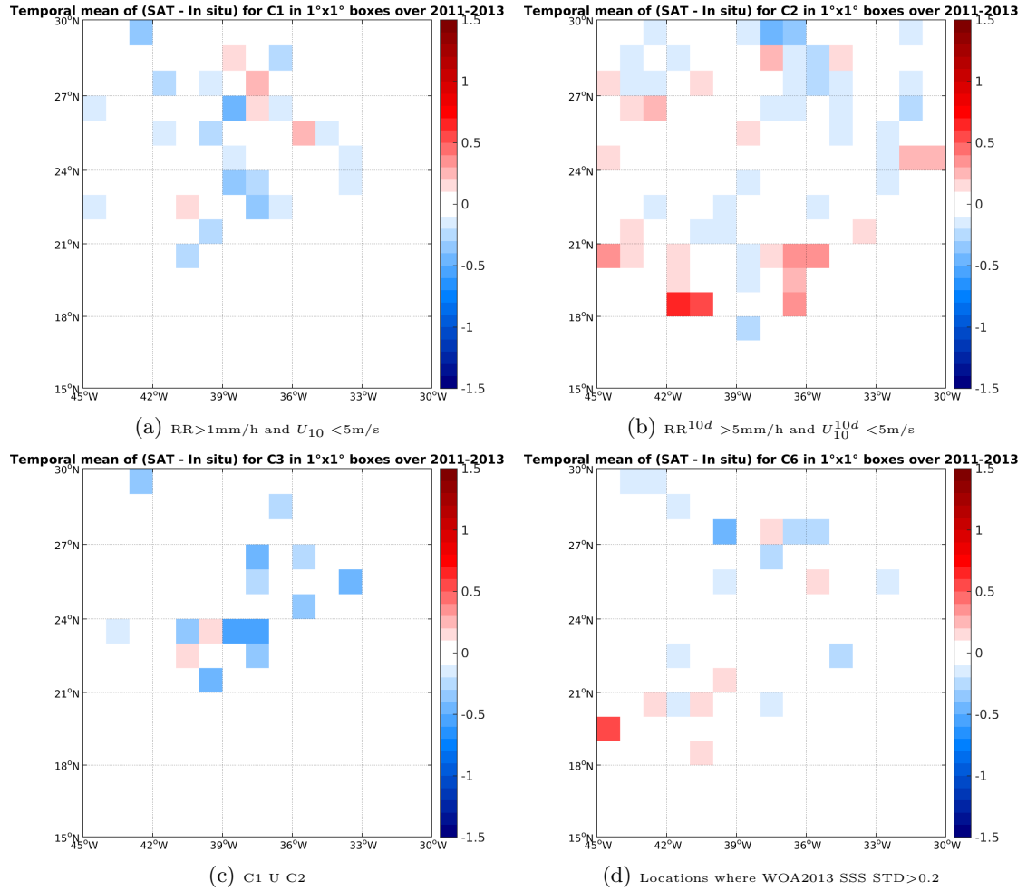
Figure 11: Temporal mean gridded over spatial boxes of size 1^\circ \times 1^\circ of \Delta SSS (SMOS-L3-CATDS-CECOS-LOCEAN-V2.1-9DAYS-25KM - Surface drifters) for 4 different subdatasets corresponding to: RR > 1\text{mm/h} and U_{10} < 5\text{m/s} (a), RR^{10d} > 5\text{mm/h} and U_{10}^{10d} < 5\text{m/s} (b), C1 U C2 (c), Locations where WOA2013 SSS STD > 0.2 (d).
