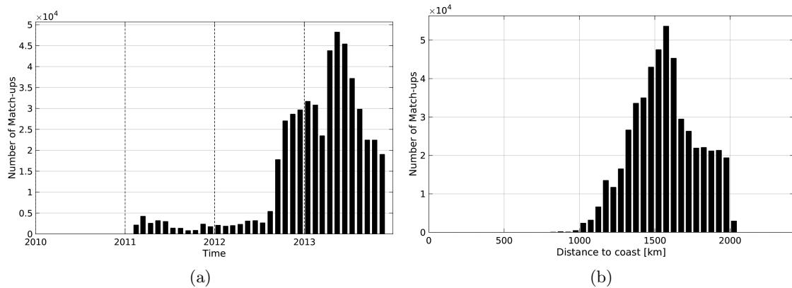
Figure 1: Number of match-ups between Surface drifters and SMOS-L3-CATDS-CECOS-LOCEAN-V2.1-9DAYS-25KM SSS as a function of time (a) and as function of the distance to coast (b) over the SPURS 1 Pi-MEP region and for the full satellite product period.
