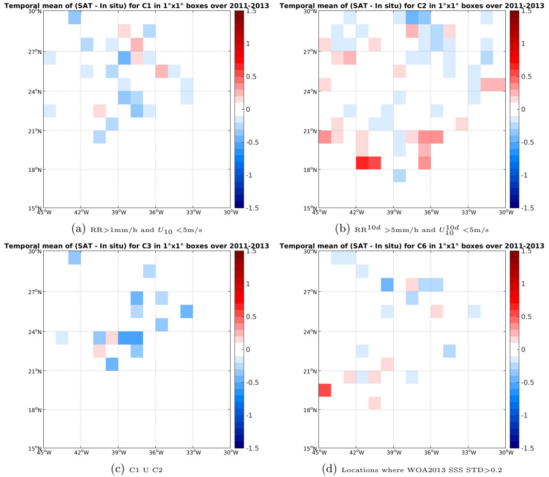
Figure 11: Temporal mean gridded over spatial boxes of size 1°x1° of \Delta SSS (SMOS-L3-CATDS-CECOS-LOCEAN-V2.1-9DAYS-25KM - Surface drifters) for 4 different subdatasets corresponding to: RR > 1\text{mm/h} and U_{10} < 5\text{m/s} (a), RR^{10d} > 5\text{mm/h} and U_{10}^{10d} < 5\text{m/s} (b), C1 U C2 (c), Locations where WOA2013 SSS STD > 0.2 (d).
