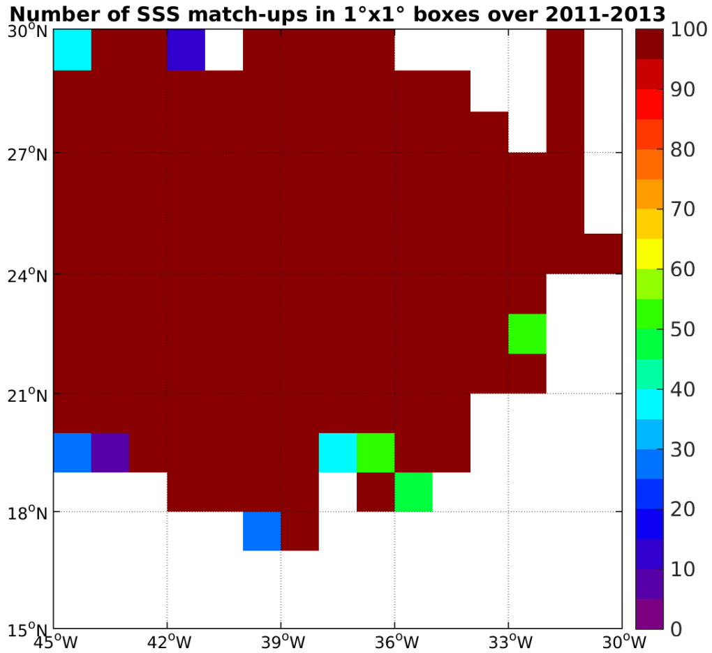
Figure 3: Number of SSS match-ups between Surface drifters SSS and the SMOS-L3-CATDS-CECOS-LOCEAN-V2.1-9DAYS-25KM SSS product for the SPURS 1 Pi-MEP region over 1°x1° boxes and for the full satellite product period.
