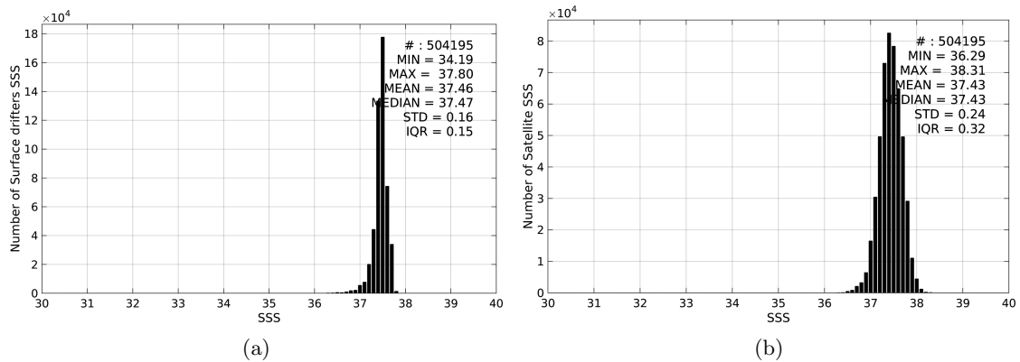
Figure 2: Histograms of SSS from Surface drifters (a) and SMOS-L3-CATDS-CECOS-LOCEAN-V2.1-9DAYS-25KM (b) considering all match-up pairs per bins of 0.1 over the SPURS 1 Pi-MEP region and for the full satellite product period.
