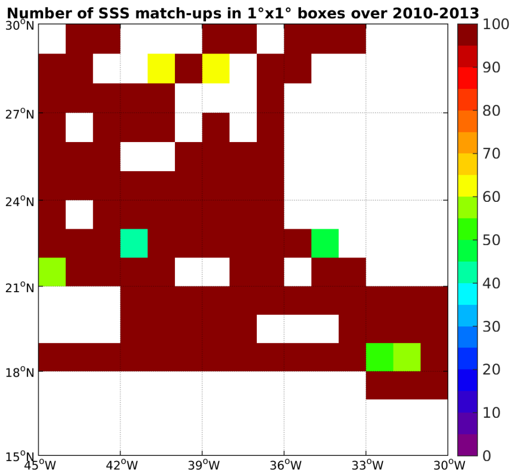
Figure 4: Number of SSS match-ups between TSG-SAMOS SSS and the SMOS-L3-CATDS-CECOS-LOCEAN-V2-9DAYS-25KM SSS product for the SPURS 1 Pi-MEP region over 1°x1° boxes and for the full satellite product period.
