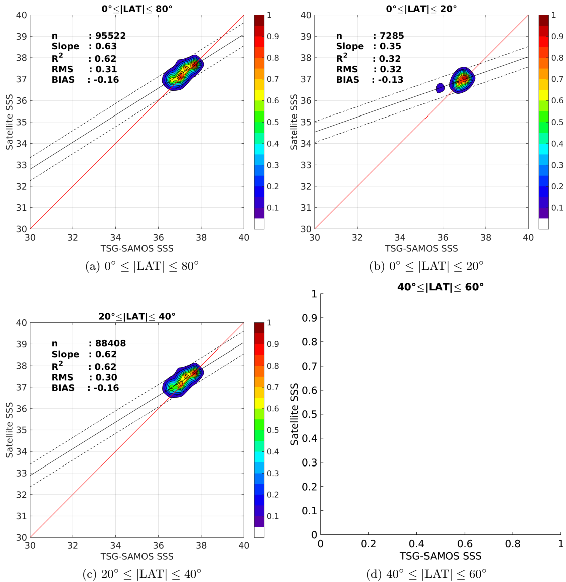
Figure 9: Contour maps of the concentration of SMOS-L3-CATDS-CECOS-LOCEAN-V2-9DAYS-25KM SSS (y-axis) versus TSG-SAMOS SSS (x-axis) at match-up pairs for different latitude bands. For each plot, the red line shows x=y . The black thin and dashed lines indicate a linear fit through the data cloud and the \pm 95\% confidence levels, respectively. The number match-up pairs n , the slope and R^2 coefficient of the linear fit, the root mean square (RMS) and the mean bias between satellite and in situ data are indicated for each latitude band in each plots.
