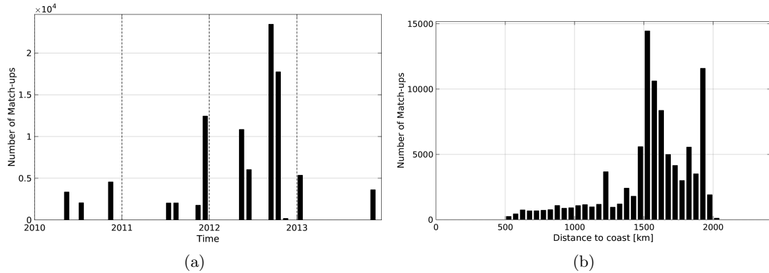
Figure 1: Number of match-ups between TSG-SAMOS and SMOS-L3-CATDS-CECOS-LOCEAN-V2-9DAYS-25KM SSS as a function of time (a) and as function of the distance to coast (b) over the SPURS 1 Pi-MEP region and for the full satellite product period.
