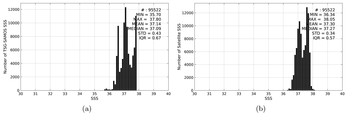
Figure 2: Histograms of SSS from TSG-SAMOS (a) and SMOS-L3-CATDS-CECOS-LOCEAN-V2-9DAYS-25KM (b) considering all match-up pairs per bins of 0.1 over the SPURS 1 Pi-MEP region and for the full satellite product period.
