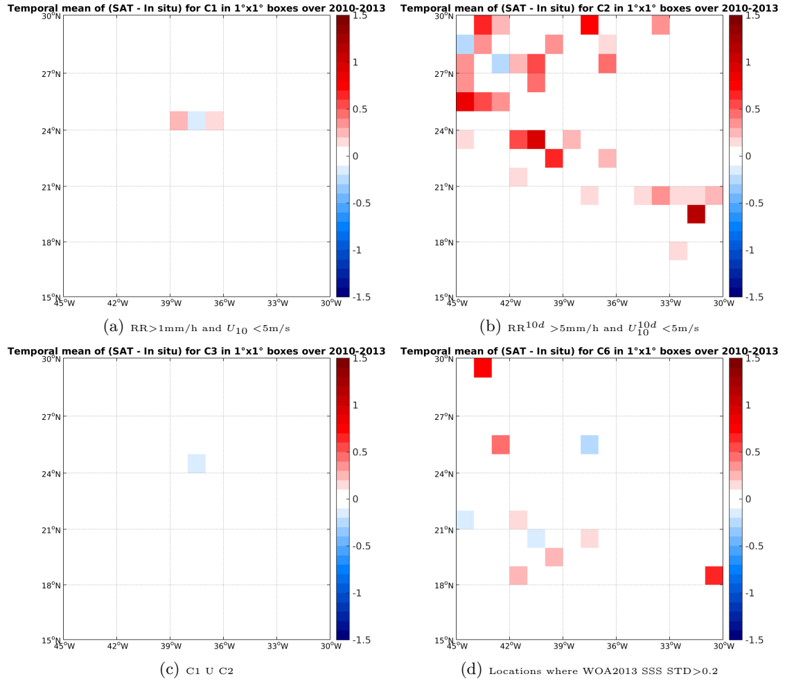
Figure 12: Temporal mean gridded over spatial boxes of size 1^\circ \times 1^\circ of \Delta SSS (SMOS-L3-CATDS-CECOS-LOCEAN-V2-9DAYS-25KM - TSG-SAMOS) for 4 different subdatasets corresponding to: RR > 1\text{mm/h} and U_{10} < 5\text{m/s} (a), RR^{10d} > 5\text{mm/h} and U_{10}^{10d} < 5\text{m/s} (b), C1 U C2 (c), Locations where WOA2013 SSS STD > 0.2 (d).
