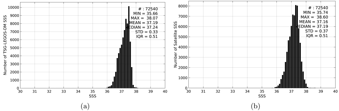
Figure 2: Histograms of SSS from TSG-LEGOS-DM (a) and SMOS-L3-CATDS-CECOS-LOCEAN-V2-9DAYS-25KM (b) considering all match-up pairs per bins of 0.1 over the SPURS 1 Pi-MEP region and for the full satellite product period.
