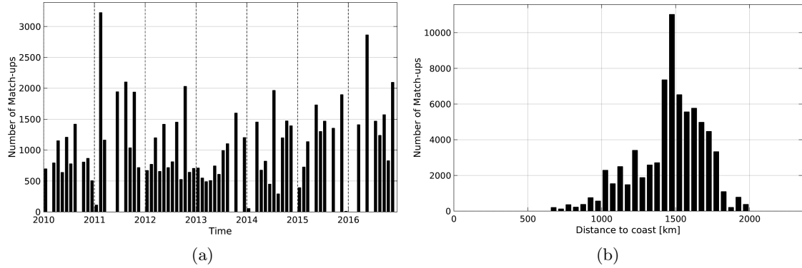
Figure 1: Number of match-ups between TSG-LEGOS-DM and SMOS-L3-CATDS-CECOS-LOCEAN-V2-9DAYS-25KM SSS as a function of time (a) and as function of the distance to coast (b) over the SPURS 1 Pi-MEP region and for the full satellite product period.
