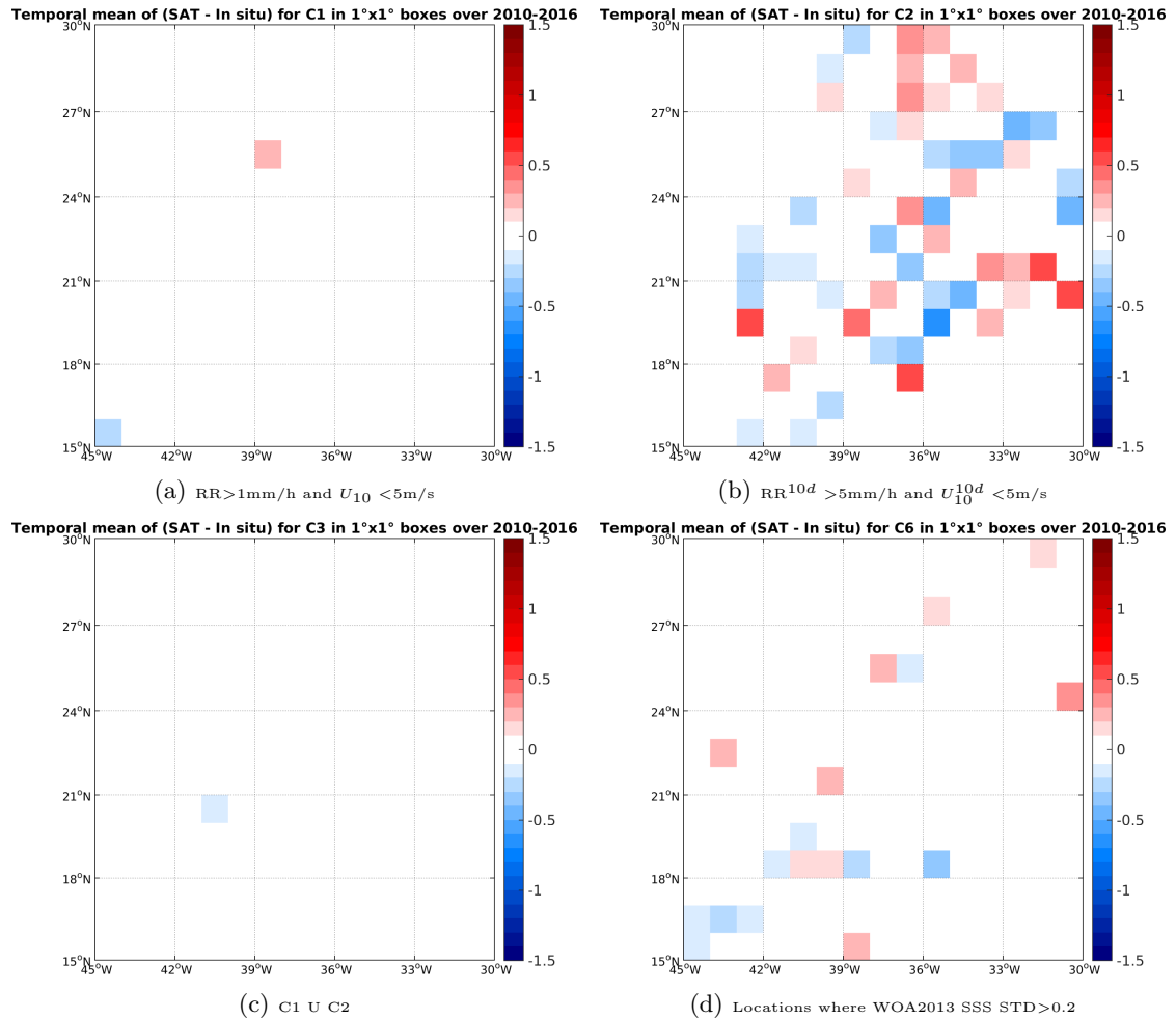
Figure 12: Temporal mean gridded over spatial boxes of size 1^\circ \times 1^\circ of \Delta SSS (SMOS-L3-CATDS-CECOS-LOCEAN-V2-9DAYS-25KM - TSG-LEGOS-DM) for 4 different subdatasets corresponding to: RR > 1 mm/h and U_{10} < 5 m/s (a), RR 10d > 5 mm/h and U_{10}^{10d} < 5 m/s (b), C1 U C2 (c), Locations where WOA2013 SSS STD > 0.2 (d).
