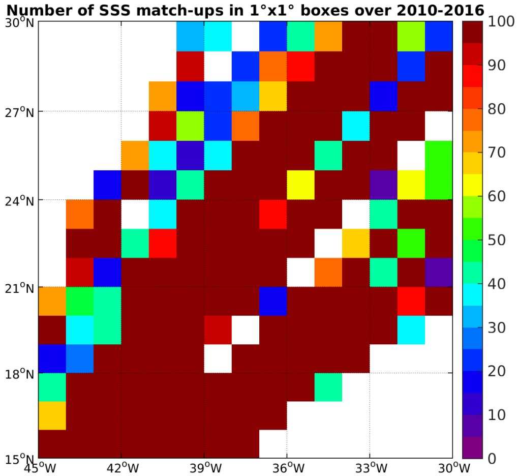
Figure 4: Number of SSS match-ups between TSG-LEGOS-DM SSS and the SMOS-L3-CATDS-CECOS-LOCEAN-V2-9DAYS-25KM SSS product for the SPURS 1 Pi-MEP region over 1°x1° boxes and for the full satellite product period.
