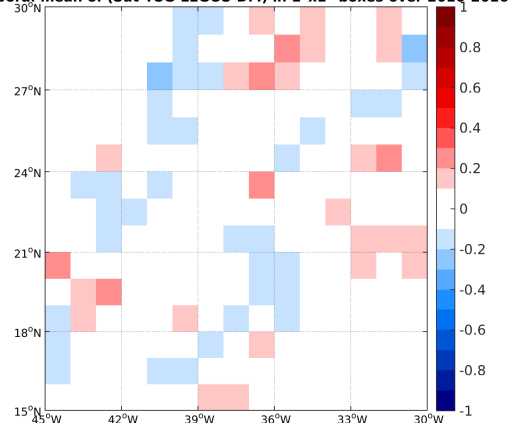
(e) MEAN( \Delta SSS) (Satellite - TSG-LEGOS-DM)
