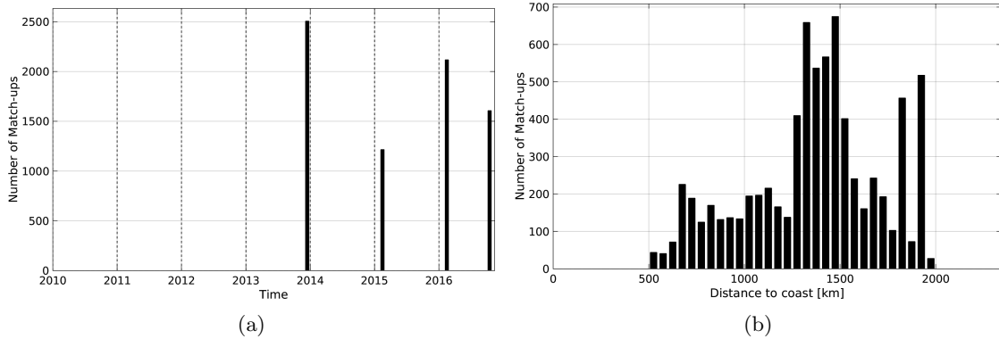
Figure 1: Number of match-ups between TSG-GOSUD-Sailing-ship and SMOS-L3-CATDS-CECOS-LOCEAN-V2-9DAYS-25KM SSS as a function of time (a) and as function of the distance to coast (b) over the SPURS 1 Pi-MEP region and for the full satellite product period.
