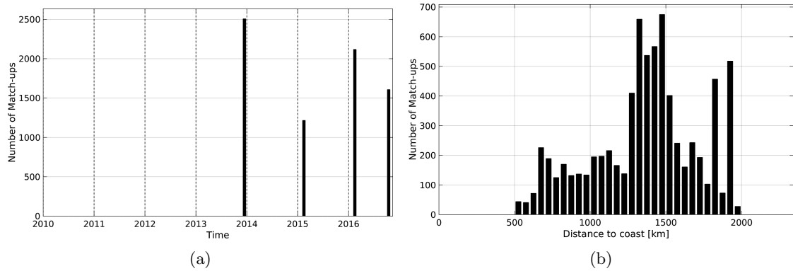
Figure 1: Number of match-ups between TSG-GOSUD-Sailing-ship and SMOS-L3-CATDS-CECOS-LOCEAN-V2-9DAYS-25KM SSS as a function of time (a) and as function of the distance to coast (b) over the SPURS 1 Pi-MEP region and for the full satellite product period.
