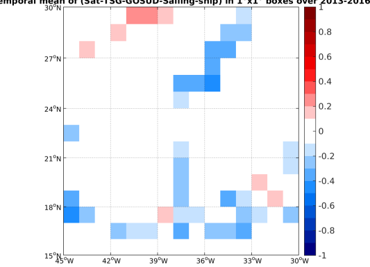
(e) MEAN( \Delta SSS) (Satellite - TSG-GOSUD-Sailing-ship)
