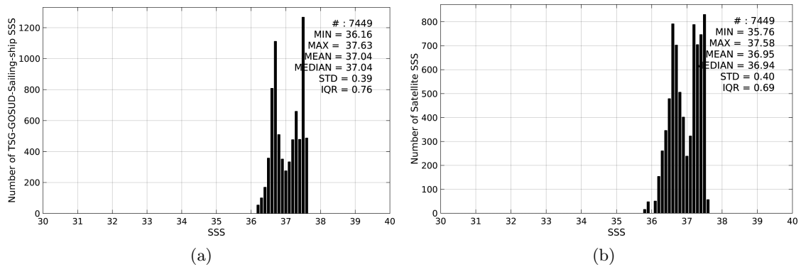
Figure 2: Histograms of SSS from TSG-GOSUD-Sailing-ship (a) and SMOS-L3-CATDS-CECOS-LOCEAN-V2-9DAYS-25KM (b) considering all match-up pairs per bins of 0.1 over the SPURS 1 Pi-MEP region and for the full satellite product period.
