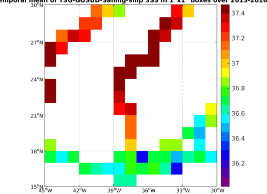
(c) MEAN(TSG-GOSUD-Sailing-ship SSS)
