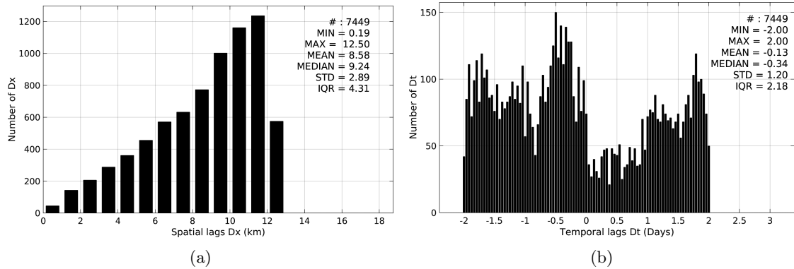
Figure 5: Histograms of the spatial (a) and temporal (b) lags between the time of the TSG-GOSUD-Sailing-ship measurements and the date of the corresponding SMOS-L3-CATDS-CECOS-LOCEAN-V2-9DAYS-25KM SSS product.
