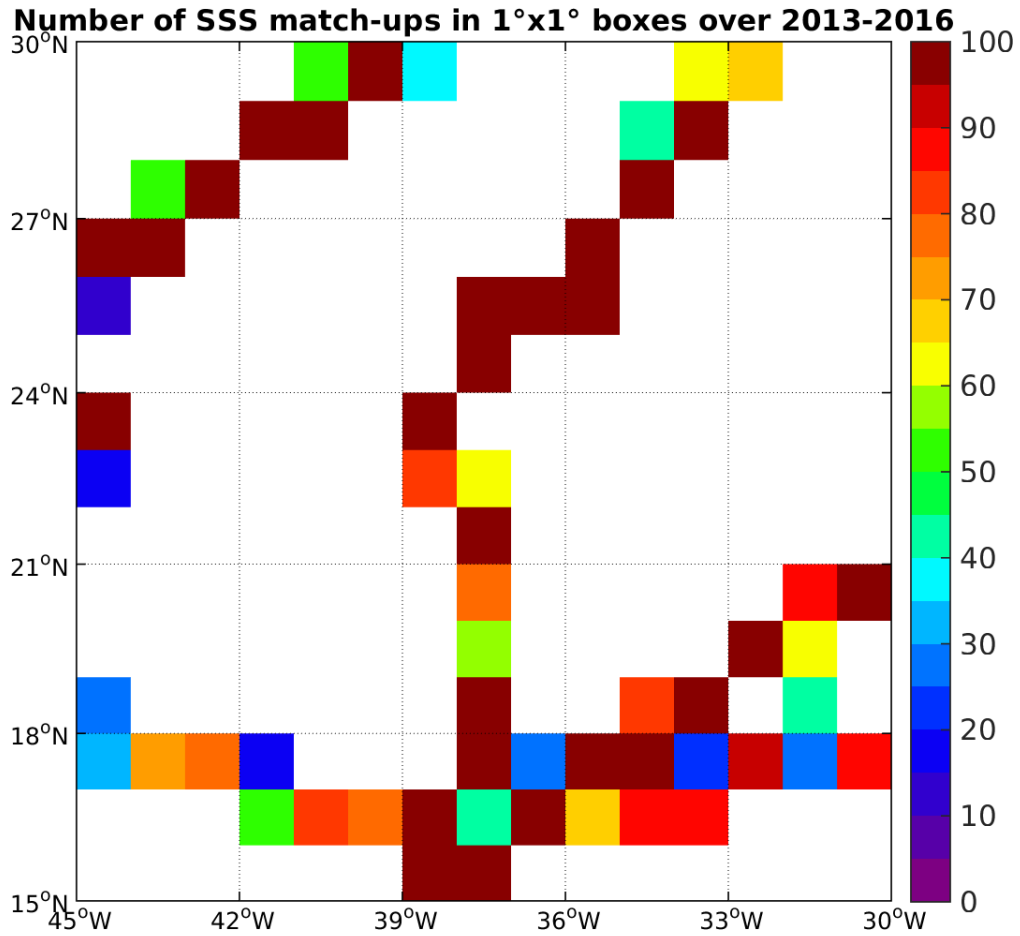
Figure 4: Number of SSS match-ups between TSG-GOSUD-Sailing-ship SSS and the SMOS-L3-CATDS-CECOS-LOCEAN-V2-9DAYS-25KM SSS product for the SPURS 1 Pi-MEP region over 1°x1° boxes and for the full satellite product period.
