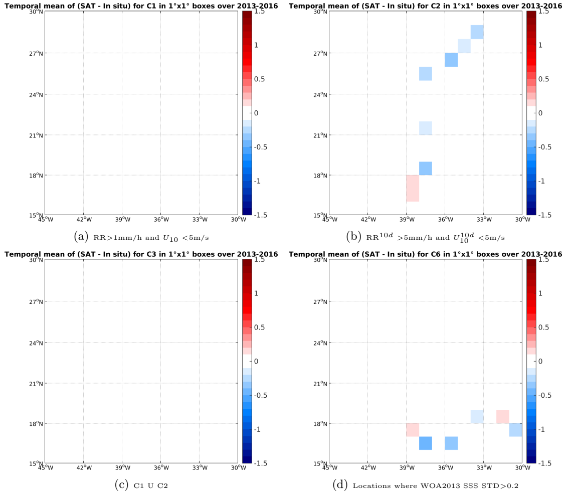
Figure 12: Temporal mean gridded over spatial boxes of size 1°x1° of \Delta SSS (SMOS-L3-CATDS-CECOS-LOCEAN-V2-9DAYS-25KM - TSG-GOSUD-Sailing-ship) for 4 different subdatasets corresponding to:RR>1mm/h and U_{10} < 5m/s (a), RR^{10d} > 5mm/h and U_{10}^{10d} < 5m/s (b), C1 U C2 (c),Locations where WOA2013 SSS STD>0.2 (d).
