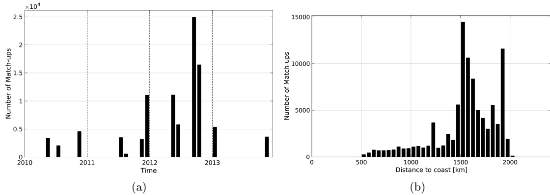
Figure 1: Number of match-ups between TSG-SAMOS and SMOS-L3-CATDS-CECOS-LOCEAN-V2-18DAYS-25KM SSS as a function of time (a) and as function of the distance to coast (b) over the SPURS 1 Pi-MEP region and for the full satellite product period.
