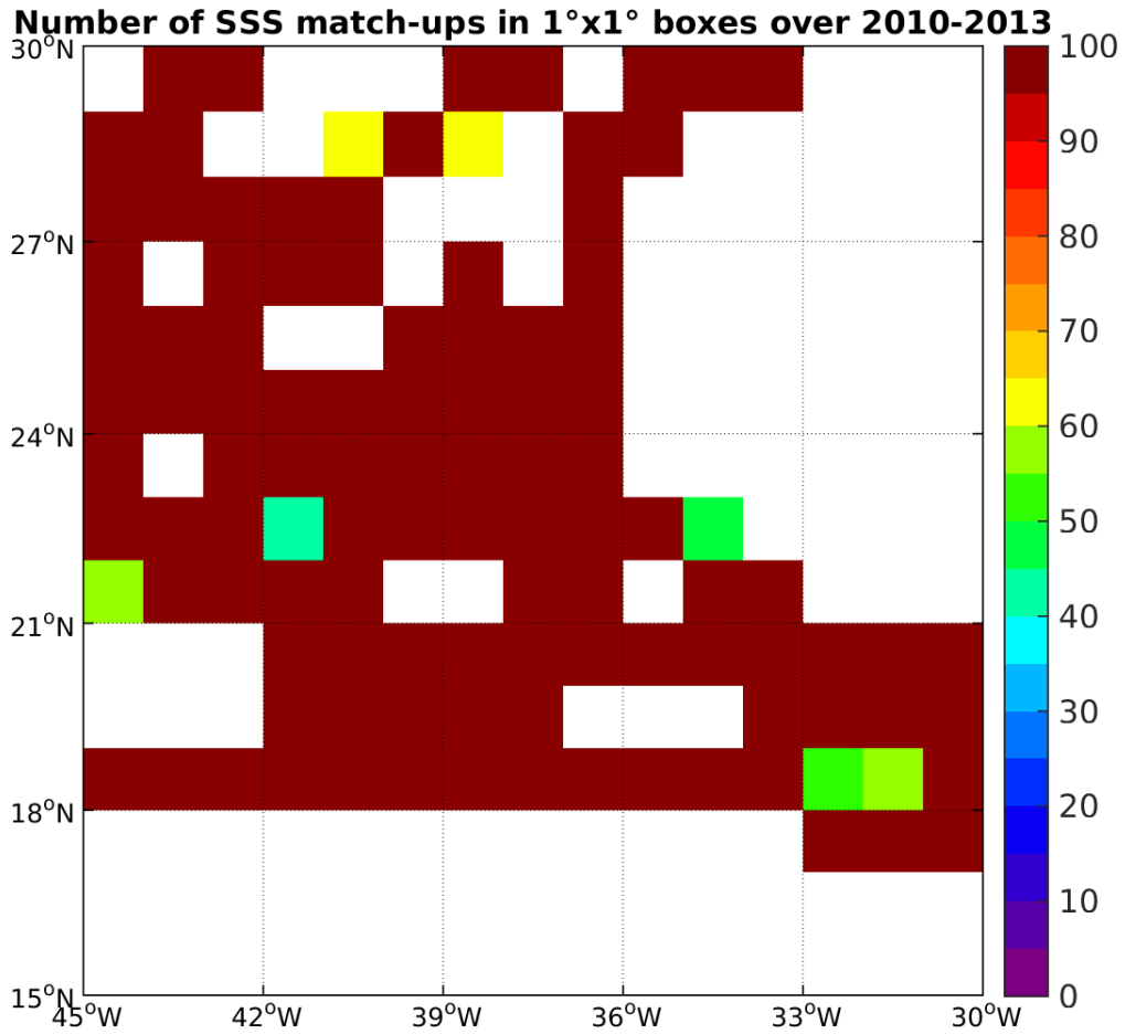
Figure 4: Number of SSS match-ups between TSG-SAMOS SSS and the SMOS-L3-CATDS-CECOS-LOCEAN-V2-18DAYS-25KM SSS product for the SPURS 1 Pi-MEP region over 1°x1° boxes and for the full satellite product period.
