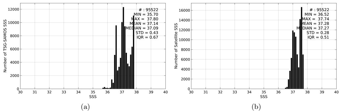
Figure 2: Histograms of SSS from TSG-SAMOS (a) and SMOS-L3-CATDS-CECOS-LOCEAN-V2-18DAYS-25KM (b) considering all match-up pairs per bins of 0.1 over the SPURS 1 Pi-MEP region and for the full satellite product period.
