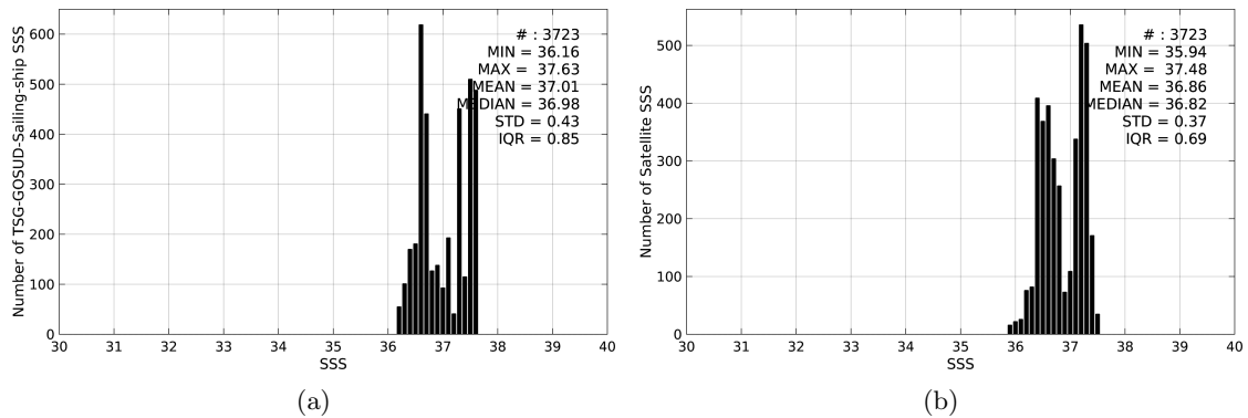
Figure 2: Histograms of SSS from TSG-GOSUD-Sailing-ship (a) and SMOS-L3-CATDS-CECOS-LOCEAN-V2-18DAYS-25KM (b) considering all match-up pairs per bins of 0.1 over the SPURS 1 Pi-MEP region and for the full satellite product period.
