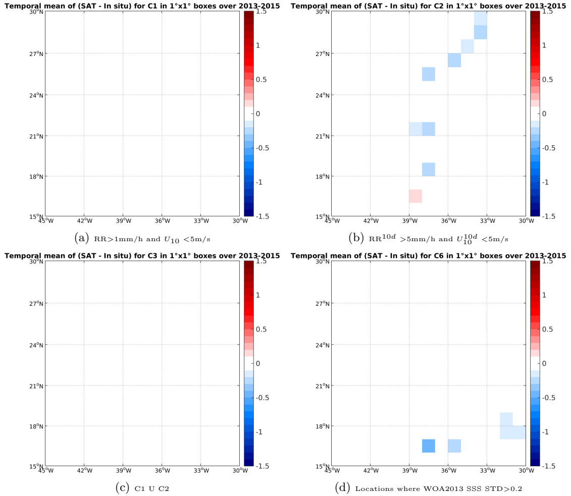
Figure 12: Temporal mean gridded over spatial boxes of size 1°x1° of \Delta SSS (SMOS-L3-CATDS-CECOS-LOCEAN-V2-18DAYS-25KM - TSG-GOSUD-Sailing-ship) for 4 different subdatasets corresponding to: RR > 1\text{mm/h} and U_{10} < 5\text{m/s} (a), RR^{10d} > 5\text{mm/h} and U_{10}^{10d} < 5\text{m/s} (b), C1 U C2 (c), Locations where WOA2013 SSS STD > 0.2 (d).
