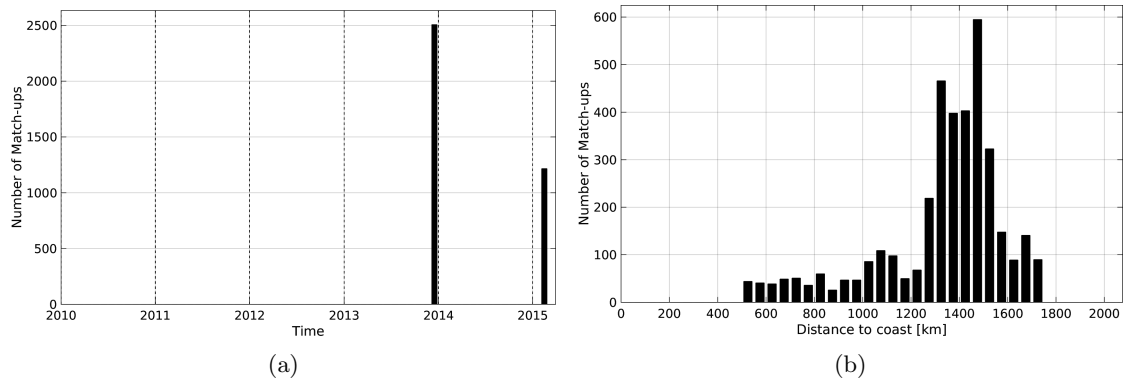
Figure 1: Number of match-ups between TSG-GOSUD-Sailing-ship and SMOS-L3-CATDS-CECOS-LOCEAN-V2-18DAYS-25KM SSS as a function of time (a) and as function of the distance to coast (b) over the SPURS 1 Pi-MEP region and for the full satellite product period.
