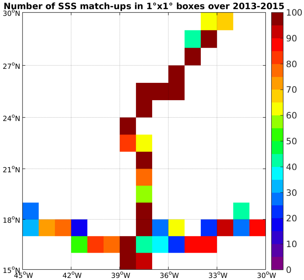
Figure 4: Number of SSS match-ups between TSG-GOSUD-Sailing-ship SSS and the SMOS-L3-CATDS-CECOS-LOCEAN-V2-18DAYS-25KM SSS product for the SPURS 1 Pi-MEP region over 1°x1° boxes and for the full satellite product period.
