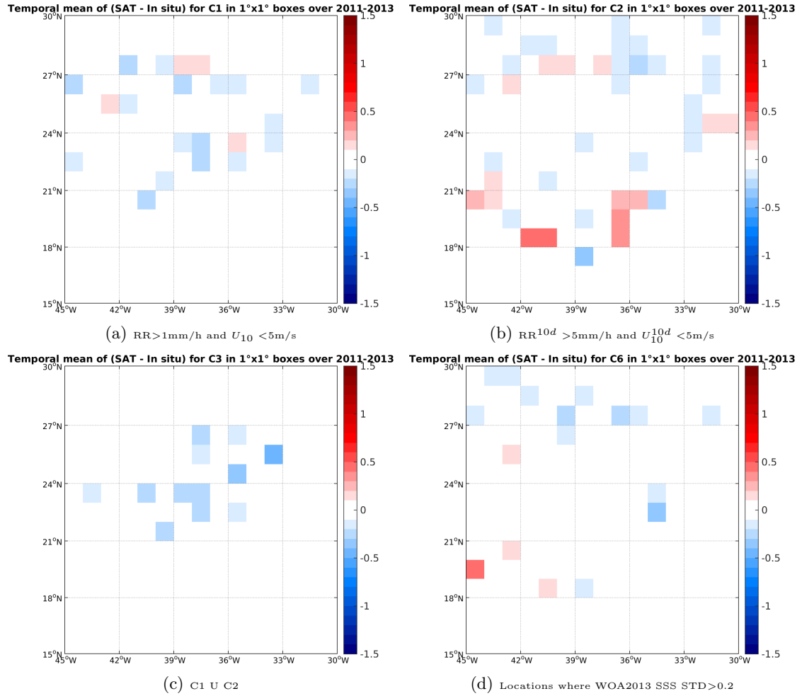
Figure 11: Temporal mean gridded over spatial boxes of size 1^\circ \times 1^\circ of \Delta SSS (SMOS-L3-CATDS-CECOS-LOCEAN-V2-18DAYS-25KM - Surface drifters) for 4 different subdatasets corresponding to: RR > 1\text{mm/h} and U_{10} < 5\text{m/s} (a), RR^{10d} > 5\text{mm/h} and U_{10}^{10d} < 5\text{m/s} (b), C1 U C2 (c), Locations where WOA2013 SSS STD > 0.2 (d).
