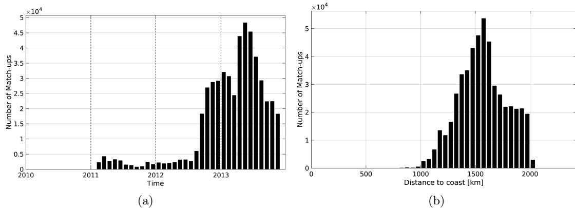
Figure 1: Number of match-ups between Surface drifters and SMOS-L3-CATDS-CECOS-LOCEAN-V2-18DAYS-25KM SSS as a function of time (a) and as function of the distance to coast (b) over the SPURS 1 Pi-MEP region and for the full satellite product period.
