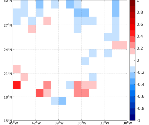
(e) MEAN( \Delta SSS) (Satellite - Surface drifters)
