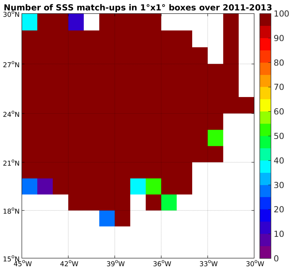
Figure 3: Number of SSS match-ups between Surface drifters SSS and the SMOS-L3-CATDS-CECOS-LOCEAN-V2-18DAYS-25KM SSS product for the SPURS 1 Pi-MEP region over 1°x1° boxes and for the full satellite product period.
