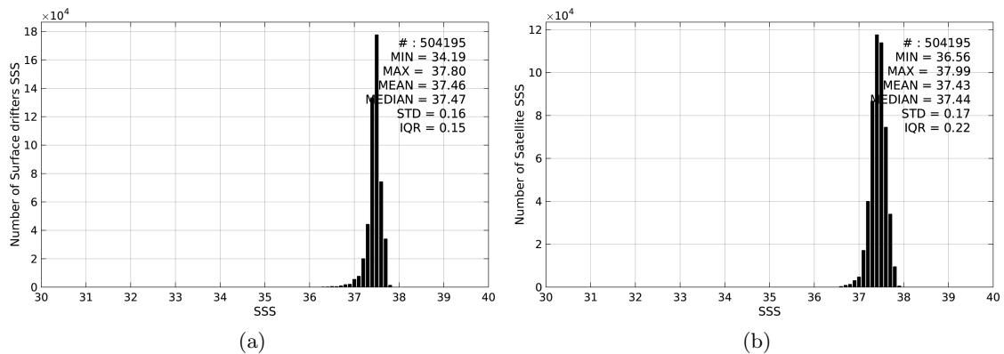
Figure 2: Histograms of SSS from Surface drifters (a) and SMOS-L3-CATDS-CECOS-LOCEAN-V2-18DAYS-25KM (b) considering all match-up pairs per bins of 0.1 over the SPURS 1 Pi-MEP region and for the full satellite product period.
