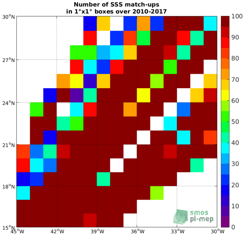
Figure 4: Number of SSS match-ups between TSG-LEGOS-DM SSS and the SMOS L3 v2 - Monthly - 0.25 Deg (CATDS-CECOS-IFREMER) SSS product for the SPURS 1 Pi-MEP region over 1°x1° boxes and for the full satellite product period.
