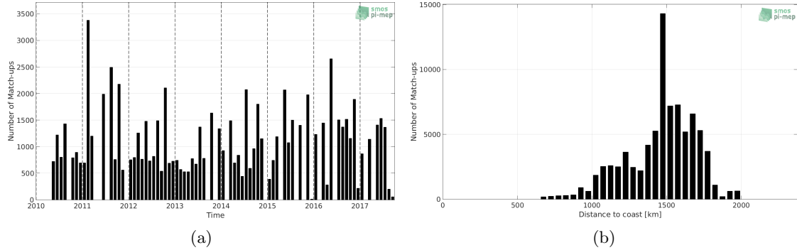
Figure 1: Number of match-ups between TSG-LEGOS-DM and SMOS L3 v2 - Monthly - 0.25 Deg (CATDS-CECOS-IFREMER) SSS as a function of time (a) and as function of the distance to coast (b) over the SPURS 1 Pi-MEP region and for the full satellite product period.
