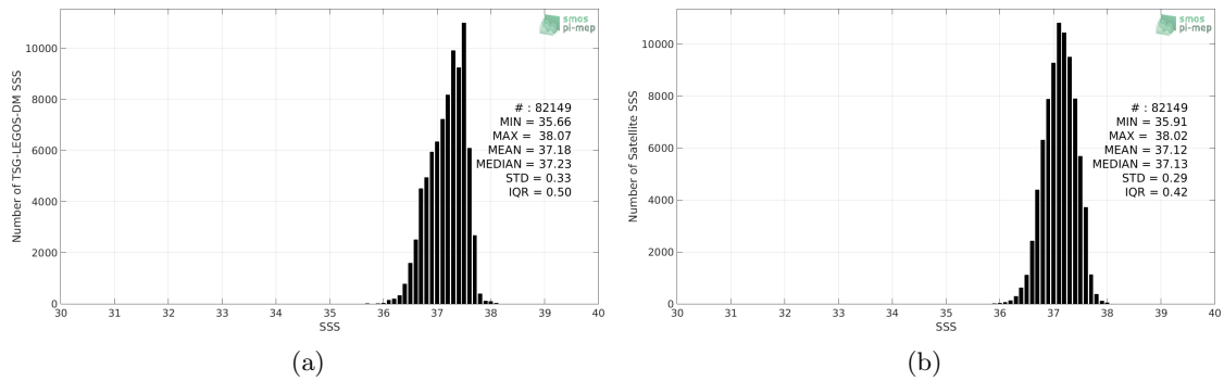
Figure 2: Histograms of SSS from TSG-LEGOS-DM (a) and SMOS L3 v2 - Monthly - 0.25 Deg (CATDS-CECOS-IFREMER) (b) considering all match-up pairs per bins of 0.1 over the SPURS 1 Pi-MEP region and for the full satellite product period.
