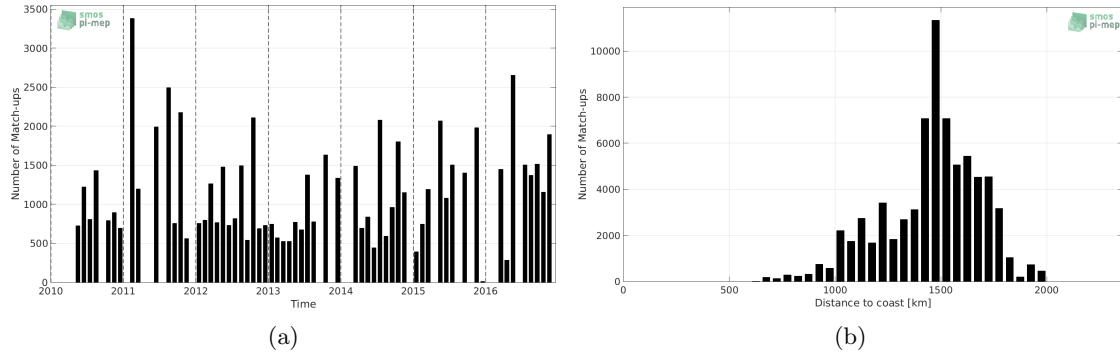
Figure 1: Number of match-ups between TSG-LEGOS-DM and SMOS-L3-CATDS-IFREMER-CECOS-V2-MONTHLY-0.25DEG SSS as a function of time (a) and as function of the distance to coast (b) over the SPURS 1 Pi-MEP region and for the full satellite product period.
