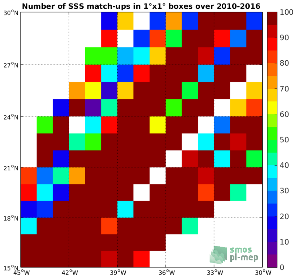
Figure 4: Number of SSS match-ups between TSG-LEGOS-DM SSS and the SMOS-L3-CATDS-IFREMER-CECOS-V2-MONTHLY-0.25DEG SSS product for the SPURS 1 Pi-MEP region over 1°x1° boxes and for the full satellite product period.
