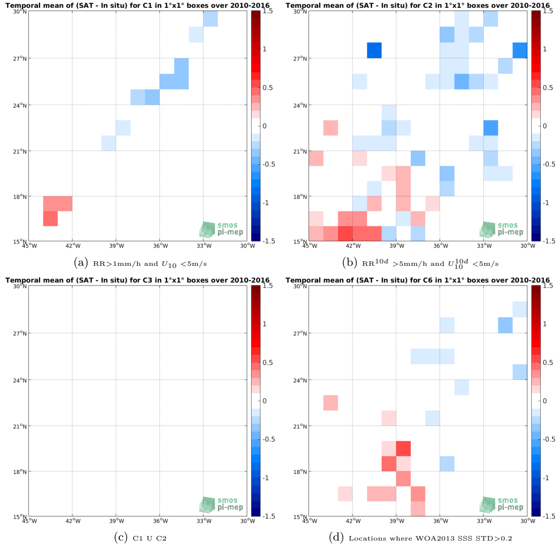
Figure 12: Temporal mean gridded over spatial boxes of size 1^\circ \times 1^\circ of \Delta SSS (SMOS-L3-CATDS-IFREMER-CECOS-V2-MONTHLY-0.25DEG - TSG-LEGOS-DM) for 4 different subdatasets corresponding to: RR > 1\text{mm/h} and U_{10} < 5\text{m/s} (a), RR^{10d} > 5\text{mm/h} and U_{10}^{10d} < 5\text{m/s} (b), C1 U C2 (c), Locations where WOA2013 SSS STD > 0.2 (d).
