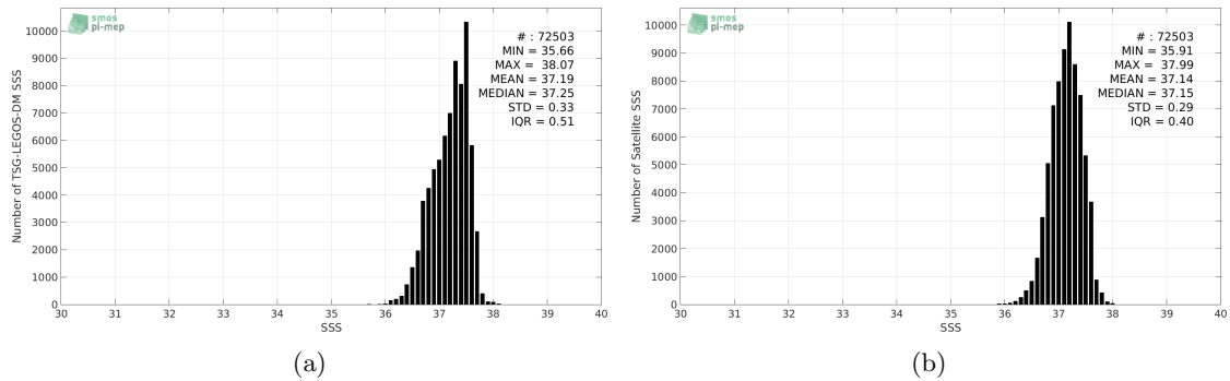
Figure 2: Histograms of SSS from TSG-LEGOS-DM (a) and SMOS-L3-CATDS-IFREMER-CECOS-V2-MONTHLY-0.25DEG (b) considering all match-up pairs per bins of 0.1 over the SPURS 1 Pi-MEP region and for the full satellite product period.
