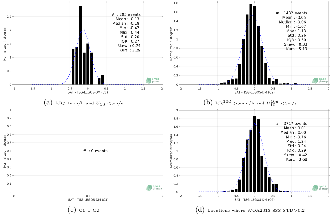
Figure 13: Normalized histogram of \Delta\text{SSS} (SMOS-L3-CATDS-IFREMER-CECOS-V2-MONTHLY-0.25DEG - TSG-LEGOS-DM) for 6 different subdatasets corresponding to: RR > 1mm/h and U_{10} < 5\text{m/s} (a), RR^{10d} > 5\text{mm/h} and U_{10}^{10d} < 5\text{m/s} (b), C1 U C2 (c), Locations where WOA2013 SSS STD > 0.2 (d).
