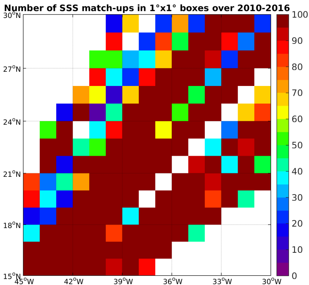
Figure 4: Number of SSS match-ups between TSG-LEGOS-DM SSS and the SMOS-L3-CATDS-IFREMER-CECOS-V2-MONTHLY-0.25DEG SSS product for the SPURS 1 Pi-MEP region over 1°x1° boxes and for the full satellite product period.
