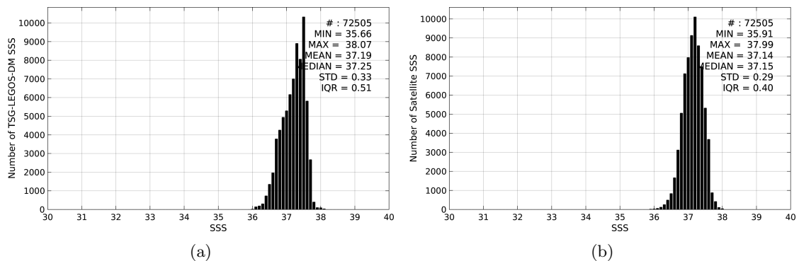
Figure 2: Histograms of SSS from TSG-LEGOS-DM (a) and SMOS-L3-CATDS-IFREMER-CECOS-V2-MONTHLY-0.25DEG (b) considering all match-up pairs per bins of 0.1 over the SPURS 1 Pi-MEP region and for the full satellite product period.
