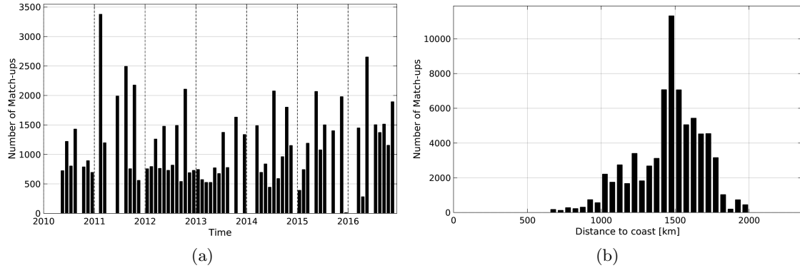
Figure 1: Number of match-ups between TSG-LEGOS-DM and SMOS-L3-CATDS-IFREMER-CECOS-V2-MONTHLY-0.25DEG SSS as a function of time (a) and as function of the distance to coast (b) over the SPURS 1 Pi-MEP region and for the full satellite product period.
