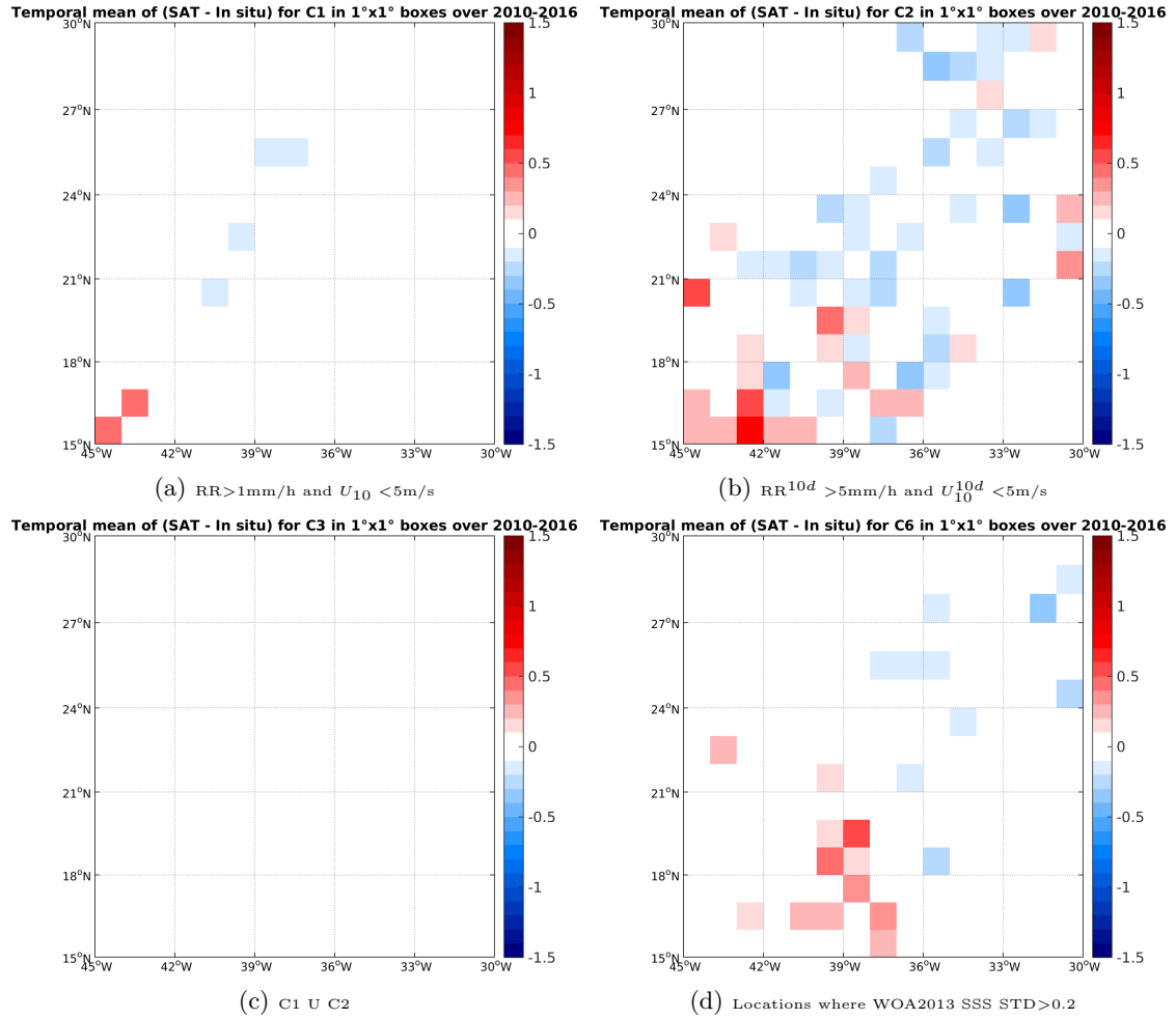
Figure 12: Temporal mean gridded over spatial boxes of size 1^\circ \times 1^\circ of \Delta SSS (SMOS-L3-CATDS-IFREMER-CECOS-V2-MONTHLY-0.25DEG - TSG-LEGOS-DM) for 4 different subdatasets corresponding to: RR > 1mm/h and U_{10} < 5 m/s (a), RR^{10d} > 5 mm/h and U_{10}^{10d} < 5 m/s (b), C1 U C2 (c), Locations where WOA2013 SSS STD > 0.2 (d).
