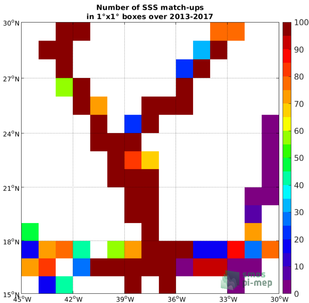
Figure 4: Number of SSS match-ups between TSG (GOSUD-Sailing-ship) SSS and the SMOS SSS L3 v2 - Monthly - 0.25 Deg (CATDS-CECOS-IFREMER) SSS product for the SPURS 1 Pi-MEP region over 1°x1° boxes and for the full satellite product period.
