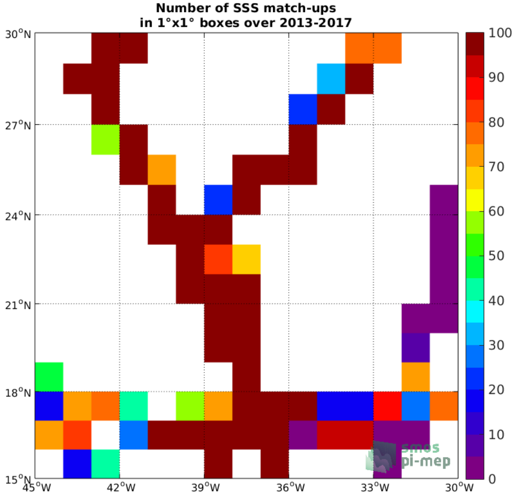
Figure 4: Number of SSS match-ups between TSG (GOSUD-Sailing-ship) SSS and the SMOS SSS L3 v2 - Monthly - 0.25 Deg (CATDS-CECOS-IFREMER) SSS product for the SPURS 1 Pi-MEP region over 1°x1° boxes and for the full satellite product period.
