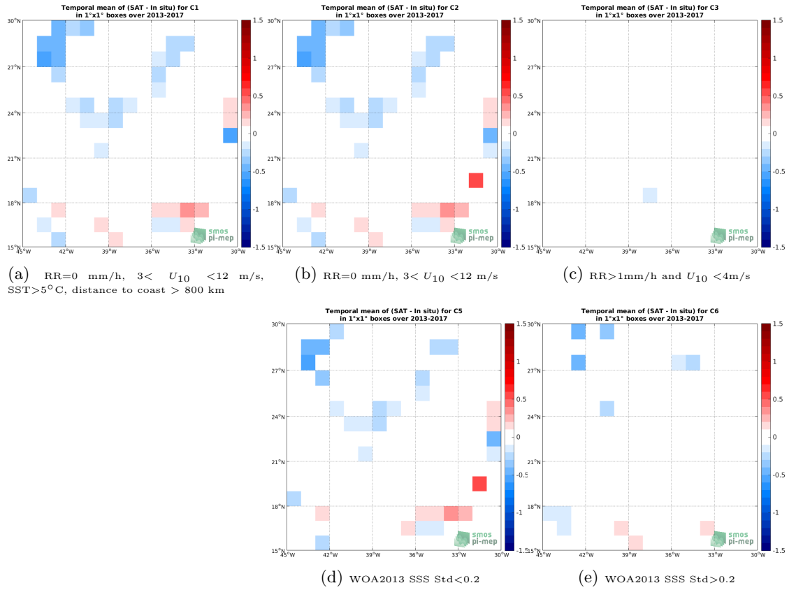
Figure 12: Temporal mean gridded over spatial boxes of size 1^{\circ} \times 1^{\circ} of \Delta SSS (SMOS SSS L3 v2 - Monthly - 0.25 Deg (CATDS-CECOS-IFREMER) - TSG (GOSUD-Sailing-ship)) for 5 different subdatasets corresponding to:RR=0 mm/h, 3 < U_{10} < 12 m/s, SST>5°C, distance to coast > 800 km (a), RR=0 mm/h, 3 < U_{10} < 12 m/s (b), RR>1mm/h and U_{10} < 4 m/s (c), WOA2013 SSS Std<0.2 (d), WOA2013 SSS Std>0.2 (e).
