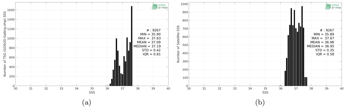
Figure 2: Histograms of SSS from TSG (GOSUD-Sailing-ship) (a) and SMOS SSS L3 v2 - Monthly - 0.25 Deg (CATDS-CECOS-IFREMER) (b) considering all match-up pairs per bins of 0.1 over the SPURS 1 Pi-MEP region and for the full satellite product period.
