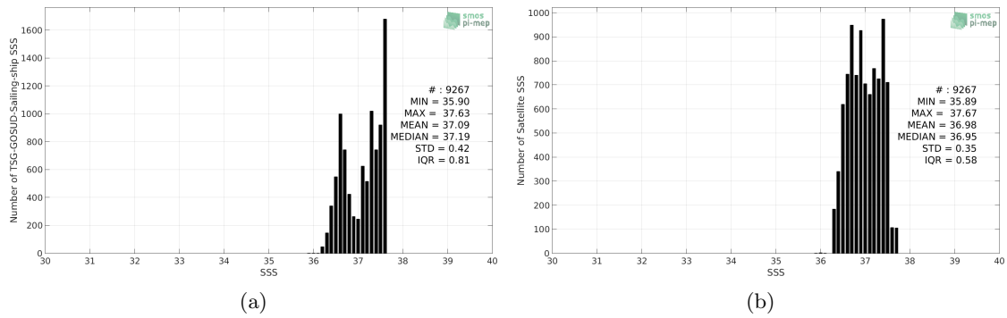
Figure 2: Histograms of SSS from TSG-GOSUD-Sailing-ship (a) and SMOS L3 v2 - Monthly - 0.25 Deg (CATDS-CECOS-IFREMER) (b) considering all match-up pairs per bins of 0.1 over the SPURS 1 Pi-MEP region and for the full satellite product period.
