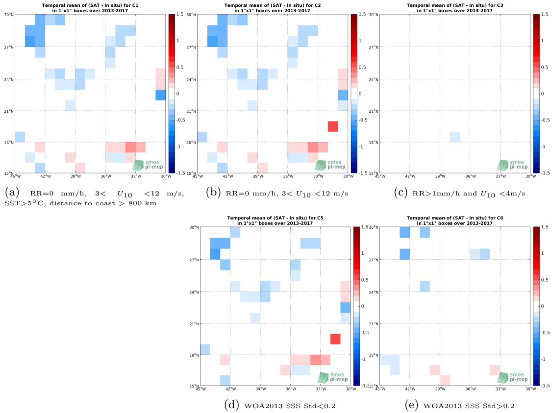
Figure 12: Temporal mean gridded over spatial boxes of size 1^\circ \times 1^\circ of \Delta SSS (SMOS L3 v2 - Monthly - 0.25 Deg (CATDS-CECOS-IFREMER) - TSG-GOSUD-Sailing-ship) for 5 different subdatasets corresponding to:RR=0 mm/h, 3 < U_{10} < 12 m/s, SST>5°C, distance to coast > 800 km (a), RR=0 mm/h, 3 < U_{10} < 12 m/s (b), RR>1mm/h and U_{10} < 4 m/s (c), WOA2013 SSS Std<0.2 (d), WOA2013 SSS Std>0.2 (e).
