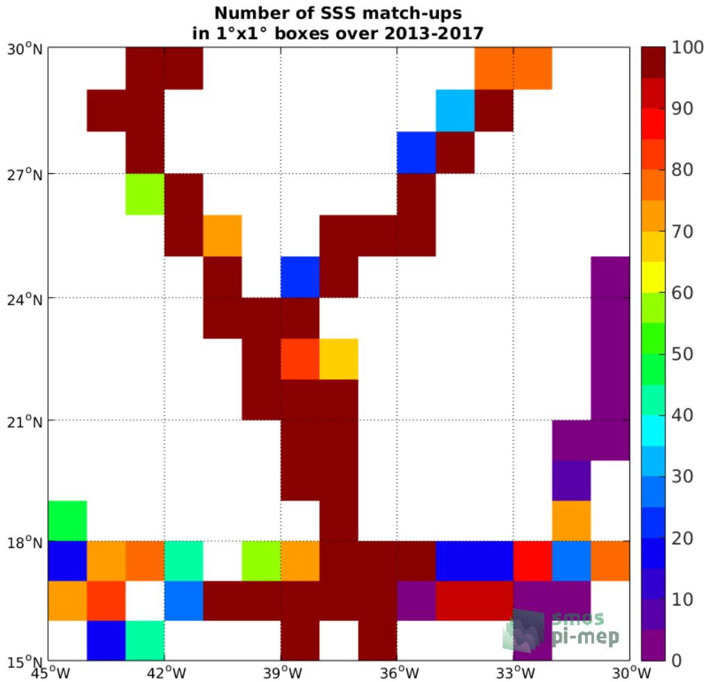
Figure 4: Number of SSS match-ups between TSG-GOSUD-Sailing-ship SSS and the SMOS L3 v2 - Monthly - 0.25 Deg (CATDS-CECOS-IFREMER) SSS product for the SPURS 1 Pi-MEP region over 1°x1° boxes and for the full satellite product period.
