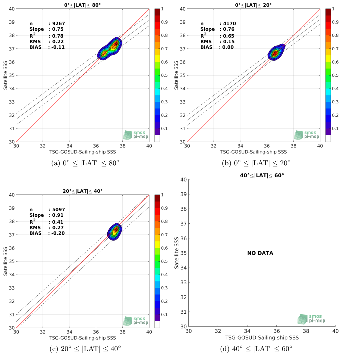
Figure 9: Contour maps of the concentration of SMOS L3 v2 - Monthly - 0.25 Deg (CATDS-CECOS-IFREMER) SSS (y-axis) versus TSG-GOSUD-Sailing-ship SSS (x-axis) at match-up pairs for different latitude bands. For each plot, the red line shows x=y . The black thin and dashed lines indicate a linear fit through the data cloud and the \pm 95\% confidence levels, respectively. The number match-up pairs n , the slope and R^2 coefficient of the linear fit, the root mean square (RMS) and the mean bias between satellite and in situ data are indicated for each latitude band in each plots.
