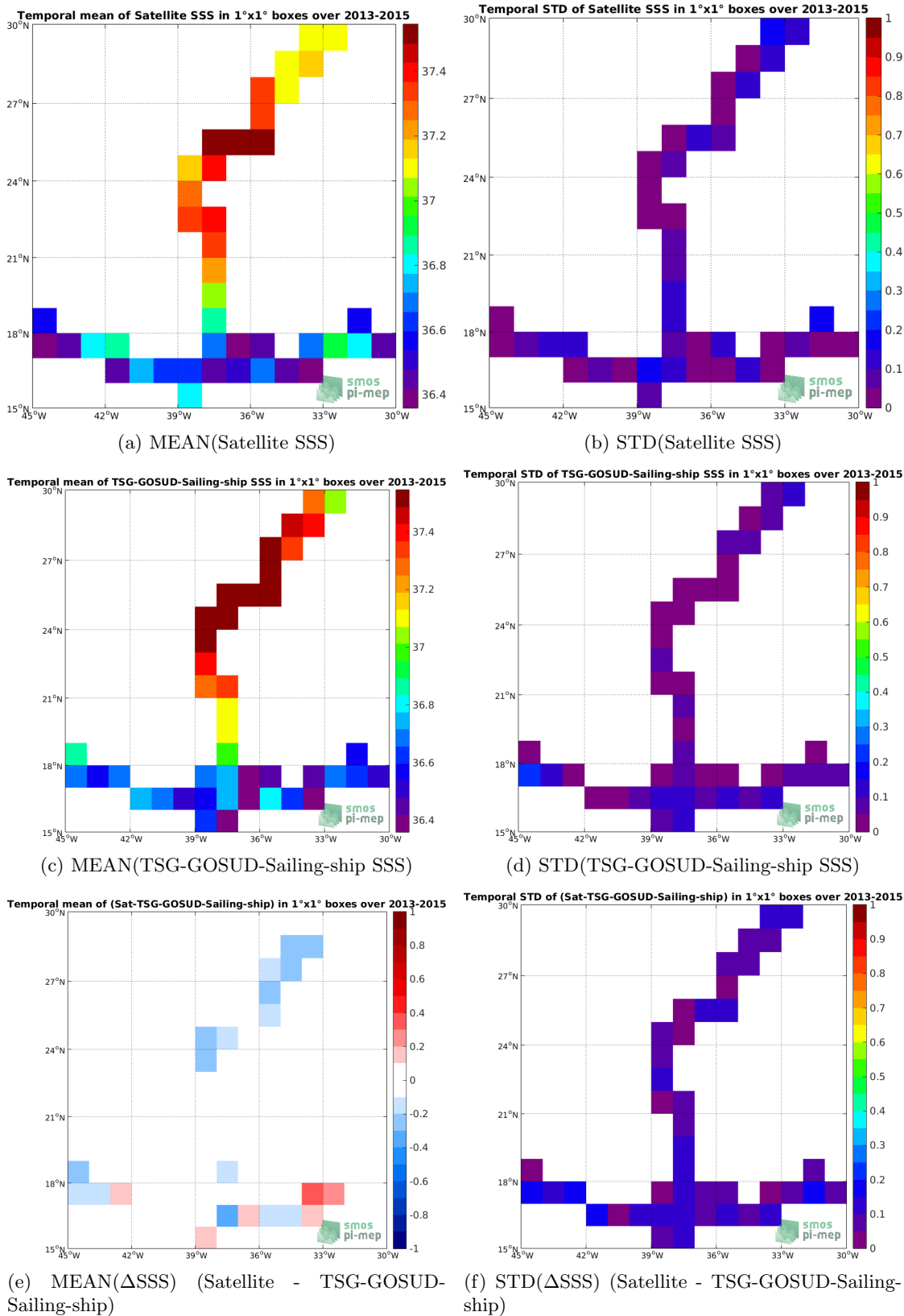
Figure 6: Temporal mean (left) and STD (right) of SSS from SMOS-L3-CATDS-IFREMER-CECOS-V2-MONTHLY-0.25DEG (top), TSG-GOSUD-Sailing-ship (middle), and of \Delta SSS (Satellite - TSG-GOSUD-Sailing-ship). Only match-up pairs are used to generate these maps.
