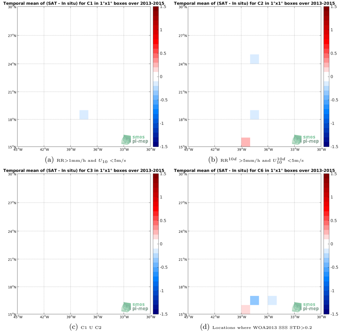
Figure 12: Temporal mean gridded over spatial boxes of size 1^\circ \times 1^\circ of \Delta SSS (SMOS-L3-CATDS-IFREMER-CECOS-V2-MONTHLY-0.25DEG - TSG-GOSUD-Sailing-ship) for 4 different sub-datasets corresponding to: RR > 1mm/h and U_{10} < 5\text{m/s} (a), RR 10d > 5mm/h and U_{10}^{10d} < 5\text{m/s} (b), C1 U C2 (c), Locations where WOA2013 SSS STD > 0.2 (d).
