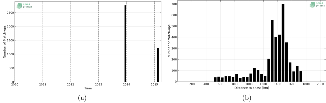
Figure 1: Number of match-ups between TSG-GOSUD-Sailing-ship and SMOS-L3-CATDS-IFREMER-CECOS-V2-MONTHLY-0.25DEG SSS as a function of time (a) and as function of the distance to coast (b) over the SPURS 1 Pi-MEP region and for the full satellite product period.
