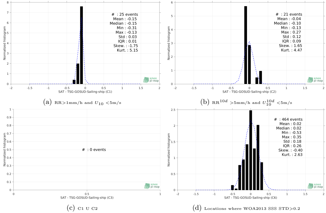
Figure 13: Normalized histogram of \Delta\text{SSS} (SMOS-L3-CATDS-IFREMER-CECOS-V2-MONTHLY-0.25DEG - TSG-GOSUD-Sailing-ship) for 6 different subdatasets corresponding to: RR > 1\text{mm/h} and U_{10} < 5\text{m/s} (a), RR^{10d} > 5\text{mm/h} and U_{10}^{10d} < 5\text{m/s} (b), C1 U C2 (c), Locations where WOA2013 SSS STD > 0.2 (d).
