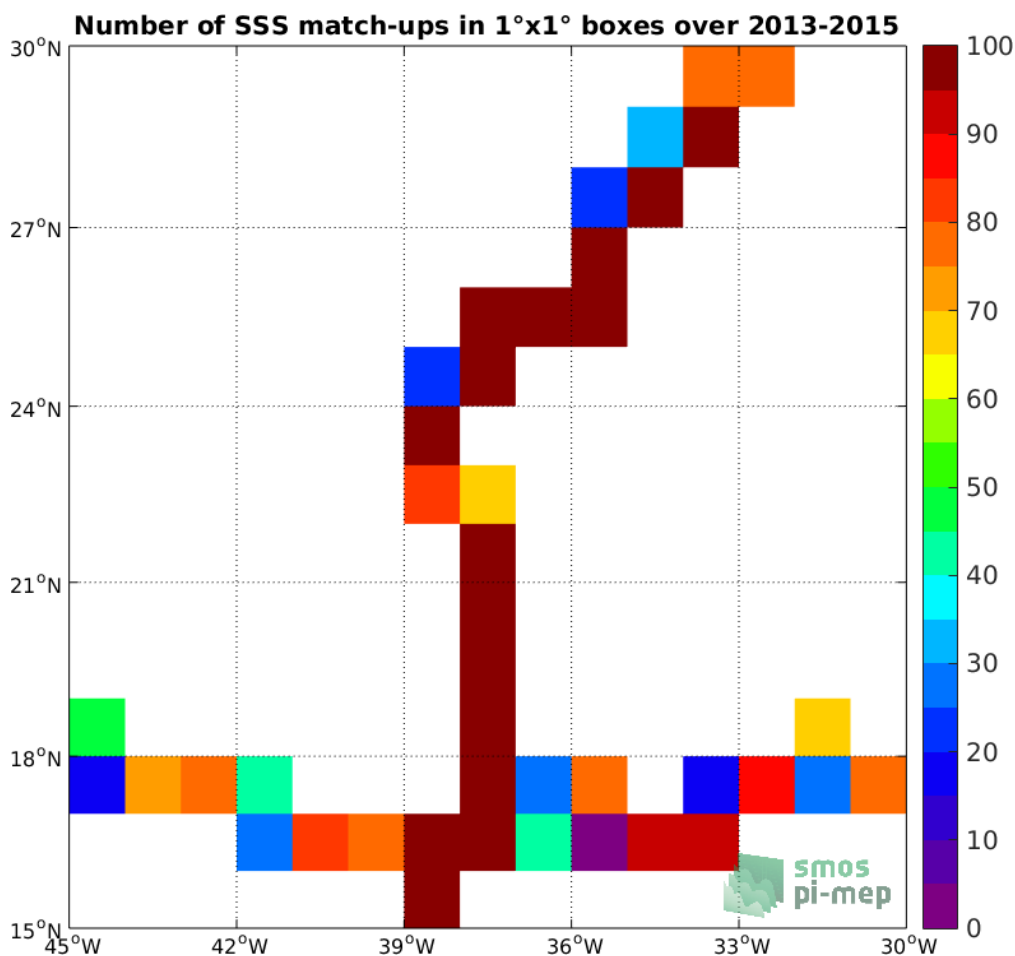
Figure 4: Number of SSS match-ups between TSG-GOSUD-Sailing-ship SSS and the SMOS-L3-CATDS-IFREMER-CECOS-V2-MONTHLY-0.25DEG SSS product for the SPURS 1 Pi-MEP region over 1°x1° boxes and for the full satellite product period.
