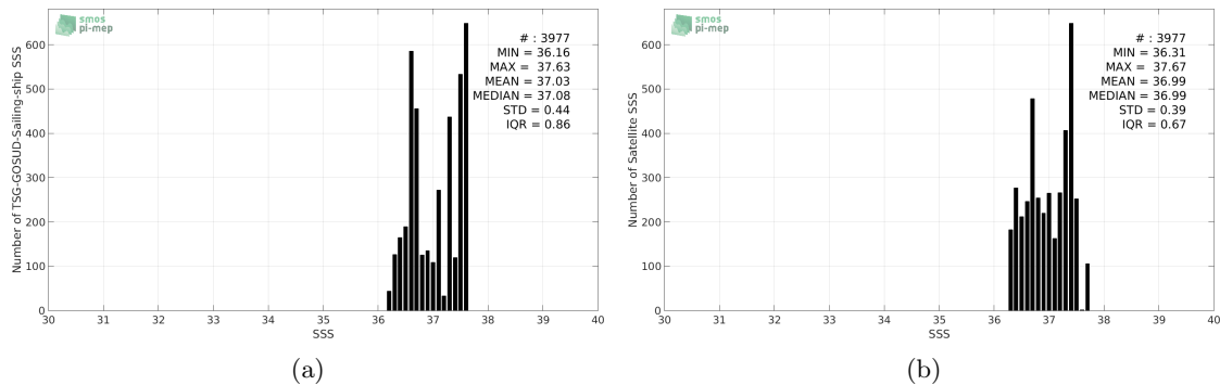
Figure 2: Histograms of SSS from TSG-GOSUD-Sailing-ship (a) and SMOS-L3-CATDS-IFREMER-CECOS-V2-MONTHLY-0.25DEG (b) considering all match-up pairs per bins of 0.1 over the SPURS 1 Pi-MEP region and for the full satellite product period.
