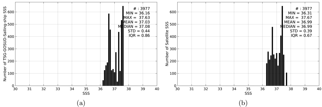
Figure 2: Histograms of SSS from TSG-GOSUD-Sailing-ship (a) and SMOS-L3-CATDS-IFREMER-CECOS-V2-MONTHLY-0.25DEG (b) considering all match-up pairs per bins of 0.1 over the SPURS 1 Pi-MEP region and for the full satellite product period.
