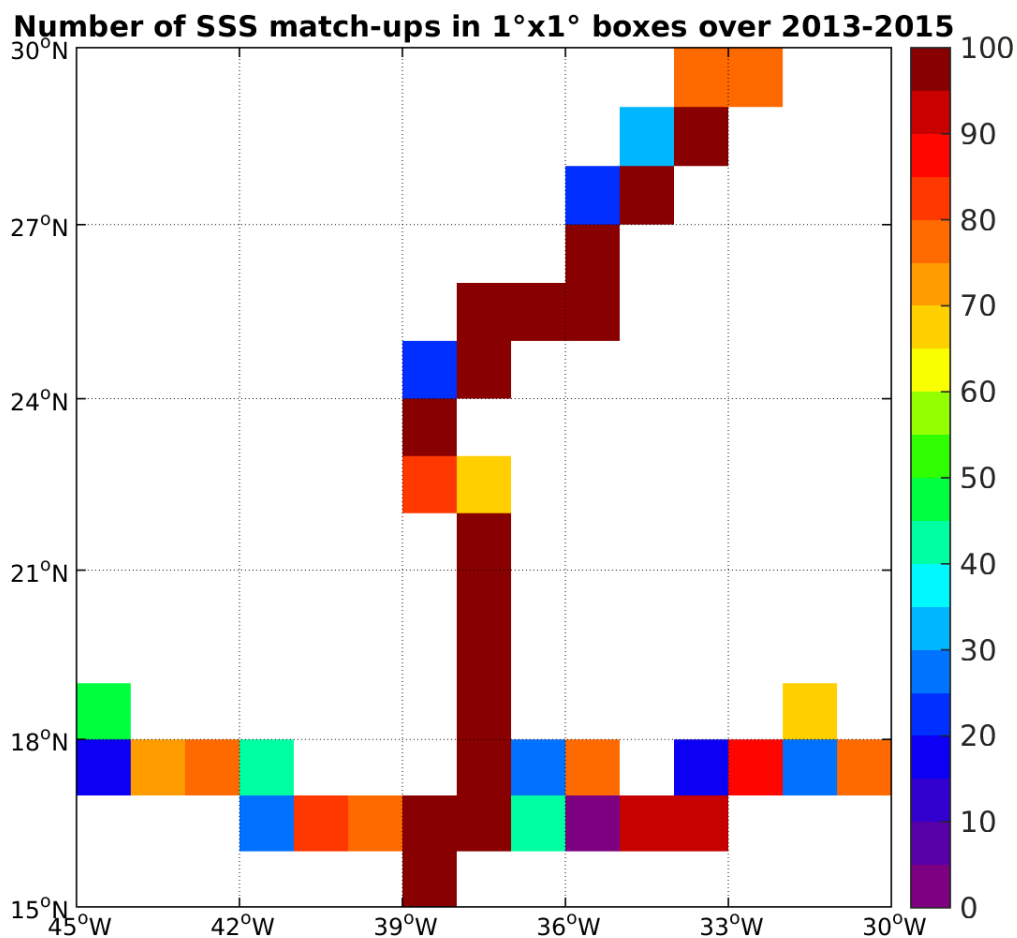
Figure 4: Number of SSS match-ups between TSG-GOSUD-Sailing-ship SSS and the SMOS-L3-CATDS-IFREMER-CECOS-V2-MONTHLY-0.25DEG SSS product for the SPURS 1 Pi-MEP region over 1°x1° boxes and for the full satellite product period.
