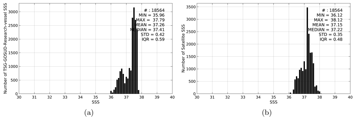
Figure 2: Histograms of SSS from TSG-GOSUD-Research-vessel (a) and SMOS-L3-CATDS-IFREMER-CECOS-V2-MONTHLY-0.25DEG (b) considering all match-up pairs per bins of 0.1 over the SPURS 1 Pi-MEP region and for the full satellite product period.
