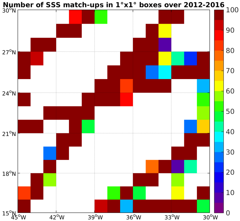
Figure 4: Number of SSS match-ups between TSG-GOSUD-Research-vessel SSS and the SMOS-L3-CATDS-IFREMER-CECOS-V2-MONTHLY-0.25DEG SSS product for the SPURS 1 Pi-MEP region over 1°x1° boxes and for the full satellite product period.
