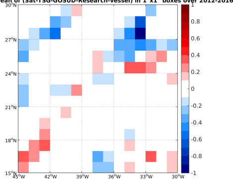
(e) MEAN( \Delta SSS) (Satellite - TSG-GOSUD-Research-vessel)
