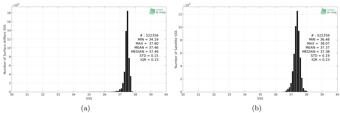
Figure 2: Histograms of SSS from Surface drifters (a) and SMOS L3 v2 - Monthly - 0.25 Deg (CATDS-CECOS-IFREMER) (b) considering all match-up pairs per bins of 0.1 over the SPURS 1 Pi-MEP region and for the full satellite product period.
