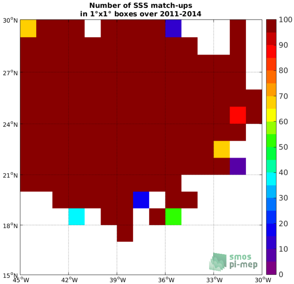
Figure 3: Number of SSS match-ups between Surface drifters SSS and the SMOS L3 v2 - Monthly - 0.25 Deg (CATDS-CECOS-IFREMER) SSS product for the SPURS 1 Pi-MEP region over 1°x1° boxes and for the full satellite product period.
