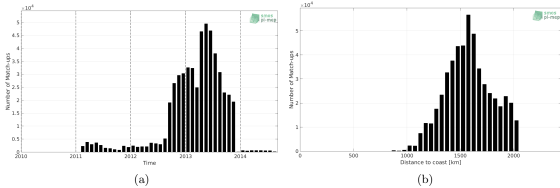
Figure 1: Number of match-ups between Surface drifters and SMOS L3 v2 - Monthly - 0.25 Deg (CATDS-CECOS-IFREMER) SSS as a function of time (a) and as function of the distance to coast (b) over the SPURS 1 Pi-MEP region and for the full satellite product period.
