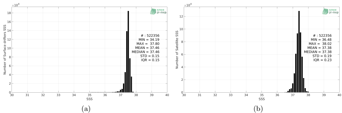
Figure 2: Histograms of SSS from Surface drifters (a) and SMOS-L3-CATDS-IFREMER-CECOS-V2-MONTHLY-0.25DEG (b) considering all match-up pairs per bins of 0.1 over the SPURS 1 Pi-MEP region and for the full satellite product period.
