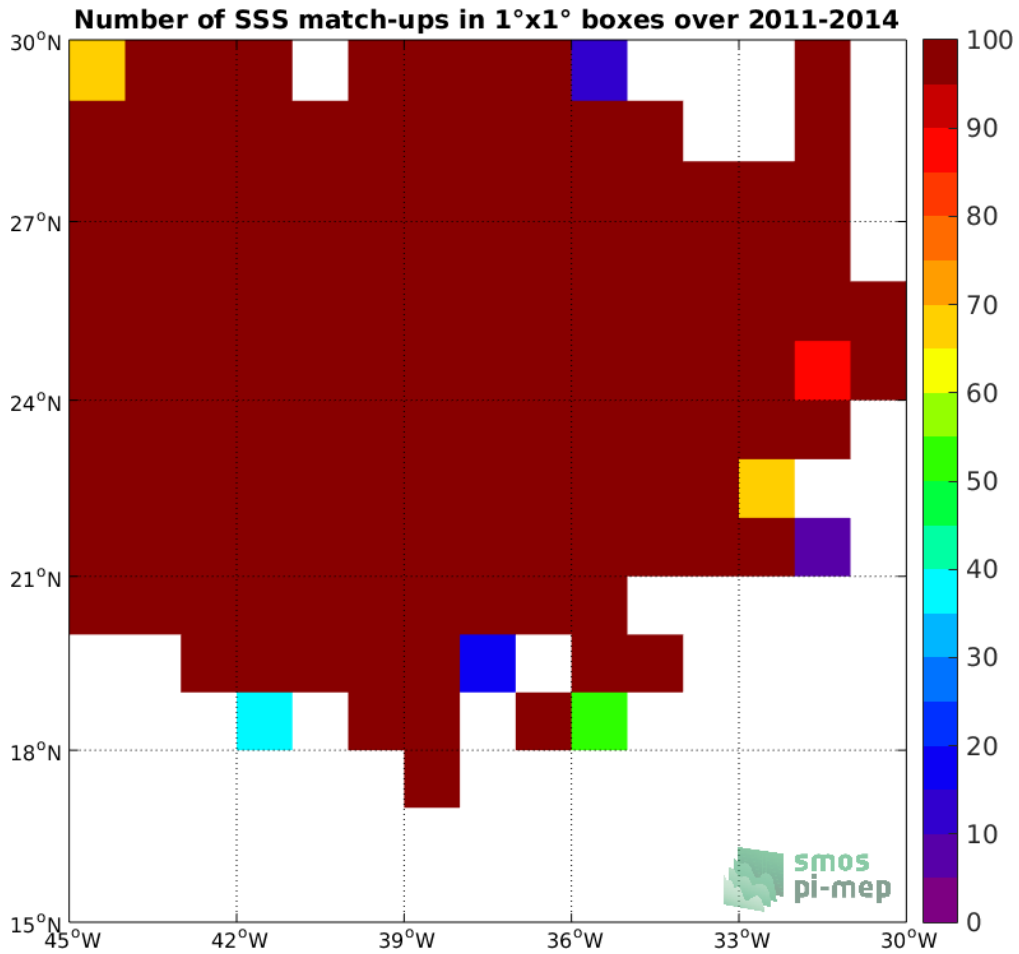
Figure 3: Number of SSS match-ups between Surface drifters SSS and the SMOS-L3-CATDS-IFREMER-CECOS-V2-MONTHLY-0.25DEG SSS product for the SPURS 1 Pi-MEP region over 1°x1° boxes and for the full satellite product period.
