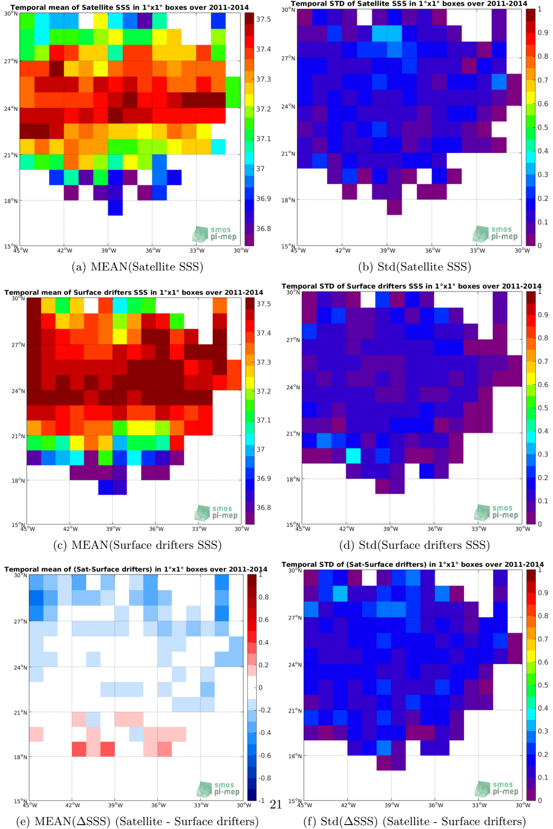
Figure 5: Temporal mean (left) and Std (right) of SSS from SMOS-L3-CATDS-IFREMER-CECOS-V2-MONTHLY-0.25DEG (top), Surface drifters (middle), and of \Delta SSS (Satellite - Surface drifters). Only match-up pairs are used to generate these maps.
