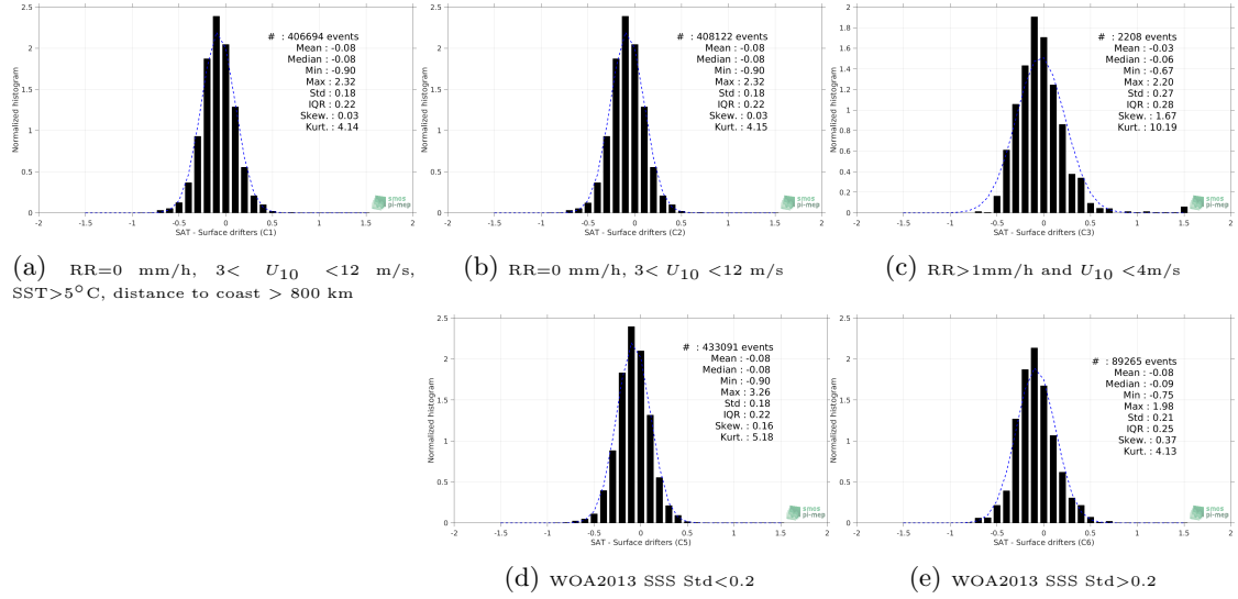
Figure 12: Normalized histogram of \Delta\text{SSS} (SMOS-L3-CATDS-IFREMER-CECOS-V2-MONTHLY-0.25DEG - Surface drifters) for 5 different subdatasets corresponding to: RR=0 mm/h, 3 < U_{10} < 12 m/s, SST>5°C, distance to coast > 800 km (a), RR=0 mm/h, 3 < U_{10} < 12 m/s (b), RR>1mm/h and U_{10} < 4 m/s (c), WOA2013 SSS Std<0.2 (d), WOA2013 SSS Std>0.2 (e).
