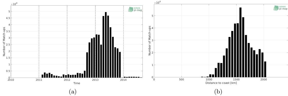
Figure 1: Number of match-ups between Surface drifters and SMOS-L3-CATDS-IFREMER-CECOS-V2-MONTHLY-0.25DEG SSS as a function of time (a) and as function of the distance to coast (b) over the SPURS 1 Pi-MEP region and for the full satellite product period.
