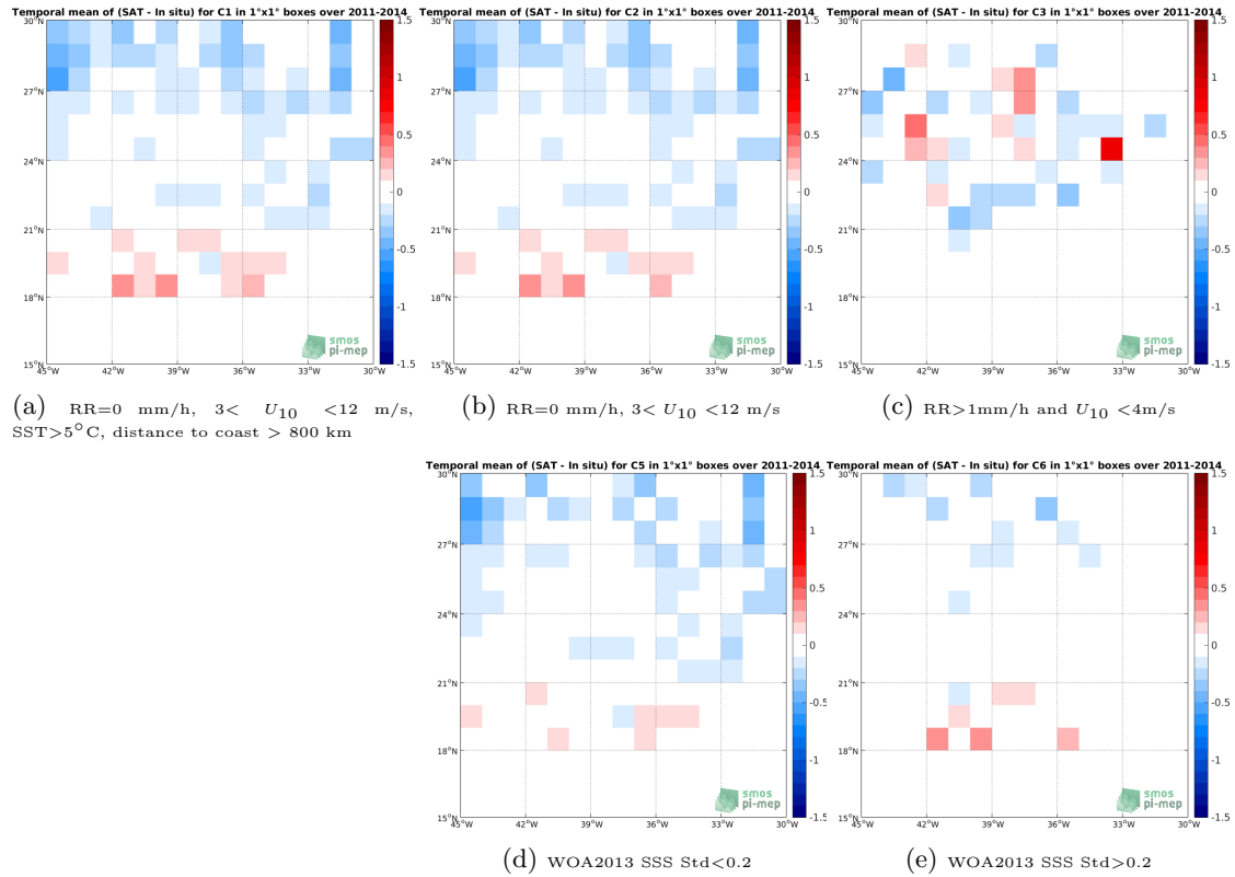
Figure 11: Temporal mean gridded over spatial boxes of size 1^\circ \times 1^\circ of \Delta SSS (SMOS-L3-CATDS-IFREMER-CECOS-V2-MONTHLY-0.25DEG - Surface drifters) for 5 different subdatasets corresponding to:RR=0 mm/h, 3 < U_{10} < 12 m/s, SST > 5^\circ\text{C} , distance to coast > 800 km (a), RR=0 mm/h, 3 < U_{10} < 12 m/s (b), RR > 1 mm/h and U_{10} < 4 m/s (c), WOA2013 SSS Std < 0.2 (d), WOA2013 SSS Std > 0.2 (e).
