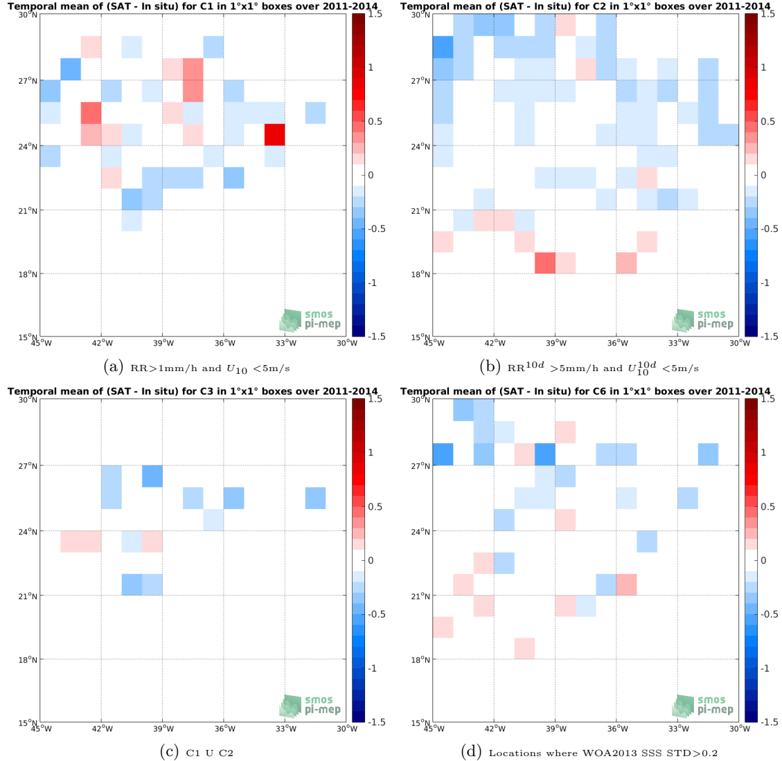
Figure 11: Temporal mean gridded over spatial boxes of size 1^\circ \times 1^\circ of \Delta SSS (SMOS-L3-CATDS-IFREMER-CECOS-V2-MONTHLY-0.25DEG - Surface drifters) for 4 different subdatasets corresponding to: RR > 1\text{mm/h} and U_{10} < 5\text{m/s} (a), RR^{10d} > 5\text{mm/h} and U_{10}^{10d} < 5\text{m/s} (b), C1 U C2 (c), Locations where WOA2013 SSS STD > 0.2 (d).
