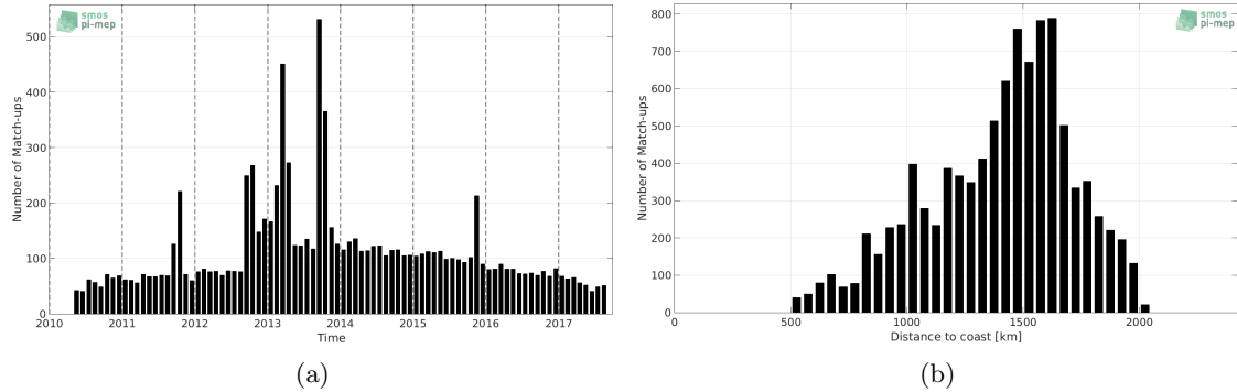
Figure 1: Number of match-ups between Argo and SMOS-L3-CATDS-IFREMER-CECOS-V2-MONTHLY-0.25DEG SSS as a function of time (a) and as function of the distance to coast (b) over the SPURS 1 Pi-MEP region and for the full satellite product period.
