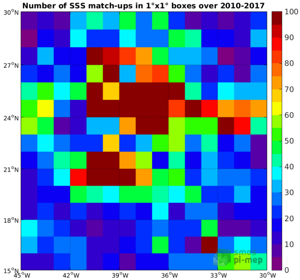
Figure 4: Number of SSS match-ups between Argo SSS and the SMOS-L3-CATDS-IFREMER-CECOS-V2-MONTHLY-0.25DEG SSS product for the SPURS 1 Pi-MEP region over 1°x1° boxes and for the full satellite product period.
