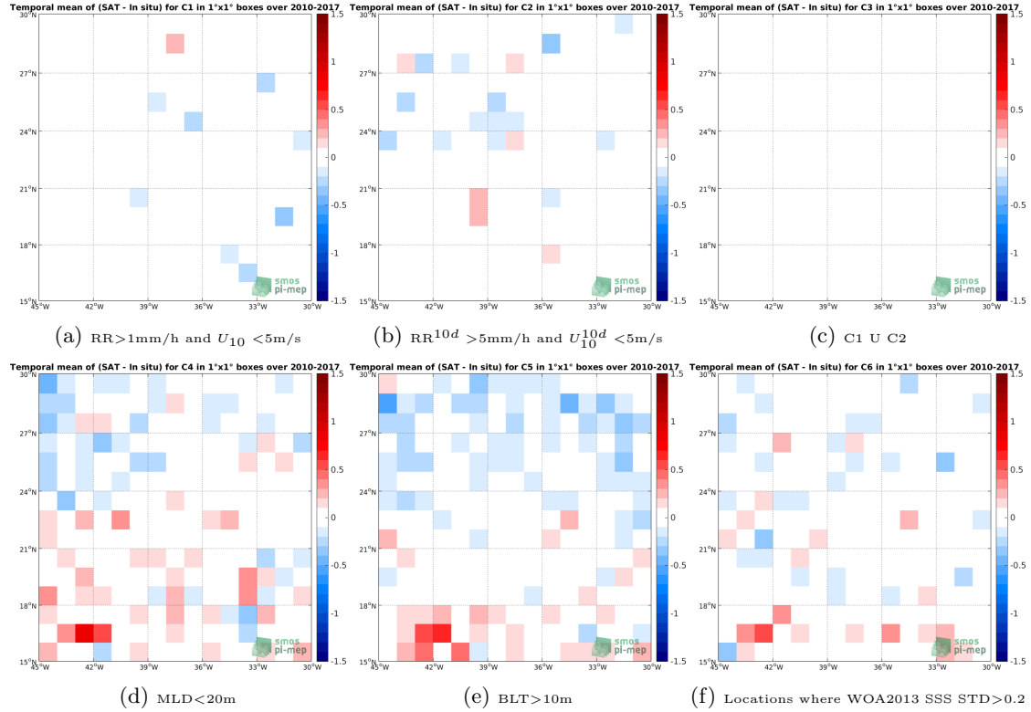
Figure 12: Temporal mean gridded over spatial boxes of size 1^\circ \times 1^\circ of \Delta\text{SSS} (SMOS-L3-CATDS-IFREMER-CECOS-V2-MONTHLY-0.25DEG - Argo) for 6 different subdatasets corresponding to: \text{RR} > 1\text{mm/h} and U_{10} < 5\text{m/s} (a), \text{RR}^{10d} > 5\text{mm/h} and U_{10}^{10d} < 5\text{m/s} (b), C1 U C2 (c), \text{MLD} < 20\text{m} (d), \text{BLT} > 10\text{m} (e), Locations where WOA2013 SSS STD > 0.2 (f).
