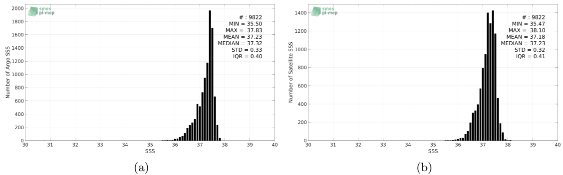
Figure 2: Histograms of SSS from Argo (a) and SMOS-L3-CATDS-IFREMER-CECOS-V2-MONTHLY-0.25DEG (b) considering all match-up pairs per bins of 0.1 over the SPURS 1 Pi-MEP region and for the full satellite product period.
