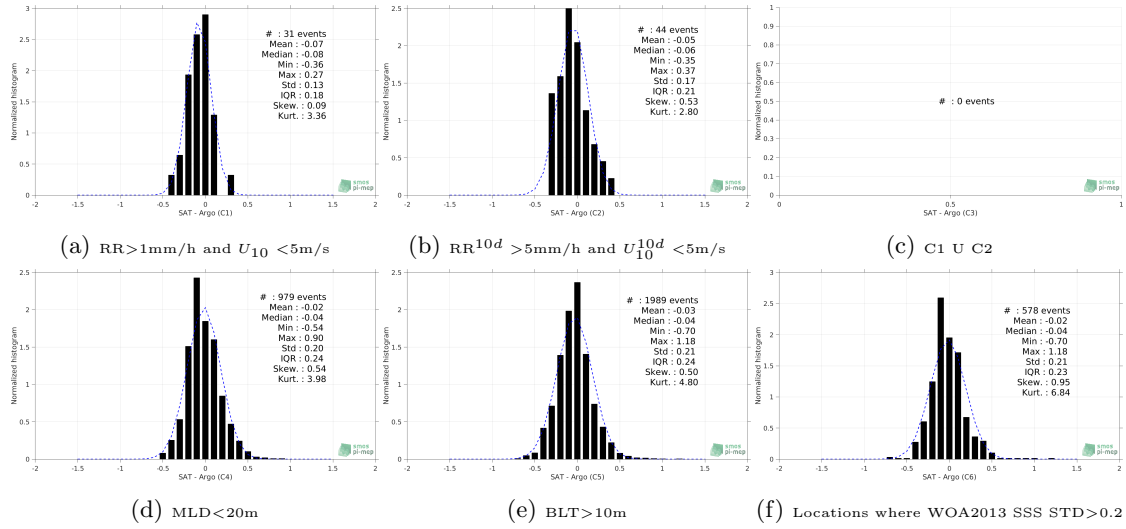
Figure 13: Normalized histogram of \Delta\text{SSS} (SMOS-L3-CATDS-IFREMER-CECOS-V2-MONTHLY-0.25DEG - Argo) for 6 different subdatasets corresponding to: RR>1mm/h and U_{10} < 5\text{m/s} (a), \text{RR}^{10d} > 5\text{mm/h} and U_{10}^{10d} < 5\text{m/s} (b), C1 U C2 (c),MLD<20m (d),BLT>10m (e),Locations where WOA2013 SSS STD>0.2 (f).
