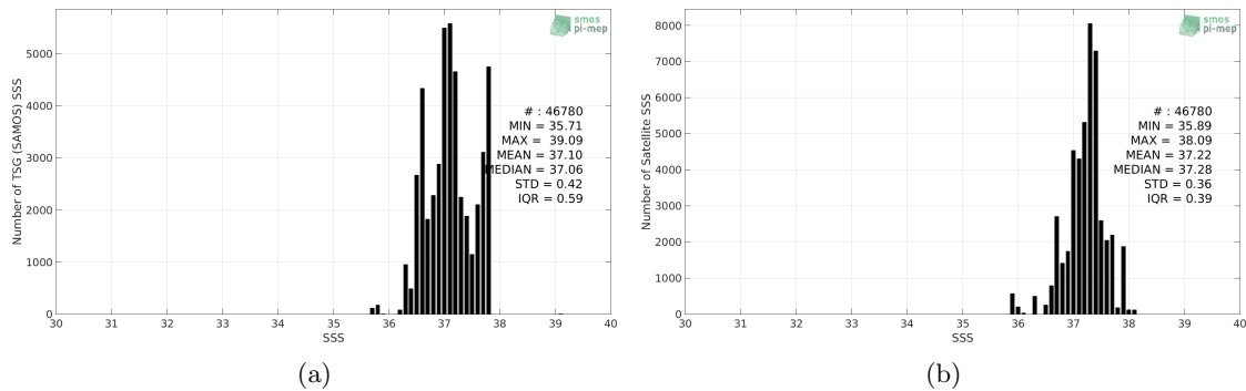
Figure 2: Histograms of SSS from TSG (SAMOS) (a) and SMOS SSS L3 v2 - Daily - 0.5 Deg (CATDS-CECOS-IFREMER) (b) considering all match-up pairs per bins of 0.1 over the SPURS 1 Pi-MEP region and for the full satellite product period.
