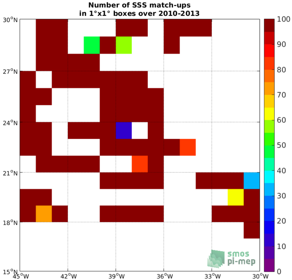
Figure 4: Number of SSS match-ups between TSG (SAMOS) SSS and the SMOS SSS L3 v2 - Daily - 0.5 Deg (CATDS-CECOS-IFREMER) SSS product for the SPURS 1 Pi-MEP region over 1°x1° boxes and for the full satellite product period.
