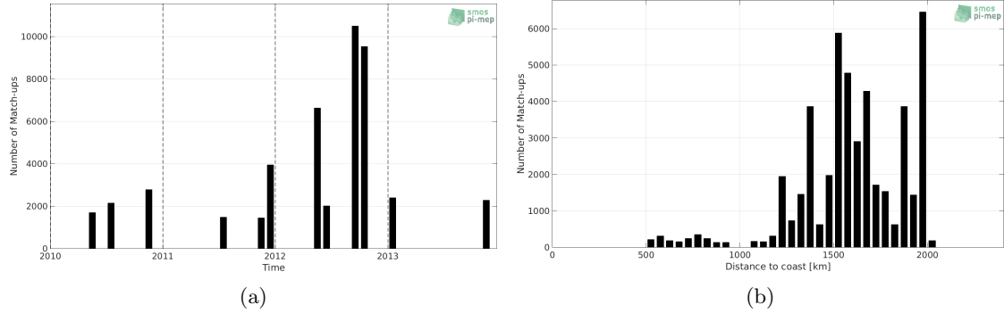
Figure 1: Number of match-ups between TSG (SAMOS) and SMOS SSS L3 v2 - Daily - 0.5 Deg (CATDS-CECOS-IFREMER) SSS as a function of time (a) and as function of the distance to coast (b) over the SPURS 1 Pi-MEP region and for the full satellite product period.
