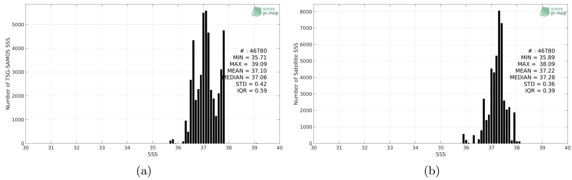
Figure 2: Histograms of SSS from TSG-SAMOS (a) and SMOS L3 v2 - Daily - 0.5 Deg (CATDS-CECOS-IFREMER) (b) considering all match-up pairs per bins of 0.1 over the SPURS 1 Pi-MEP region and for the full satellite product period.
