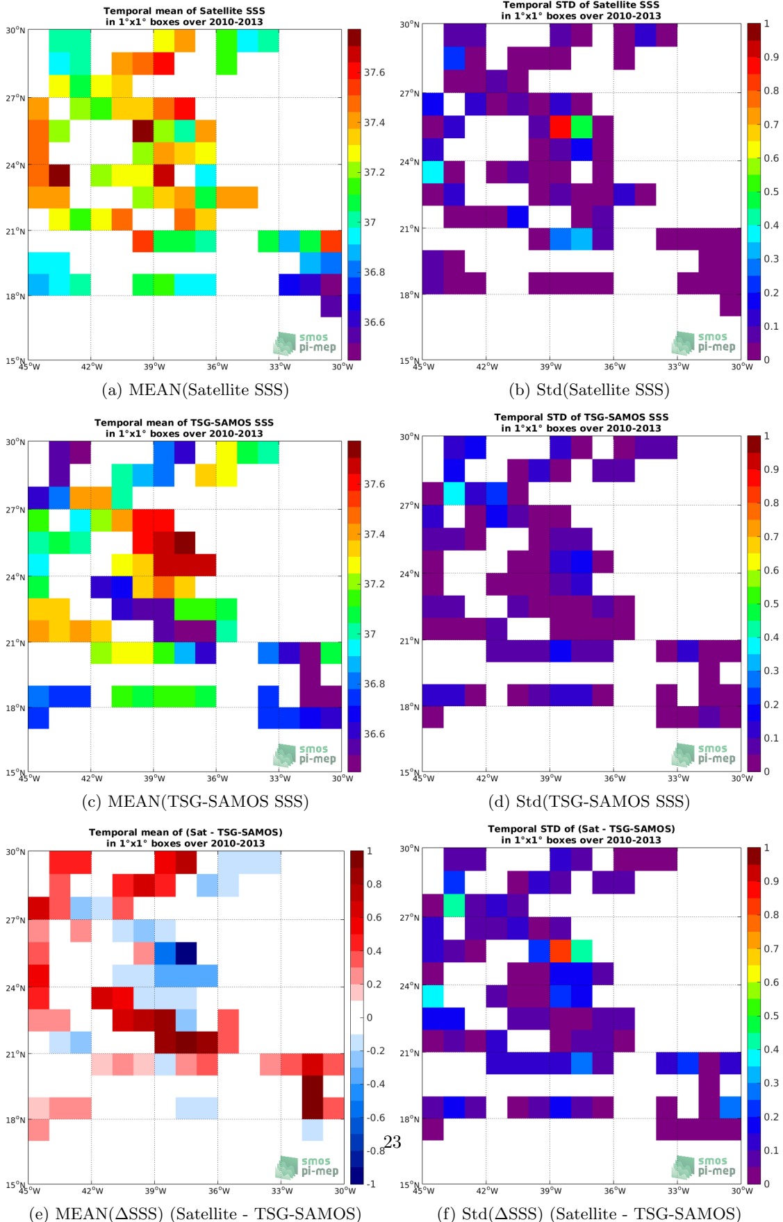
Figure 6: Temporal mean (left) and Std (right) of SSS from SMOS L3 v2 - Daily - 0.5 Deg (CATDS-CECOS-IFREMER) (top), TSG-SAMOS (middle), and of \Delta SSS (Satellite - TSG-SAMOS). Only match-up pairs are used to generate these maps.
