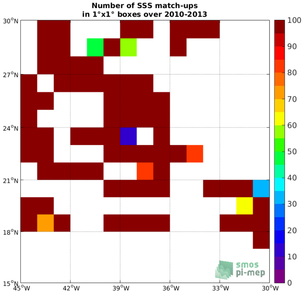
Figure 4: Number of SSS match-ups between TSG-SAMOS SSS and the SMOS L3 v2 - Daily - 0.5 Deg (CATDS-CECOS-IFREMER) SSS product for the SPURS 1 Pi-MEP region over 1°x1° boxes and for the full satellite product period.
