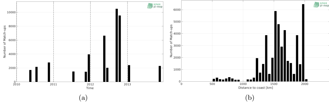
Figure 1: Number of match-ups between TSG-SAMOS and SMOS L3 v2 - Daily - 0.5 Deg (CATDS-CECOS-IFREMER) SSS as a function of time (a) and as function of the distance to coast (b) over the SPURS 1 Pi-MEP region and for the full satellite product period.
