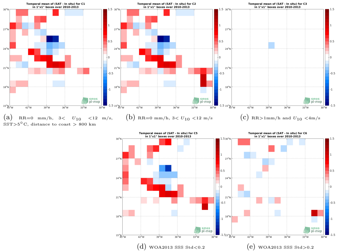
Figure 12: Temporal mean gridded over spatial boxes of size 1^\circ \times 1^\circ of \Delta SSS (SMOS-L3-CATDS-CECOS-IFREMER-V2-1DAY-0.5DEG - TSG-SAMOS) for 5 different subdatasets corresponding to:RR=0 mm/h, 3 < U_{10} < 12 m/s, SST >5^\circ C, distance to coast > 800 km (a), RR=0 mm/h, 3 < U_{10} < 12 m/s (b), RR >1 mm/h and U_{10} < 4 m/s (c), WOA2013 SSS Std <0.2 (d), WOA2013 SSS Std >0.2 (e).
