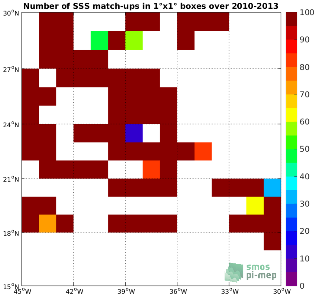
Figure 4: Number of SSS match-ups between TSG-SAMOS SSS and the SMOS-L3-CATDS-CECOS-IFREMER-V2-1DAY-0.5DEG SSS product for the SPURS 1 Pi-MEP region over 1°x1° boxes and for the full satellite product period.
