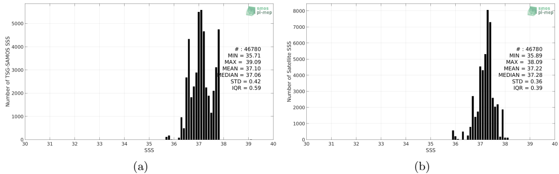
Figure 2: Histograms of SSS from TSG-SAMOS (a) and SMOS-L3-CATDS-CECOS-IFREMER-V2-1DAY-0.5DEG (b) considering all match-up pairs per bins of 0.1 over the SPURS 1 Pi-MEP region and for the full satellite product period.
