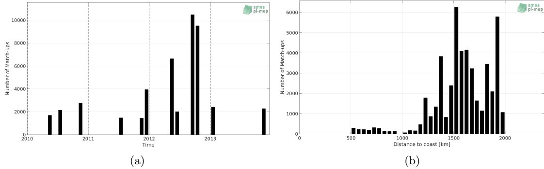
Figure 1: Number of match-ups between TSG-SAMOS and SMOS-L3-CATDS-CECOS-IFREMER-V2-1DAY-0.5DEG SSS as a function of time (a) and as function of the distance to coast (b) over the SPURS 1 Pi-MEP region and for the full satellite product period.
