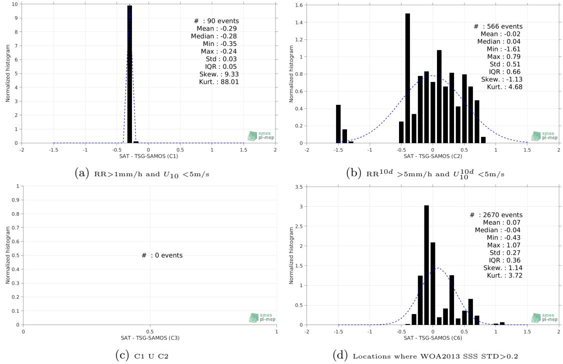
Figure 13: Normalized histogram of \Delta\text{SSS} (SMOS-L3-CATDS-CECOS-IFREMER-V2-1DAY-0.5DEG - TSG-SAMOS) for 6 different subdatasets corresponding to: RR > 1mm/h and U_{10} < 5\text{m/s} (a), RR^{10d} > 5\text{mm/h} and U_{10}^{10d} < 5\text{m/s} (b), C1 U C2 (c), Locations where WOA2013 SSS STD > 0.2 (d).
