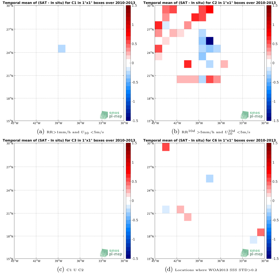
Figure 12: Temporal mean gridded over spatial boxes of size 1^\circ \times 1^\circ of \Delta SSS (SMOS-L3-CATDS-CECOS-IFREMER-V2-1DAY-0.5DEG - TSG-SAMOS) for 4 different subdatasets corresponding to: RR > 1\text{mm/h} and U_{10} < 5\text{m/s} (a), RR^{10d} > 5\text{mm/h} and U_{10}^{10d} < 5\text{m/s} (b), C1 U C2 (c), Locations where WOA2013 SSS STD > 0.2 (d).
