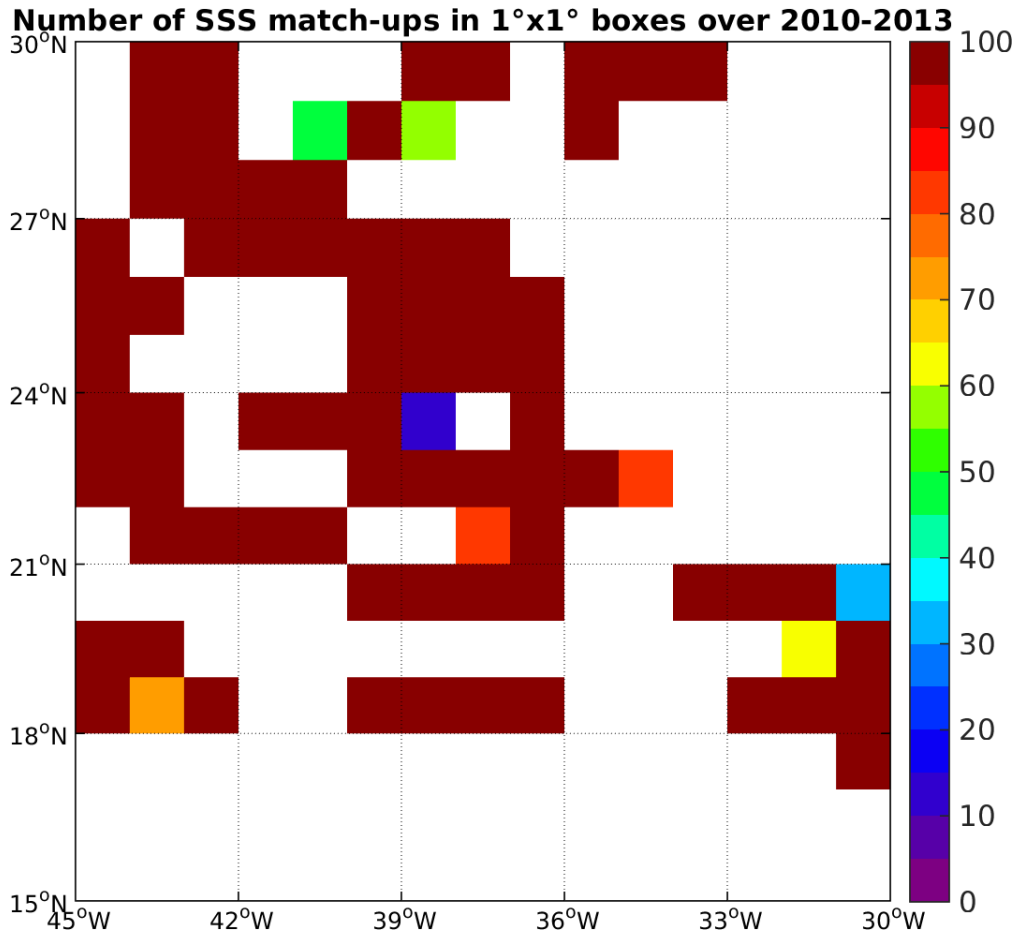
Figure 4: Number of SSS match-ups between TSG-SAMOS SSS and the SMOS-L3-CATDS-CECOS-IFREMER-V2-1DAY-0.5deg SSS product for the SPURS 1 Pi-MEP region over 1°x1° boxes and for the full satellite product period.
