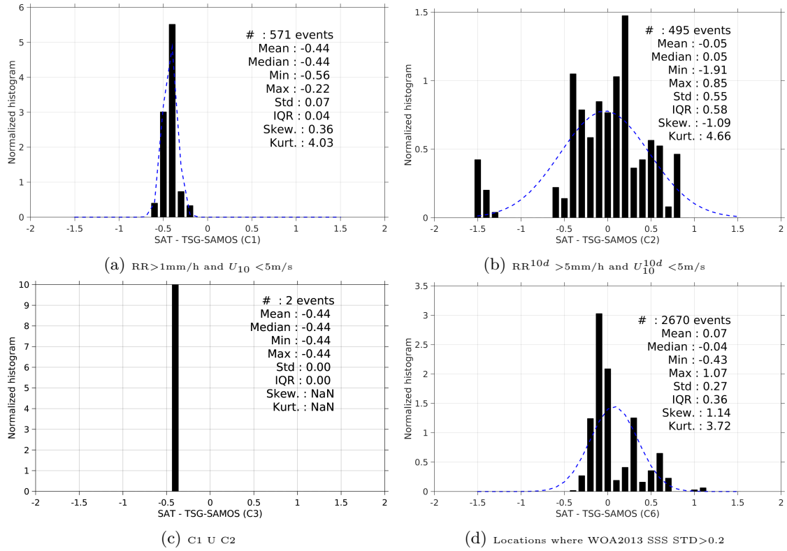
Figure 13: Normalized histogram of \Delta SSS (SMOS-L3-CATDS-CECOS-IFREMER-V2-1DAY-0.5deg - TSG-SAMOS) for 6 different subdatasets corresponding to: RR > 1mm/h and U_{10} < 5 m/s (a), RR^{10d} > 5 mm/h and U_{10}^{10d} < 5 m/s (b), C1 U C2 (c), Locations where WOA2013 SSS STD > 0.2 (d).
