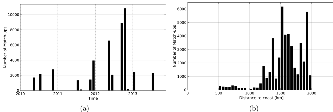
Figure 1: Number of match-ups between TSG-SAMOS and SMOS-L3-CATDS-CECOS-IFREMER-V2-1DAY-0.5deg SSS as a function of time (a) and as function of the distance to coast (b) over the SPURS 1 Pi-MEP region and for the full satellite product period.
