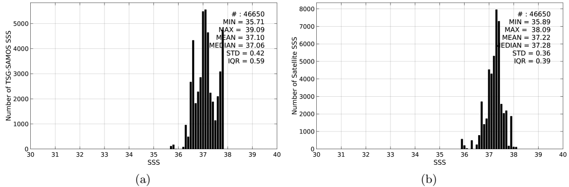
Figure 2: Histograms of SSS from TSG-SAMOS (a) and SMOS-L3-CATDS-CECOS-IFREMER-V2-1DAY-0.5deg (b) considering all match-up pairs per bins of 0.1 over the SPURS 1 Pi-MEP region and for the full satellite product period.
