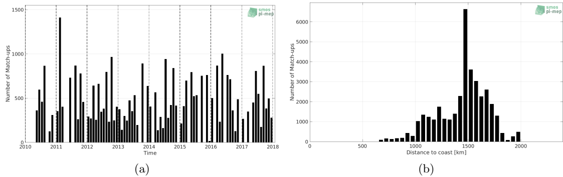
Figure 1: Number of match-ups between TSG (LEGOS-DM) and SMOS SSS L3 v2 - Daily - 0.5 Deg (CATDS-CECOS-IFREMER) SSS as a function of time (a) and as function of the distance to coast (b) over the SPURS 1 Pi-MEP region and for the full satellite product period.
