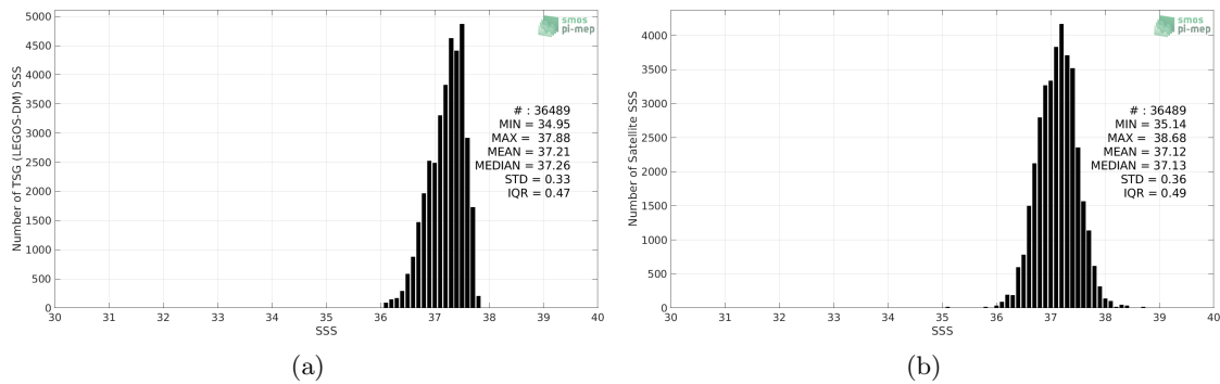
Figure 2: Histograms of SSS from TSG (LEGOS-DM) (a) and SMOS SSS L3 v2 - Daily - 0.5 Deg (CATDS-CECOS-IFREMER) (b) considering all match-up pairs per bins of 0.1 over the SPURS 1 Pi-MEP region and for the full satellite product period.
