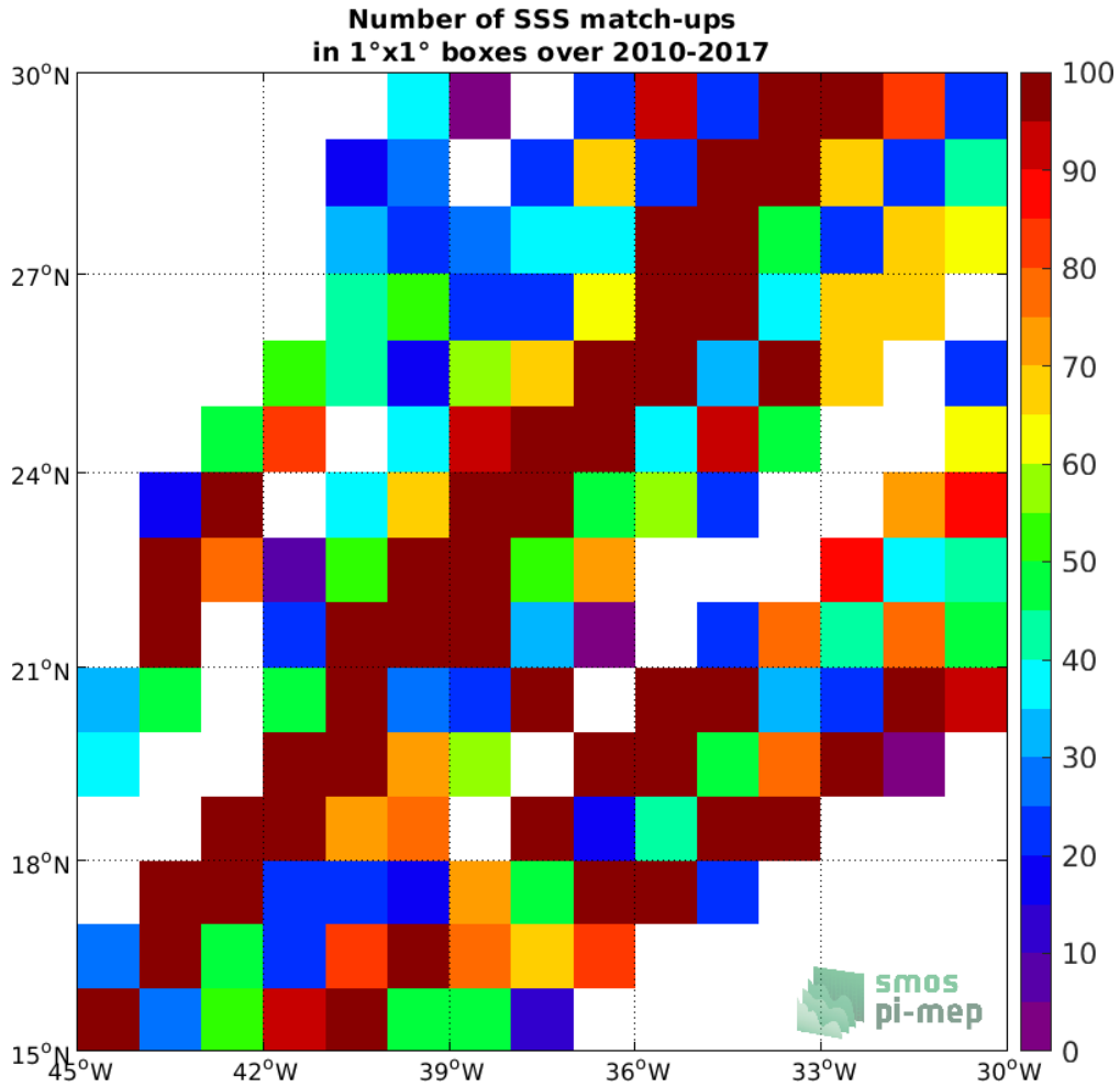
Figure 4: Number of SSS match-ups between TSG (LEGOS-DM) SSS and the SMOS SSS L3 v2 - Daily - 0.5 Deg (CATDS-CECOS-IFREMER) SSS product for the SPURS 1 Pi-MEP region over 1°x1° boxes and for the full satellite product period.
