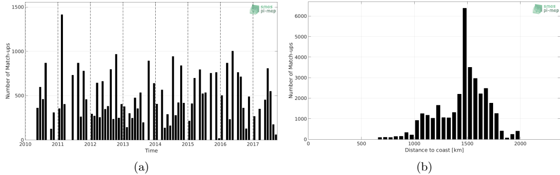
Figure 1: Number of match-ups between TSG-LEGOS-DM and SMOS L3 v2 - Daily - 0.5 Deg (CATDS-CECOS-IFREMER) SSS as a function of time (a) and as function of the distance to coast (b) over the SPURS 1 Pi-MEP region and for the full satellite product period.
