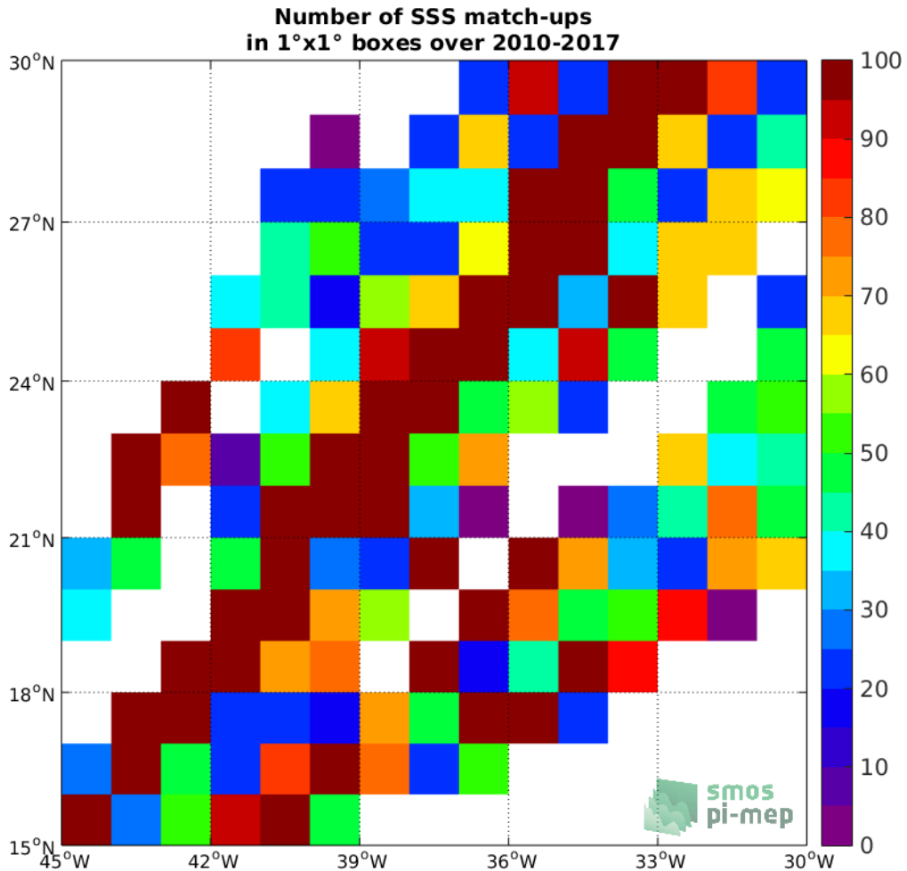
Figure 4: Number of SSS match-ups between TSG-LEGOS-DM SSS and the SMOS L3 v2 - Daily - 0.5 Deg (CATDS-CECOS-IFREMER) SSS product for the SPURS 1 Pi-MEP region over 1°x1° boxes and for the full satellite product period.
