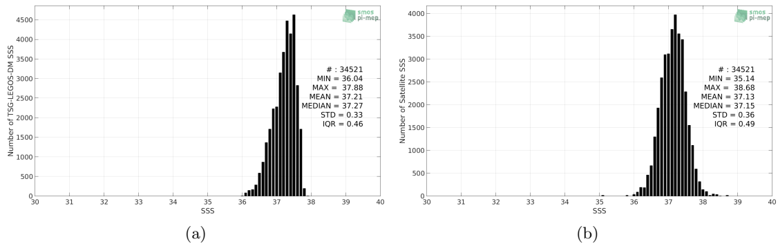
Figure 2: Histograms of SSS from TSG-LEGOS-DM (a) and SMOS L3 v2 - Daily - 0.5 Deg (CATDS-CECOS-IFREMER) (b) considering all match-up pairs per bins of 0.1 over the SPURS 1 Pi-MEP region and for the full satellite product period.
