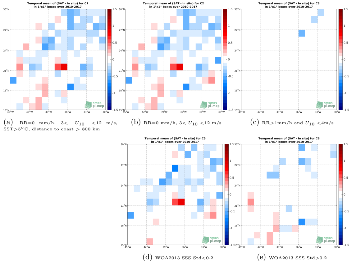
Figure 12: Temporal mean gridded over spatial boxes of size 1^\circ \times 1^\circ of \Delta SSS (SMOS-L3-CATDS-CECOS-IFREMER-V2-1DAY-0.5DEG - TSG-LEGOS-DM) for 5 different subdatasets corresponding to:RR=0 mm/h, 3 < U_{10} < 12 m/s, SST >5^\circ C, distance to coast > 800 km (a), RR=0 mm/h, 3 < U_{10} < 12 m/s (b), RR >1 mm/h and U_{10} < 4 m/s (c), WOA2013 SSS Std <0.2 (d), WOA2013 SSS Std >0.2 (e).
