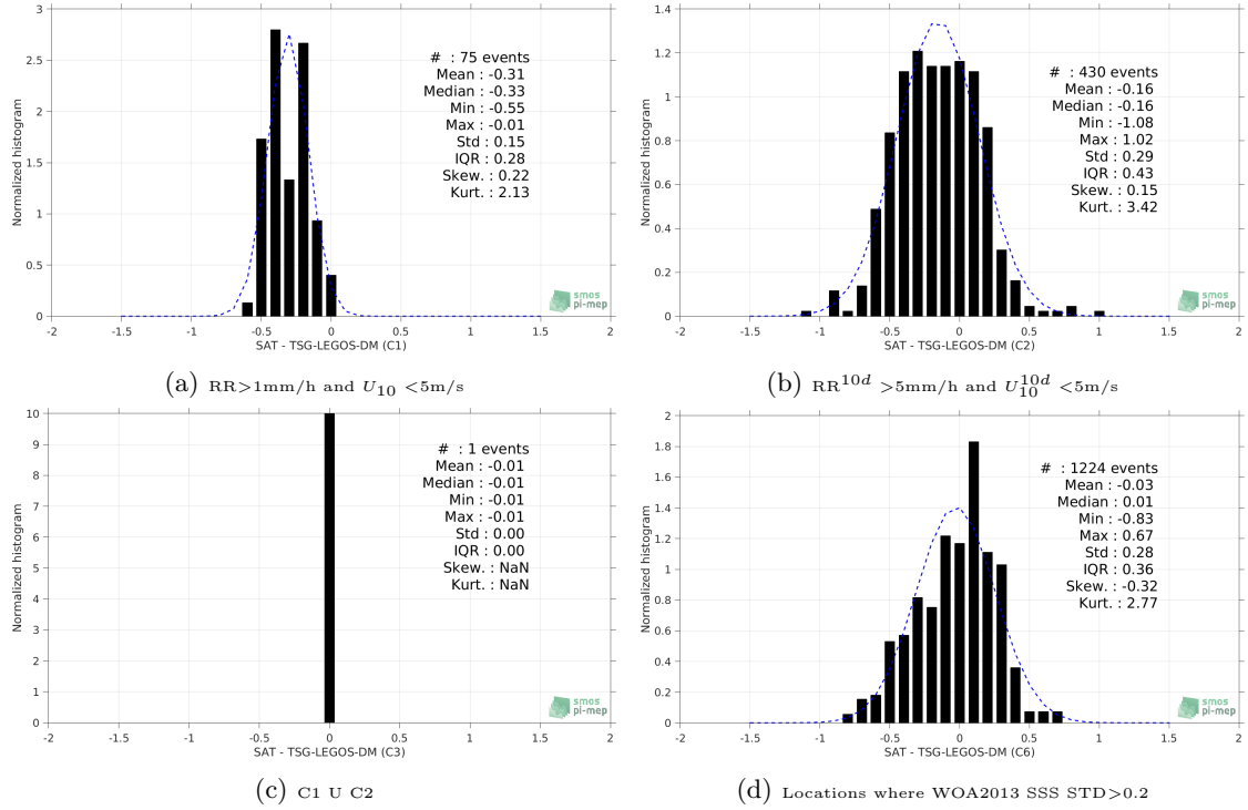
Figure 13: Normalized histogram of \Delta SSS (SMOS-L3-CATDS-CECOS-IFREMER-V2-1DAY-0.5DEG - TSG-LEGOS-DM) for 6 different subdatasets corresponding to: RR > 1\text{mm/h} and U_{10} < 5\text{m/s} (a), RR^{10d} > 5\text{mm/h} and U_{10}^{10d} < 5\text{m/s} (b), C1 U C2 (c), Locations where WOA2013 SSS STD > 0.2 (d).
