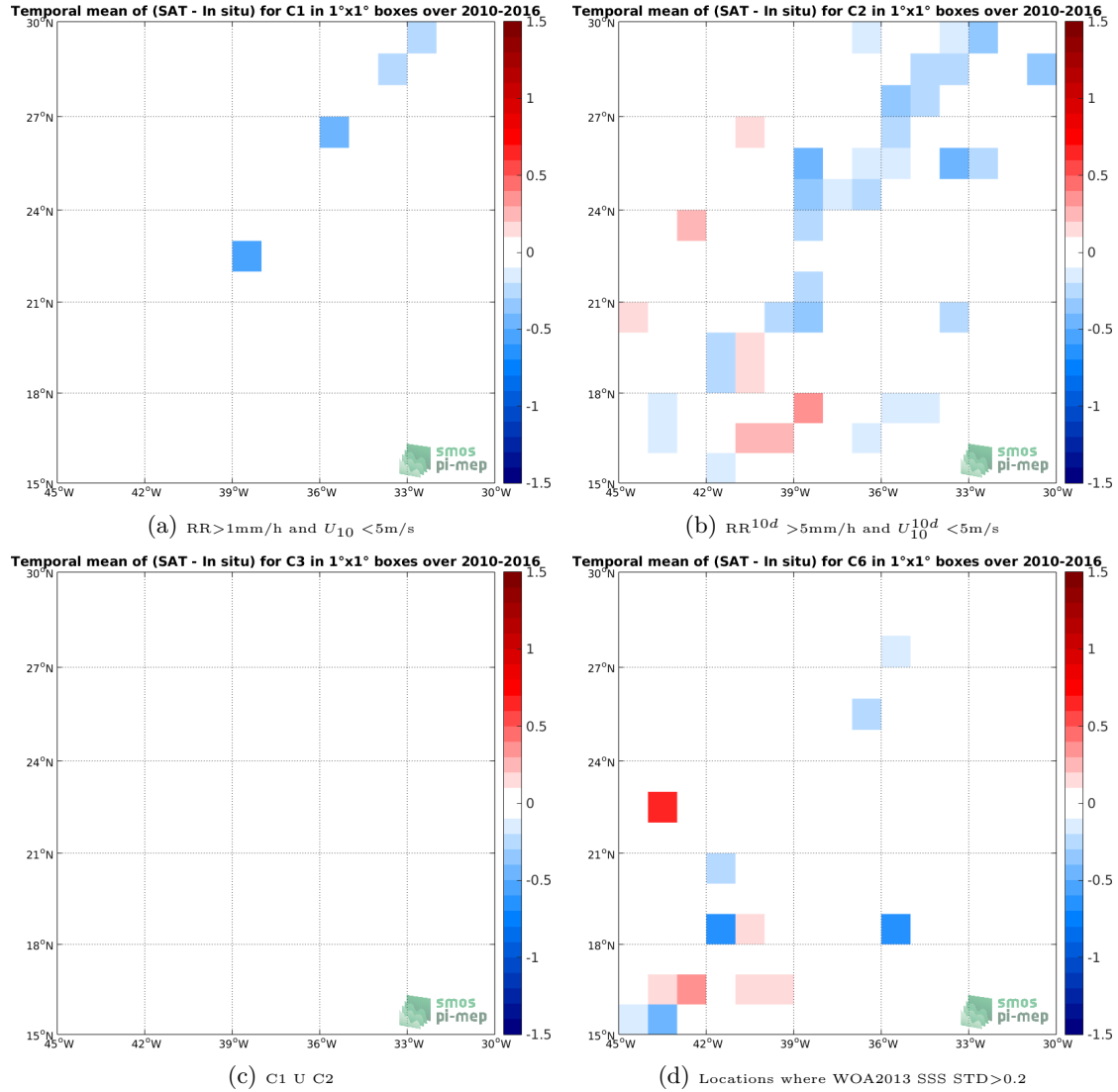
Figure 12: Temporal mean gridded over spatial boxes of size 1^\circ \times 1^\circ of \Delta SSS (SMOS-L3-CATDS-CECOS-IFREMER-V2-1DAY-0.5DEG - TSG-LEGOS-DM) for 4 different subdatasets corresponding to: RR > 1\text{mm/h} and U_{10} < 5\text{m/s} (a), RR^{10d} > 5\text{mm/h} and U_{10}^{10d} < 5\text{m/s} (b), C1 U C2 (c), Locations where WOA2013 SSS STD > 0.2 (d).
