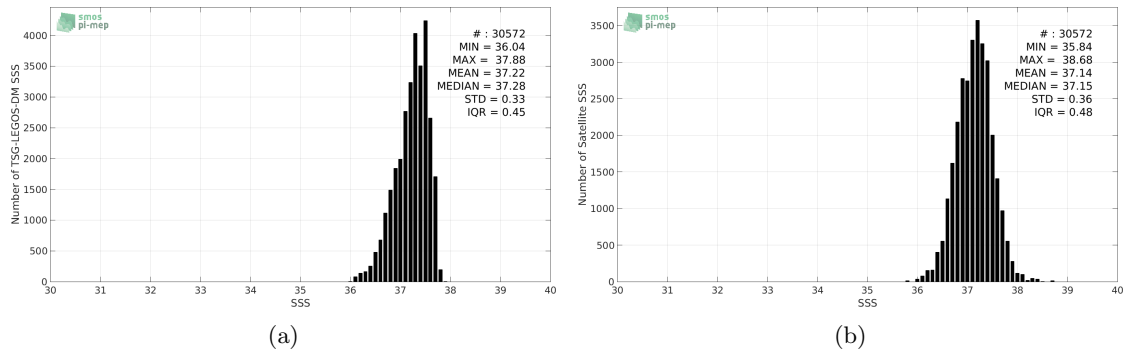
Figure 2: Histograms of SSS from TSG-LEGOS-DM (a) and SMOS-L3-CATDS-CECOS-IFREMER-V2-1DAY-0.5DEG (b) considering all match-up pairs per bins of 0.1 over the SPURS 1 Pi-MEP region and for the full satellite product period.
