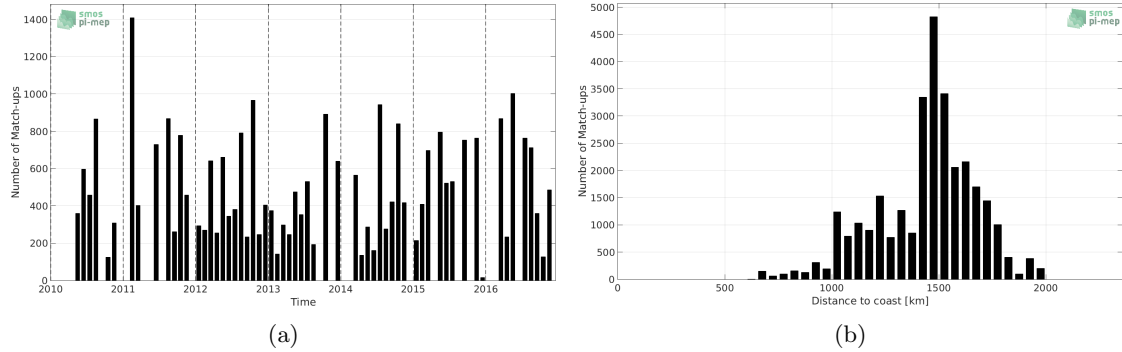
Figure 1: Number of match-ups between TSG-LEGOS-DM and SMOS-L3-CATDS-CECOS-IFREMER-V2-1DAY-0.5DEG SSS as a function of time (a) and as function of the distance to coast (b) over the SPURS 1 Pi-MEP region and for the full satellite product period.
