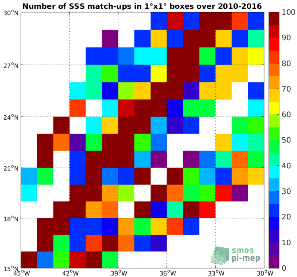
Figure 4: Number of SSS match-ups between TSG-LEGOS-DM SSS and the SMOS-L3-CATDS-CECOS-IFREMER-V2-1DAY-0.5DEG SSS product for the SPURS 1 Pi-MEP region over 1°x1° boxes and for the full satellite product period.
