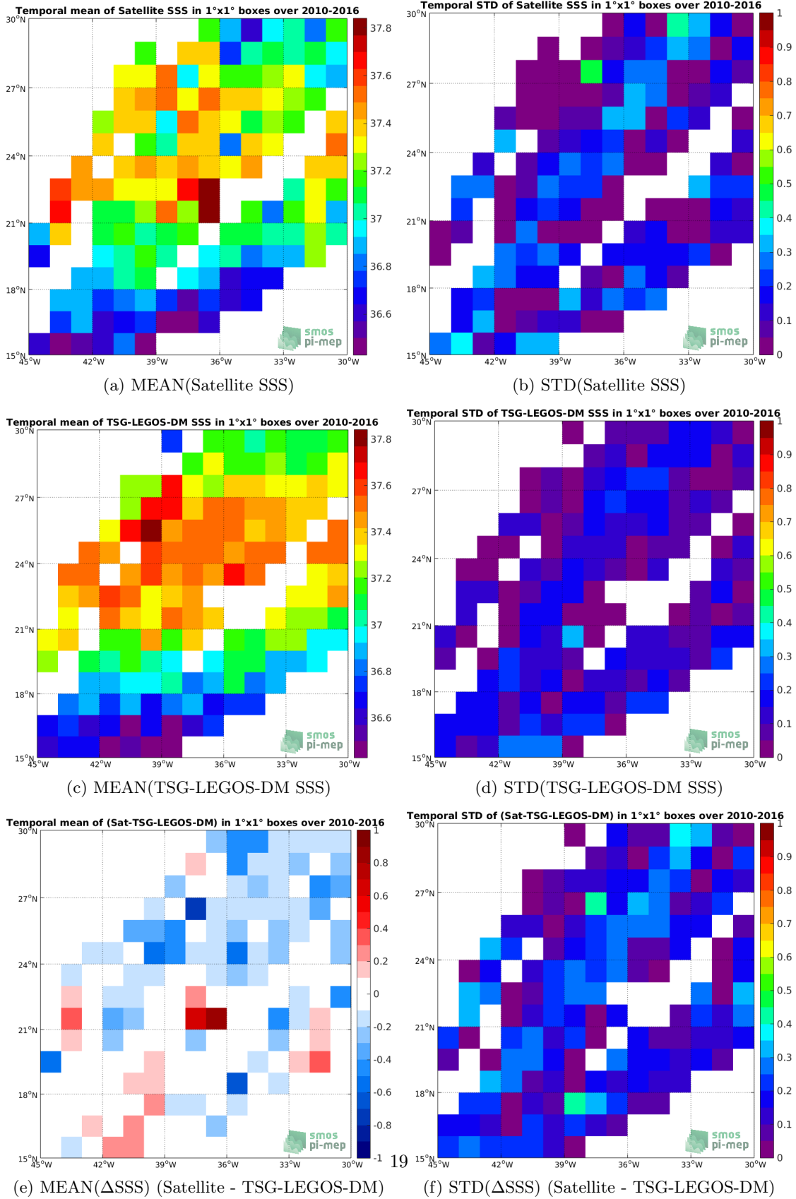
Figure 6: Temporal mean (left) and STD (right) of SSS from SMOS-L3-CATDS-CECOF-IFREMER-V2-1DAY-0.5DEG (top), TSG-LEGOS-DM (middle), and of \Delta SSS (Satellite - TSG-LEGOS-DM). Only match-up pairs are used to generate these maps.
