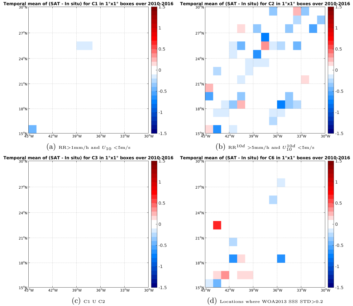
Figure 12: Temporal mean gridded over spatial boxes of size 1^\circ \times 1^\circ of \Delta\text{SSS} (SMOS-L3-CATDS-CECOS-IFREMER-V2-1DAY-0.5DEG - TSG-LEGOS-DM) for 4 different subdatasets corresponding to: RR > 1\text{mm/h} and U_{10} < 5\text{m/s} (a), RR^{10d} > 5\text{mm/h} and U_{10}^{10d} < 5\text{m/s} (b), C1 U C2 (c), Locations where WOA2013 SSS STD > 0.2 (d).
