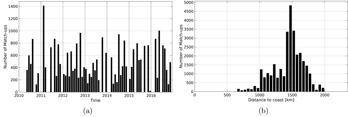
Figure 1: Number of match-ups between TSG-LEGOS-DM and SMOS-L3-CATDS-CECOS-IFREMER-V2-1DAY-0.5DEG SSS as a function of time (a) and as function of the distance to coast (b) over the SPURS 1 Pi-MEP region and for the full satellite product period.
