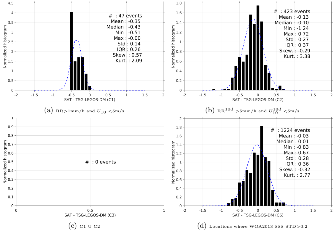
Figure 13: Normalized histogram of \Delta\text{SSS} (SMOS-L3-CATDS-CECOS-IFREMER-V2-1DAY-0.5DEG - TSG-LEGOS-DM) for 6 different subdatasets corresponding to: RR>1mm/h and U_{10} < 5\text{m/s} (a), \text{RR}^{10d} > 5\text{mm/h} and U_{10}^{10d} < 5\text{m/s} (b), C1 U C2 (c), Locations where WOA2013 SSS STD>0.2 (d).
