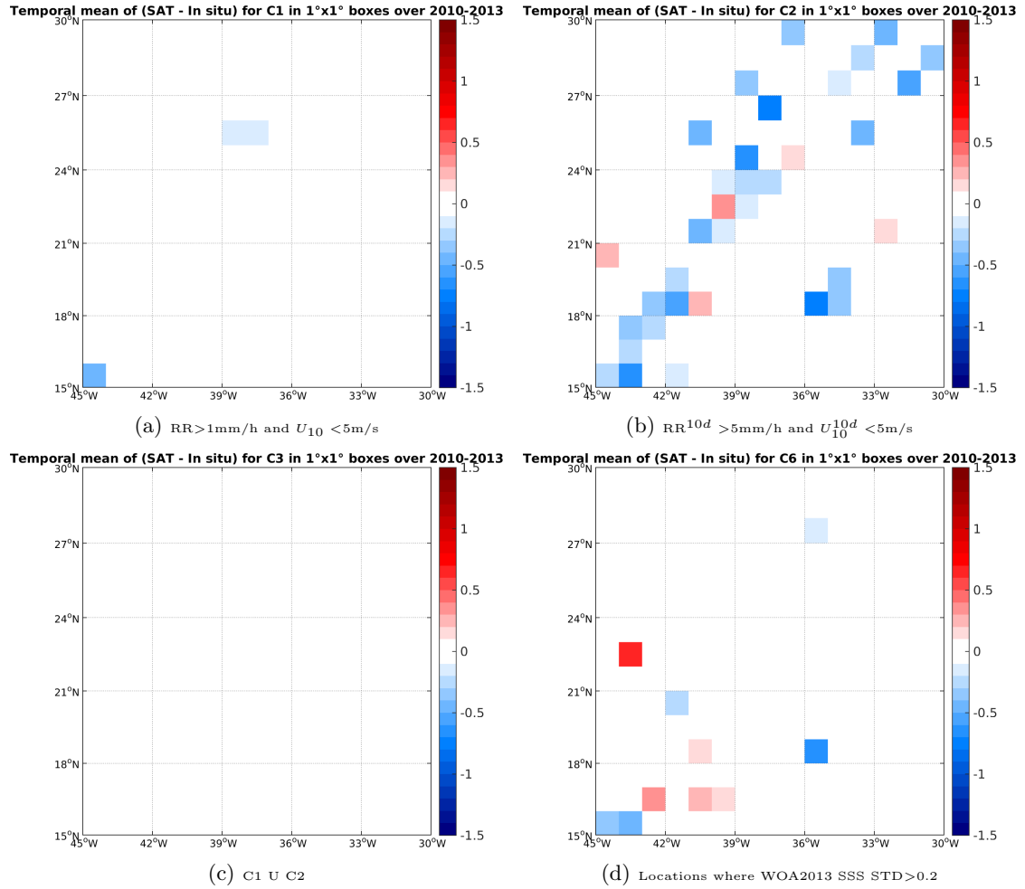
Figure 12: Temporal mean gridded over spatial boxes of size 1^\circ \times 1^\circ of \Delta SSS (SMOS-L3-CATDS-CECOS-IFREMER-V2-1DAY-0.5deg - TSG-LEGOS-DM) for 4 different subdatasets corresponding to: RR > 1\text{mm/h} and U_{10} < 5\text{m/s} (a), RR^{10d} > 5\text{mm/h} and U_{10}^{10d} < 5\text{m/s} (b), C1 U C2 (c), Locations where WOA2013 SSS STD > 0.2 (d).
