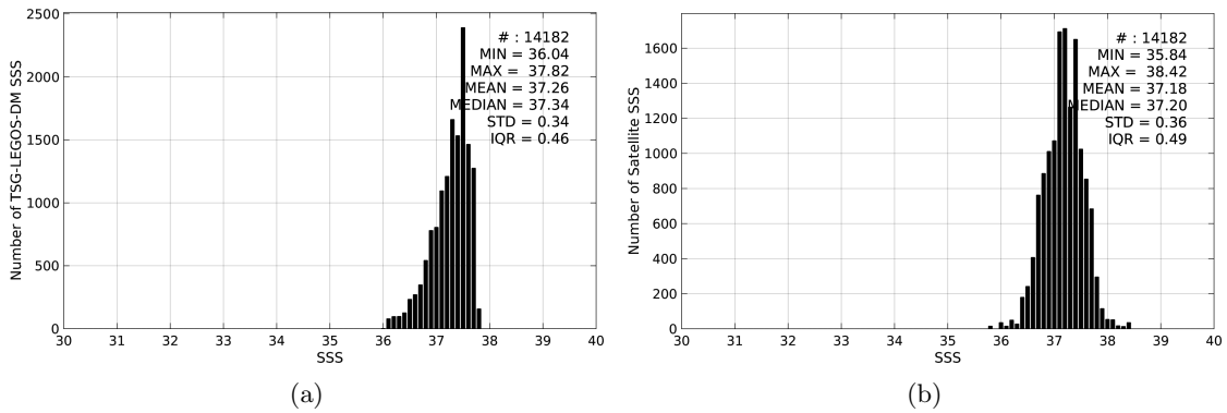
Figure 2: Histograms of SSS from TSG-LEGOS-DM (a) and SMOS-L3-CATDS-CECOS-IFREMER-V2-1DAY-0.5deg (b) considering all match-up pairs per bins of 0.1 over the SPURS 1 Pi-MEP region and for the full satellite product period.
