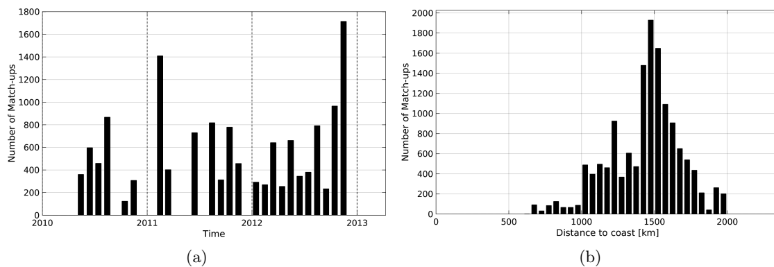
Figure 1: Number of match-ups between TSG-LEGOS-DM and SMOS-L3-CATDS-CECOS-IFREMER-V2-1DAY-0.5deg SSS as a function of time (a) and as function of the distance to coast (b) over the SPURS 1 Pi-MEP region and for the full satellite product period.
