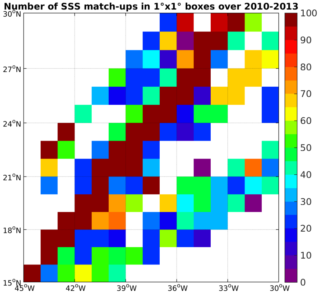
Figure 4: Number of SSS match-ups between TSG-LEGOS-DM SSS and the SMOS-L3-CATDS-CECOS-IFREMER-V2-1DAY-0.5deg SSS product for the SPURS 1 Pi-MEP region over 1°x1° boxes and for the full satellite product period.
