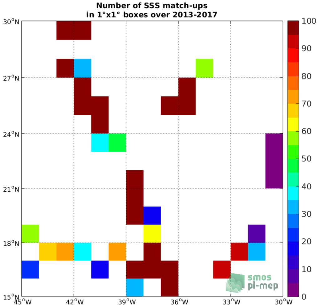
Figure 4: Number of SSS match-ups between TSG (GOSUD-Sailing-ship) SSS and the SMOS SSS L3 v2 - Daily - 0.5 Deg (CATDS-CECOS-IFREMER) SSS product for the SPURS 1 Pi-MEP region over 1°x1° boxes and for the full satellite product period.
