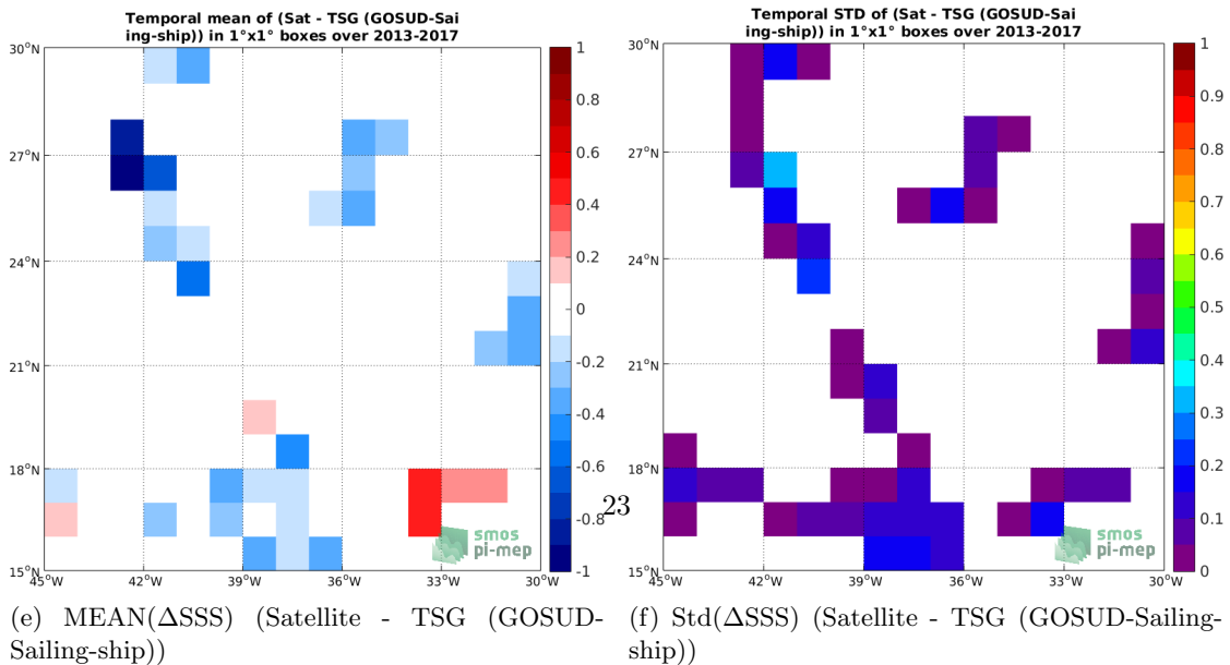
Figure 6: Temporal mean (left) and Std (right) of SSS from SMOS SSS L3 v2 - Daily - 0.5 Deg (CATDS-CECOS-IFREMER) (top), TSG (GOSUD-Sailing-ship) (middle), and of \Delta SSS (Satellite - TSG (GOSUD-Sailing-ship)). Only match-up pairs are used to generate these maps.
