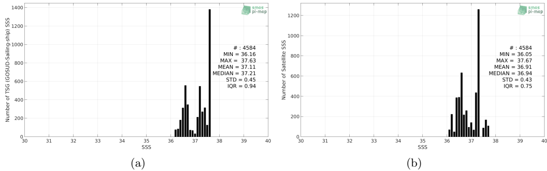
Figure 2: Histograms of SSS from TSG (GOSUD-Sailing-ship) (a) and SMOS SSS L3 v2 - Daily - 0.5 Deg (CATDS-CECOS-IFREMER) (b) considering all match-up pairs per bins of 0.1 over the SPURS 1 Pi-MEP region and for the full satellite product period.
