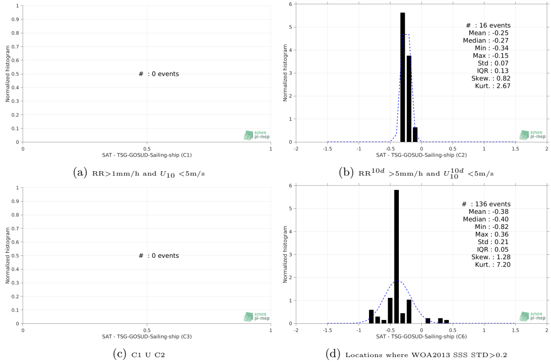
Figure 13: Normalized histogram of \Delta\text{SSS} (SMOS-L3-CATDS-CECOS-IFREMER-V2-1DAY-0.5DEG - TSG-GOSUD-Sailing-ship) for 6 different subdatasets corresponding to: RR > 1\text{mm/h} and U_{10} < 5\text{m/s} (a), RR^{10d} > 5\text{mm/h} and U_{10}^{10d} < 5\text{m/s} (b), C1 U C2 (c), Locations where WOA2013 SSS STD > 0.2 (d).
