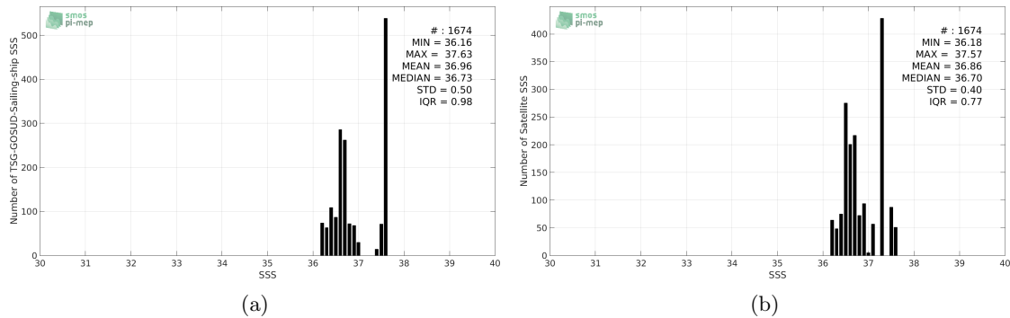
Figure 2: Histograms of SSS from TSG-GOSUD-Sailing-ship (a) and SMOS-L3-CATDS-CECOS-IFREMER-V2-1DAY-0.5DEG (b) considering all match-up pairs per bins of 0.1 over the SPURS 1 Pi-MEP region and for the full satellite product period.
