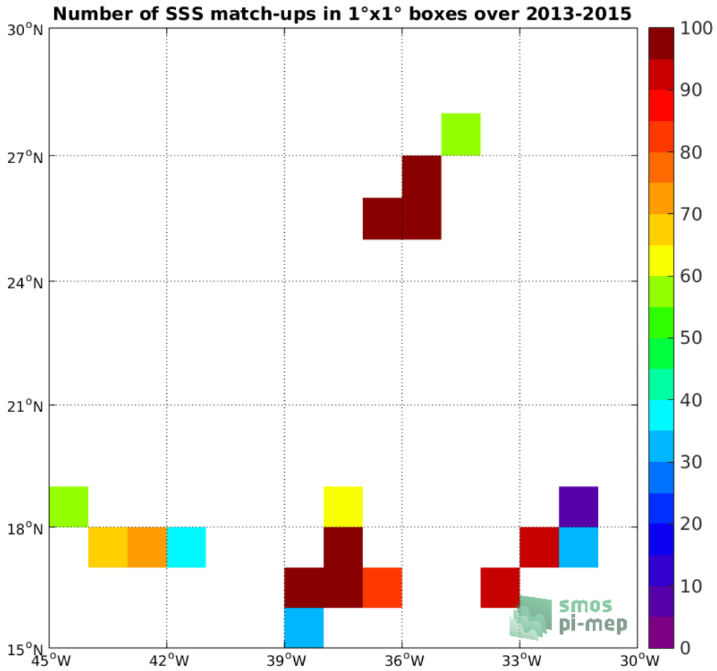
Figure 4: Number of SSS match-ups between TSG-GOSUD-Sailing-ship SSS and the SMOS-L3-CATDS-CECOS-IFREMER-V2-1DAY-0.5DEG SSS product for the SPURS 1 Pi-MEP region over 1°x1° boxes and for the full satellite product period.
