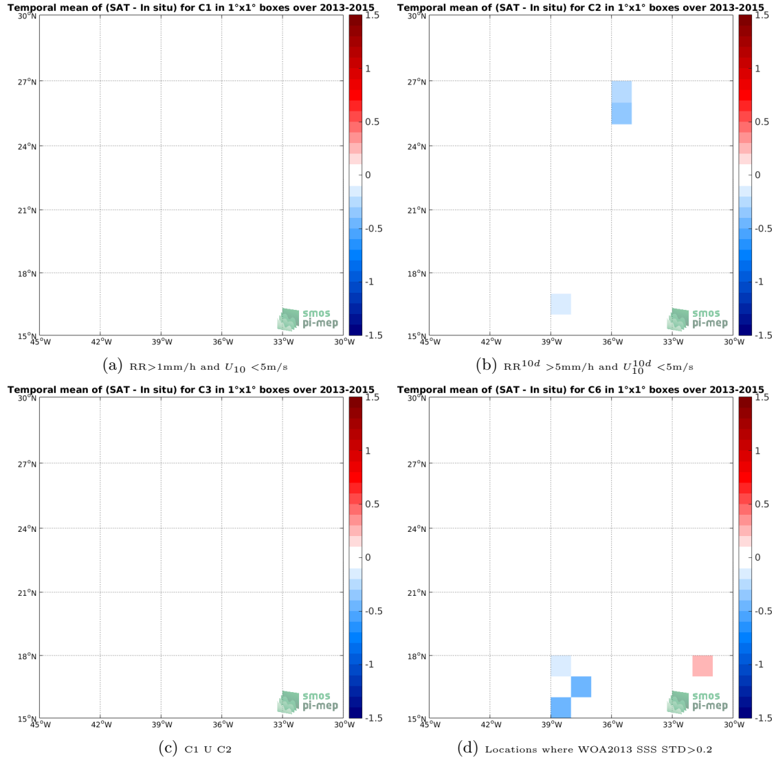
Figure 12: Temporal mean gridded over spatial boxes of size 1^\circ \times 1^\circ of \Delta SSS (SMOS-L3-CATDS-CECOS-IFREMER-V2-1DAY-0.5DEG - TSG-GOSUD-Sailing-ship) for 4 different subdatasets corresponding to: RR > 1\text{mm/h} and U_{10} < 5\text{m/s} (a), RR^{10d} > 5\text{mm/h} and U_{10}^{10d} < 5\text{m/s} (b), C1 U C2 (c), Locations where WOA2013 SSS STD > 0.2 (d).
