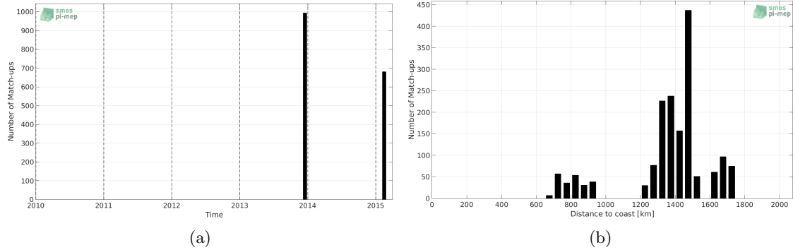
Figure 1: Number of match-ups between TSG-GOSUD-Sailing-ship and SMOS-L3-CATDS-CECOS-IFREMER-V2-1DAY-0.5DEG SSS as a function of time (a) and as function of the distance to coast (b) over the SPURS 1 Pi-MEP region and for the full satellite product period.
