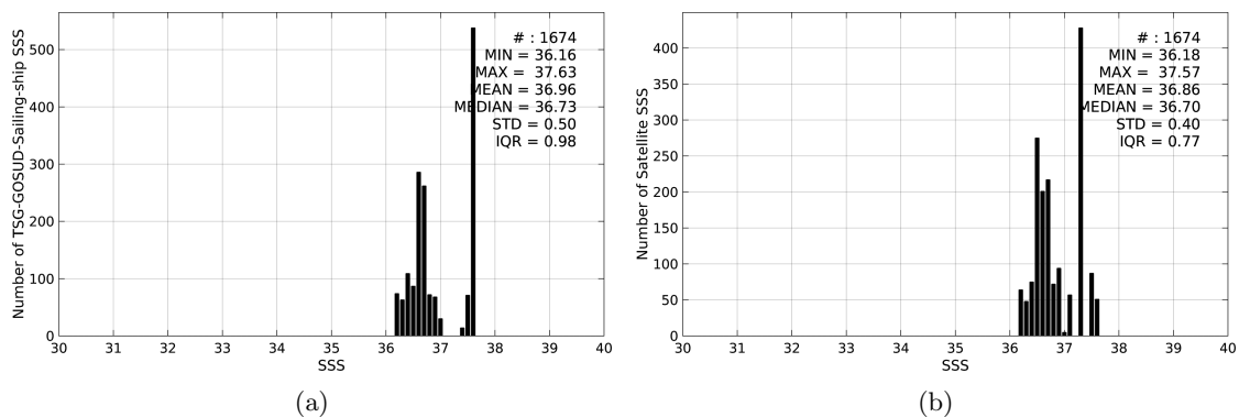
Figure 2: Histograms of SSS from TSG-GOSUD-Sailing-ship (a) and SMOS-L3-CATDS-CECOS-IFREMER-V2-1DAY-0.5DEG (b) considering all match-up pairs per bins of 0.1 over the SPURS 1 Pi-MEP region and for the full satellite product period.
