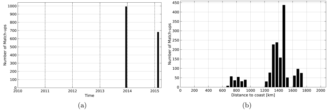
Figure 1: Number of match-ups between TSG-GOSUD-Sailing-ship and SMOS-L3-CATDS-CECOS-IFREMER-V2-1DAY-0.5DEG SSS as a function of time (a) and as function of the distance to coast (b) over the SPURS 1 Pi-MEP region and for the full satellite product period.
