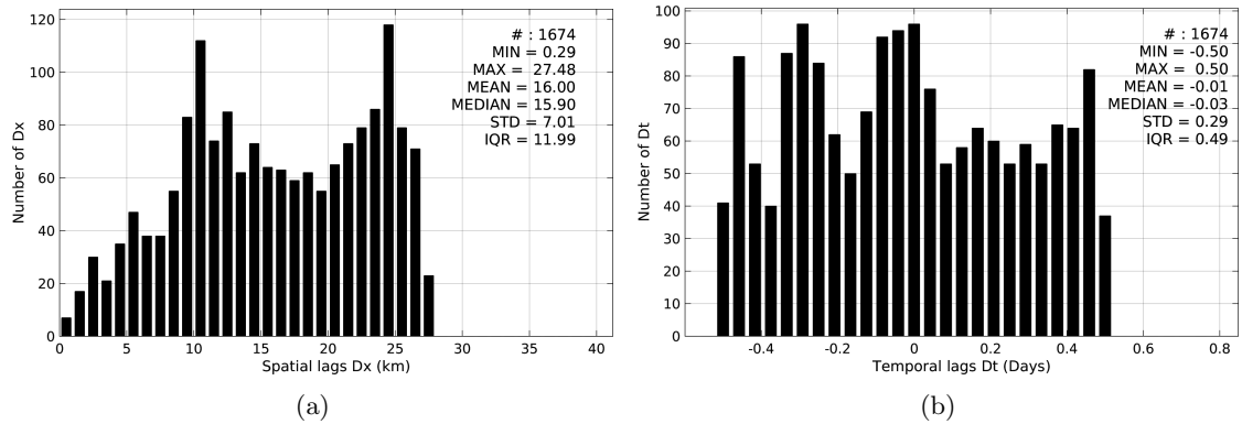
Figure 5: Histograms of the spatial (a) and temporal (b) lags between the time of the TSG-GOSUD-Sailing-ship measurements and the date of the corresponding SMOS-L3-CATDS-CECOS-IFREMER-V2-1DAY-0.5DEG SSS product.
