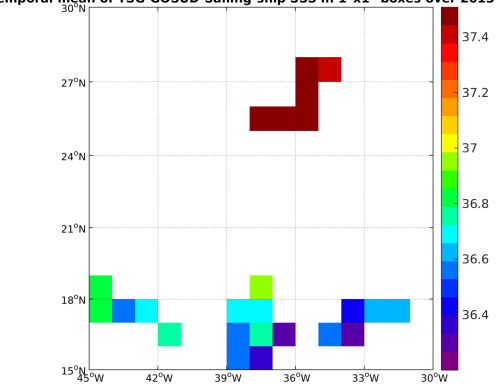
(c) MEAN(TSG-GOSUD-Sailing-ship SSS)
