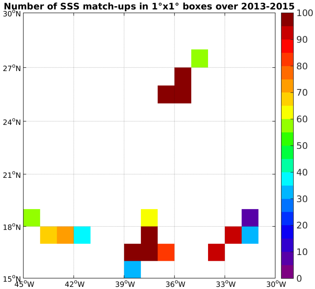
Figure 4: Number of SSS match-ups between TSG-GOSUD-Sailing-ship SSS and the SMOS-L3-CATDS-CECOS-IFREMER-V2-1DAY-0.5DEG SSS product for the SPURS 1 Pi-MEP region over 1°x1° boxes and for the full satellite product period.
