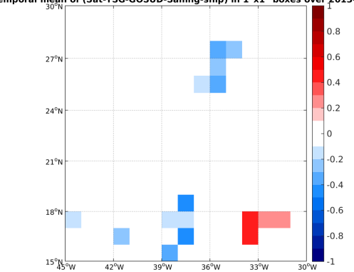
(e) MEAN( \Delta SSS) (Satellite - TSG-GOSUD-Sailing-ship)
