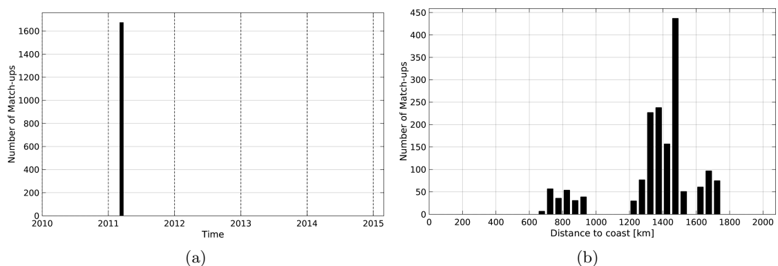
Figure 1: Number of match-ups between TSG-GOSUD-Sailing-ship and SMOS-L3-CATDS-CECOS-IFREMER-V2-1DAY-0.5deg SSS as a function of time (a) and as function of the distance to coast (b) over the SPURS 1 Pi-MEP region and for the full satellite product period.
