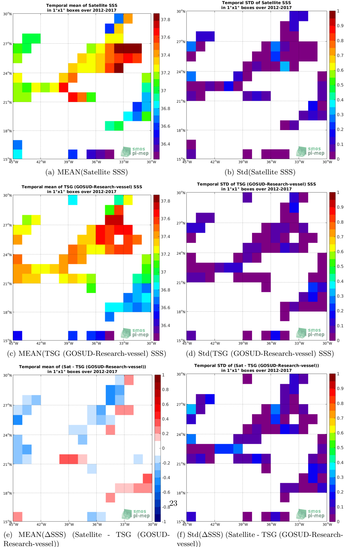
Figure 6: Temporal mean (left) and Std (right) of SSS from SMOS SSS L3 v2 - Daily - 0.5 Deg (CATDS-CECOS-IFREMER) (top), TSG (GOSUD-Research-vessel) (middle), and of \Delta SSS (Satellite - TSG (GOSUD-Research-vessel)). Only match-up pairs are used to generate these maps.
