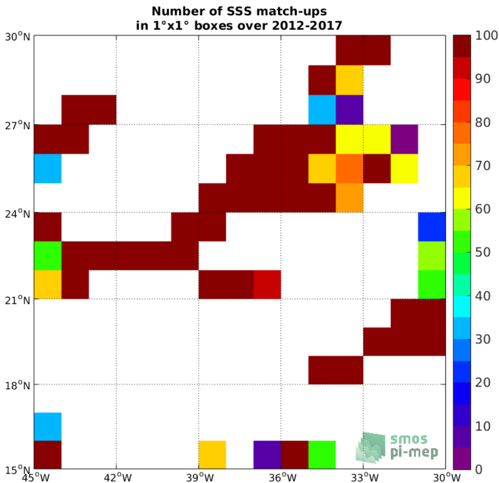
Figure 4: Number of SSS match-ups between TSG (GOSUD-Research-vessel) SSS and the SMOS SSS L3 v2 - Daily - 0.5 Deg (CATDS-CECOS-IFREMER) SSS product for the SPURS 1 Pi-MEP region over 1°x1° boxes and for the full satellite product period.
