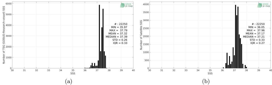
Figure 2: Histograms of SSS from TSG (GOSUD-Research-vessel) (a) and SMOS SSS L3 v2 - Daily - 0.5 Deg (CATDS-CECOS-IFREMER) (b) considering all match-up pairs per bins of 0.1 over the SPURS 1 Pi-MEP region and for the full satellite product period.
