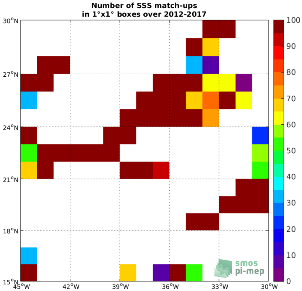
Figure 4: Number of SSS match-ups between TSG-GOSUD-Research-vessel SSS and the SMOS L3 v2 - Daily - 0.5 Deg (CATDS-CECOS-IFREMER) SSS product for the SPURS 1 Pi-MEP region over 1°x1° boxes and for the full satellite product period.
