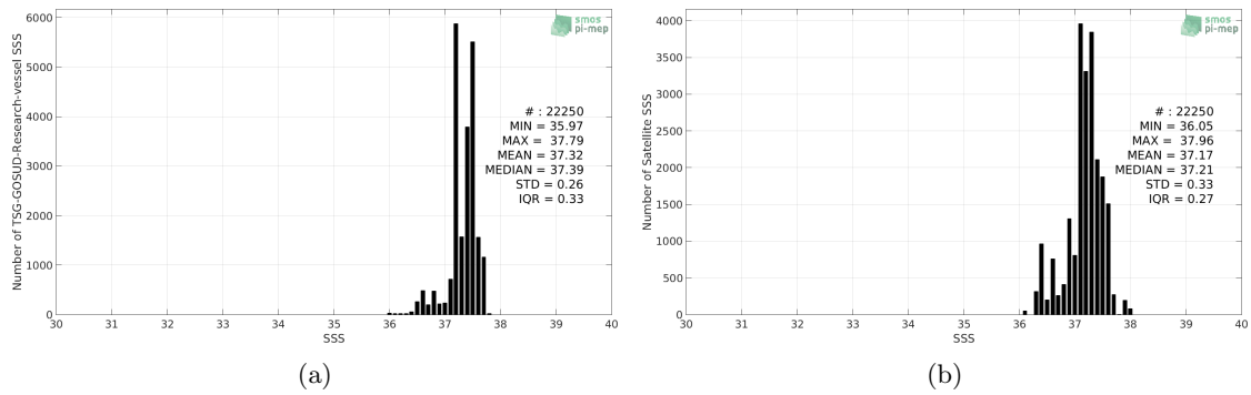
Figure 2: Histograms of SSS from TSG-GOSUD-Research-vessel (a) and SMOS L3 v2 - Daily - 0.5 Deg (CATDS-CECOS-IFREMER) (b) considering all match-up pairs per bins of 0.1 over the SPURS 1 Pi-MEP region and for the full satellite product period.
