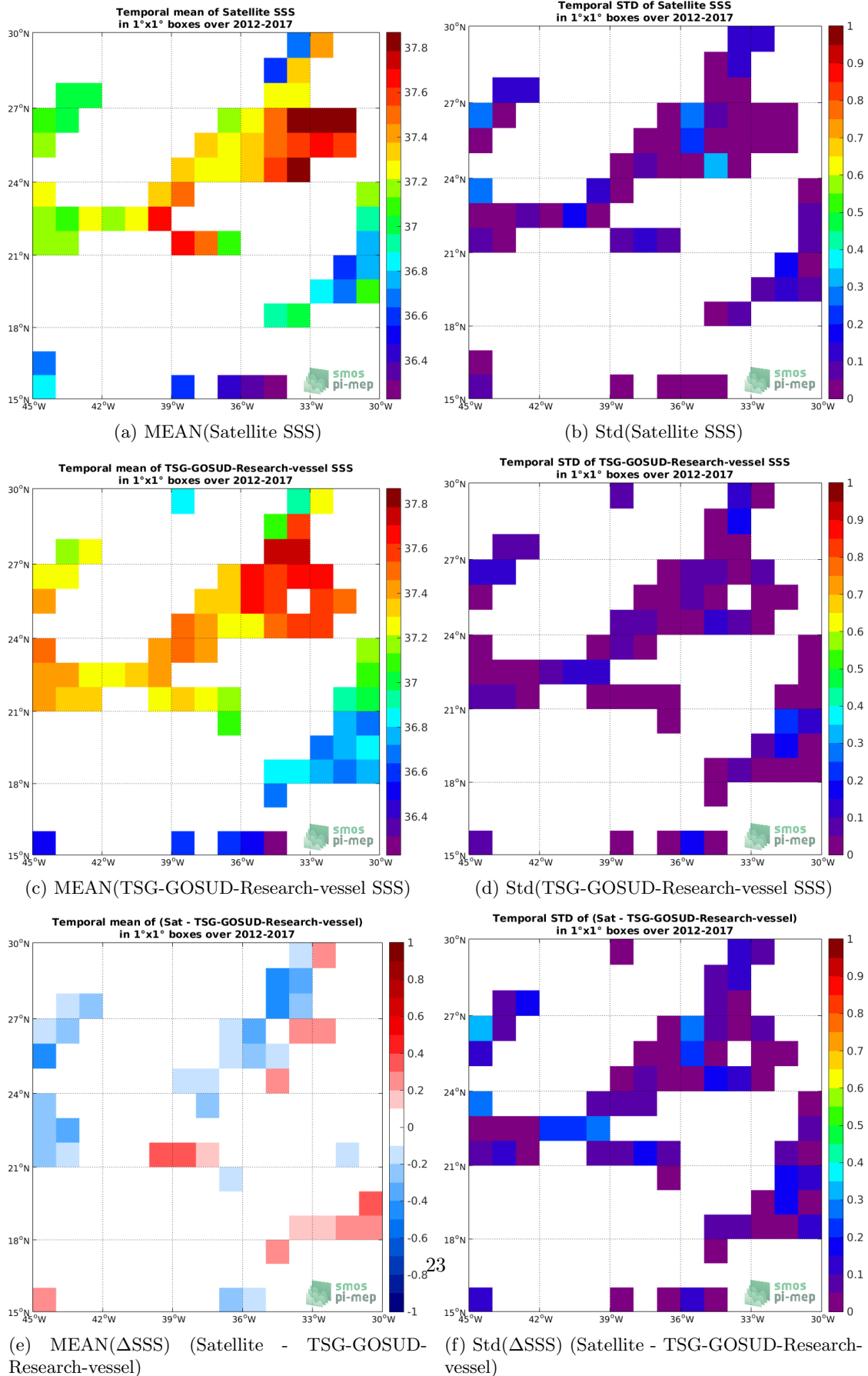
Figure 6: Temporal mean (left) and Std (right) of SSS from SMOS L3 v2 - Daily - 0.5 Deg (CATDS-CECOS-IFREMER) (top), TSG-GOSUD-Research-vessel (middle), and of \Delta SSS (Satellite - TSG-GOSUD-Research-vessel). Only match-up pairs are used to generate these maps.
