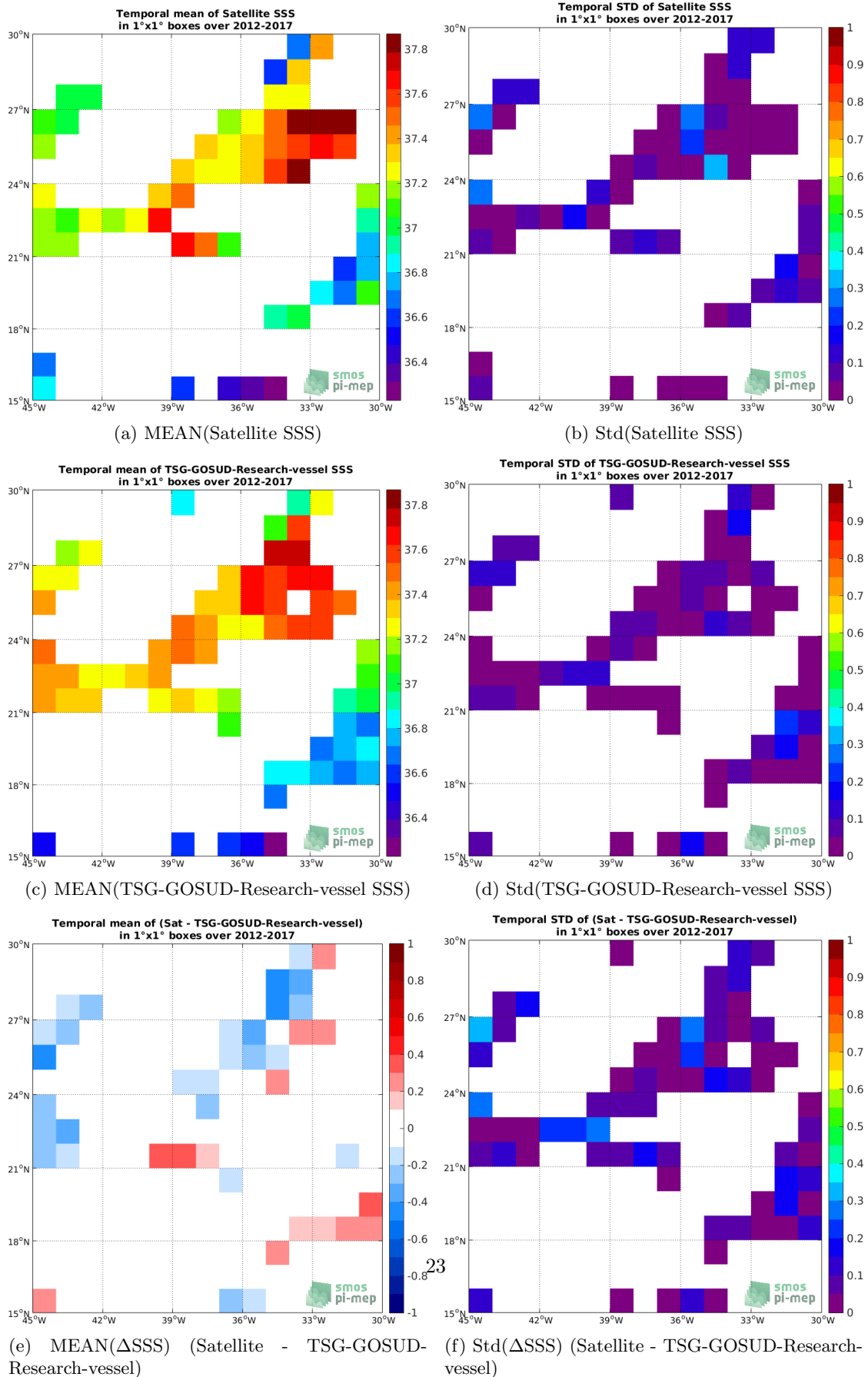
Figure 6: Temporal mean (left) and Std (right) of SSS from SMOS-L3-CATDS-CECOS-IFREMER-V2-1DAY-0.5DEG (top), TSG-GOSUD-Research-vessel (middle), and of \Delta SSS (Satellite - TSG-GOSUD-Research-vessel). Only match-up pairs are used to generate these maps.
