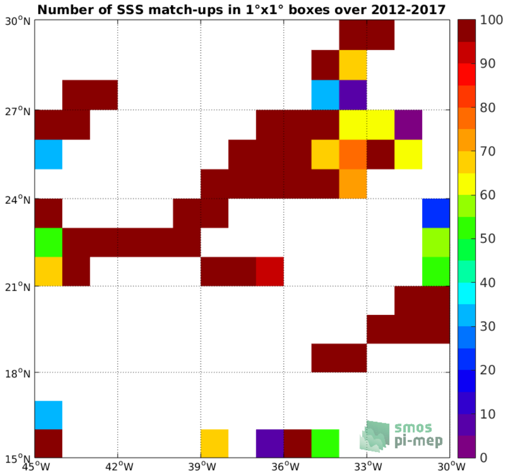
Figure 4: Number of SSS match-ups between TSG-GOSUD-Research-vessel SSS and the SMOS-L3-CATDS-CECOS-IFREMER-V2-1DAY-0.5DEG SSS product for the SPURS 1 Pi-MEP region over 1°x1° boxes and for the full satellite product period.
