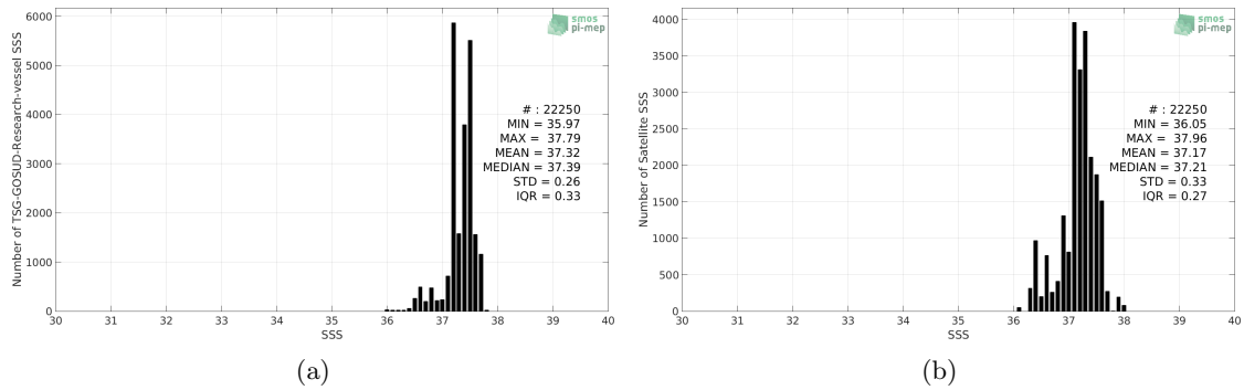
Figure 2: Histograms of SSS from TSG-GOSUD-Research-vessel (a) and SMOS-L3-CATDS-CECOS-IFREMER-V2-1DAY-0.5DEG (b) considering all match-up pairs per bins of 0.1 over the SPURS 1 Pi-MEP region and for the full satellite product period.
