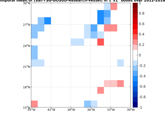
(e) MEAN( \Delta SSS) (Satellite - TSG-GOSUD-Research-vessel)
