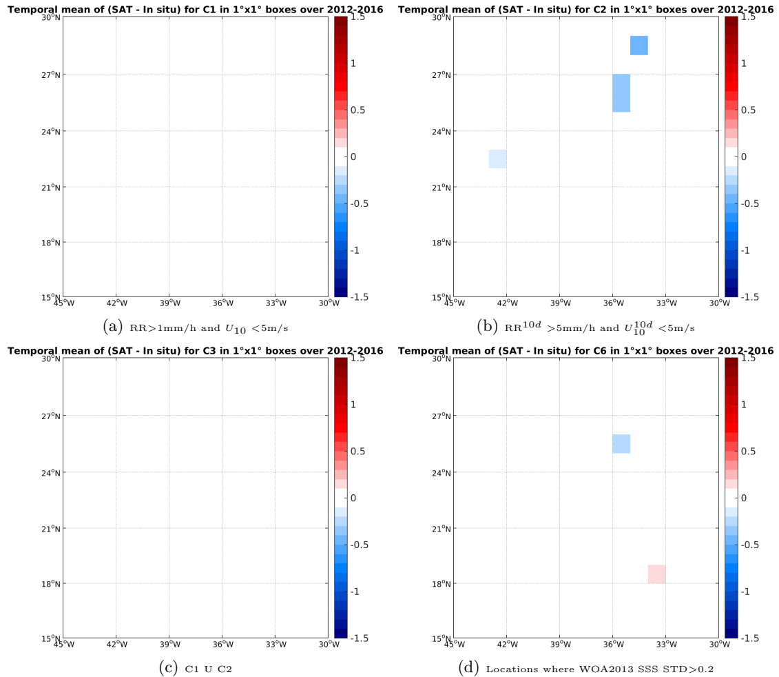
Figure 12: Temporal mean gridded over spatial boxes of size 1^\circ \times 1^\circ of \Delta SSS (SMOS-L3-CATDS-CECOS-IFREMER-V2-1DAY-0.5DEG - TSG-GOSUD-Research-vessel) for 4 different subdatasets corresponding to: RR > 1\text{mm/h} and U_{10} < 5\text{m/s} (a), RR^{10d} > 5\text{mm/h} and U_{10}^{10d} < 5\text{m/s} (b), C1 U C2 (c), Locations where WOA2013 SSS STD > 0.2 (d).
