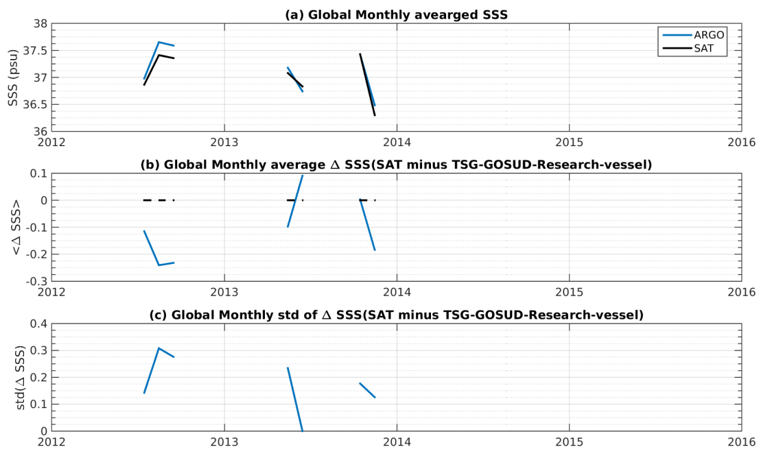
Figure 7: Time series of the monthly averaged mean SSS (top), mean \Delta SSS (Satellite - TSG-GOSUD-Research-vessel) and STD of \Delta SSS (Satellite - TSG-GOSUD-Research-vessel) over the SPURS 1 Pi-MEP region considering all match-ups collected by the Pi-MEP platform.
