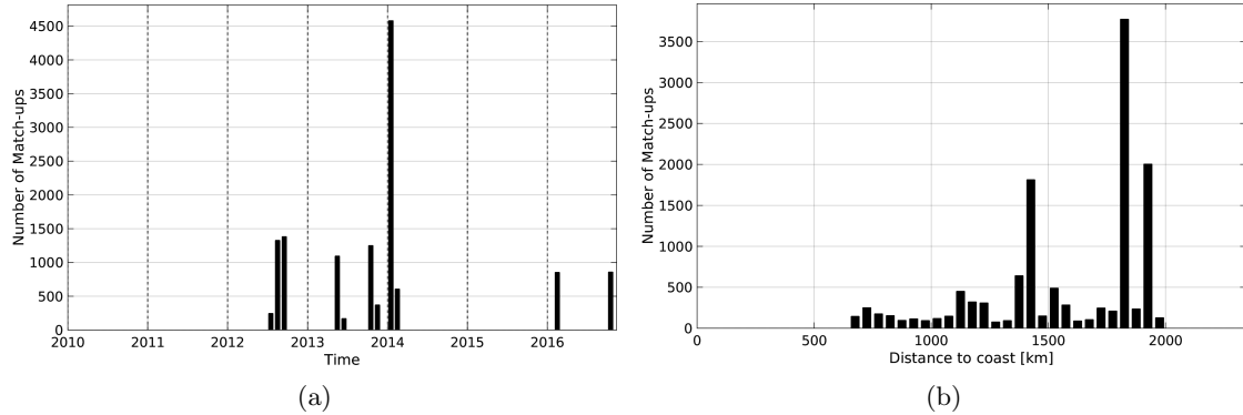
Figure 1: Number of match-ups between TSG-GOSUD-Research-vessel and SMOS-L3-CATDS-CECOS-IFREMER-V2-1DAY-0.5DEG SSS as a function of time (a) and as function of the distance to coast (b) over the SPURS 1 Pi-MEP region and for the full satellite product period.
