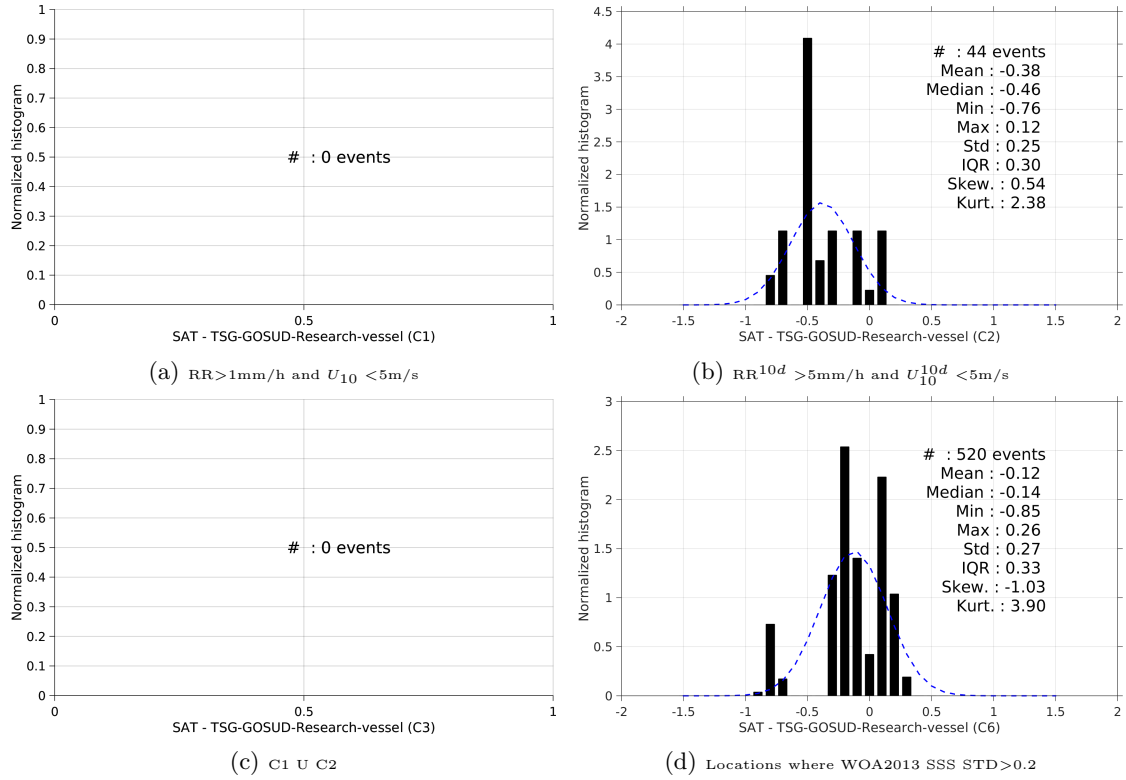
Figure 13: Normalized histogram of \Delta\text{SSS} (SMOS-L3-CATDS-CECOS-IFREMER-V2-1DAY-0.5DEG - TSG-GOSUD-Research-vessel) for 6 different subdatasets corresponding to: RR > 1\text{mm/h} and U_{10} < 5\text{m/s} (a), RR^{10d} > 5\text{mm/h} and U_{10}^{10d} < 5\text{m/s} (b), C1 \cup C2 (c), Locations where WOA2013 SSS STD > 0.2 (d).
