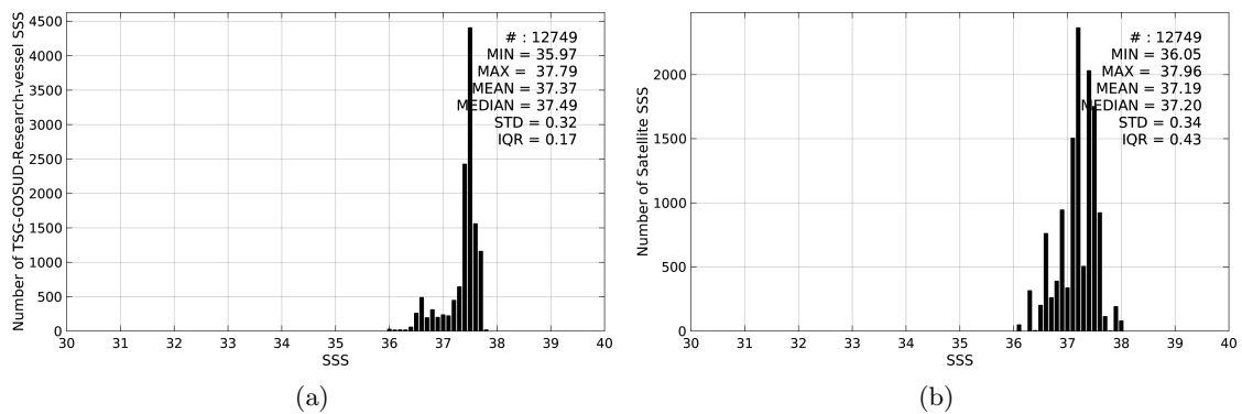
Figure 2: Histograms of SSS from TSG-GOSUD-Research-vessel (a) and SMOS-L3-CATDS-CECOS-IFREMER-V2-1DAY-0.5DEG (b) considering all match-up pairs per bins of 0.1 over the SPURS 1 Pi-MEP region and for the full satellite product period.
