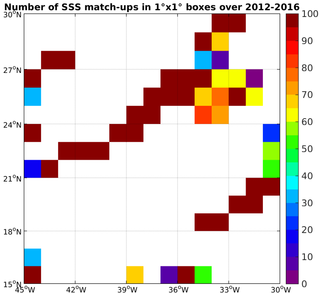
Figure 4: Number of SSS match-ups between TSG-GOSUD-Research-vessel SSS and the SMOS-L3-CATDS-CECOS-IFREMER-V2-1DAY-0.5DEG SSS product for the SPURS 1 Pi-MEP region over 1°x1° boxes and for the full satellite product period.
