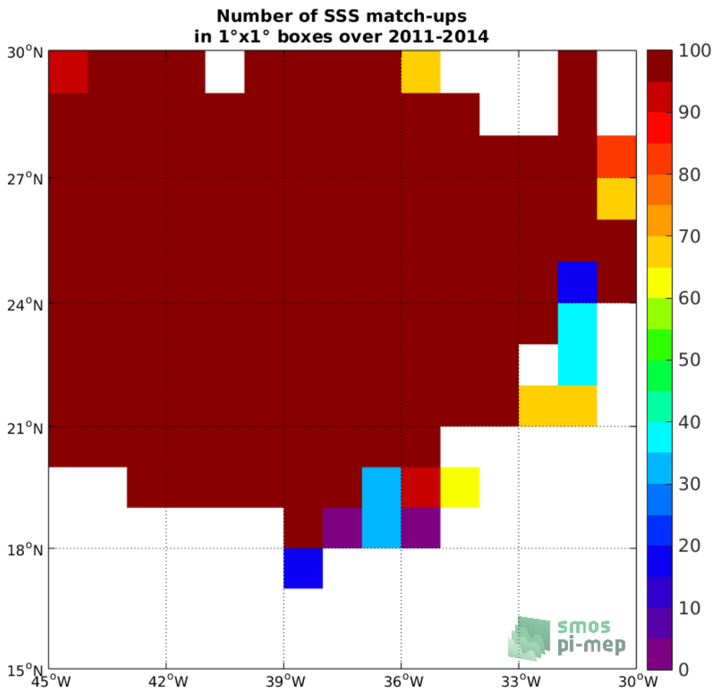
Figure 3: Number of SSS match-ups between Surface drifters SSS and the SMOS SSS L3 v2 - Daily - 0.5 Deg (CATDS-CECOS-IFREMER) SSS product for the SPURS 1 Pi-MEP region over 1°x1° boxes and for the full satellite product period.
