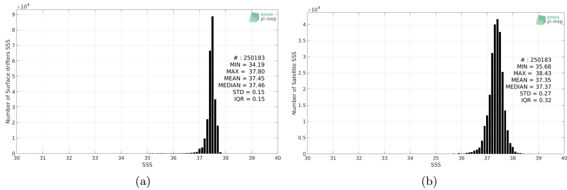
Figure 2: Histograms of SSS from Surface drifters (a) and SMOS SSS L3 v2 - Daily - 0.5 Deg (CATDS-CECOS-IFREMER) (b) considering all match-up pairs per bins of 0.1 over the SPURS 1 Pi-MEP region and for the full satellite product period.
