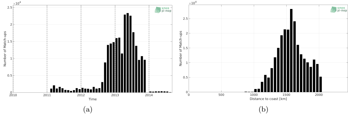
Figure 1: Number of match-ups between Surface drifters and SMOS SSS L3 v2 - Daily - 0.5 Deg (CATDS-CECOS-IFREMER) SSS as a function of time (a) and as function of the distance to coast (b) over the SPURS 1 Pi-MEP region and for the full satellite product period.
