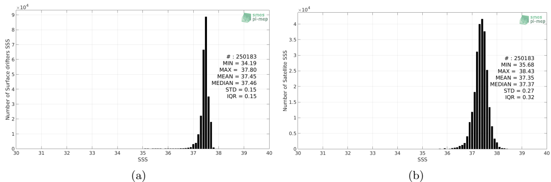
Figure 2: Histograms of SSS from Surface drifters (a) and SMOS L3 v2 - Daily - 0.5 Deg (CATDS-CECOS-IFREMER) (b) considering all match-up pairs per bins of 0.1 over the SPURS 1 Pi-MEP region and for the full satellite product period.
