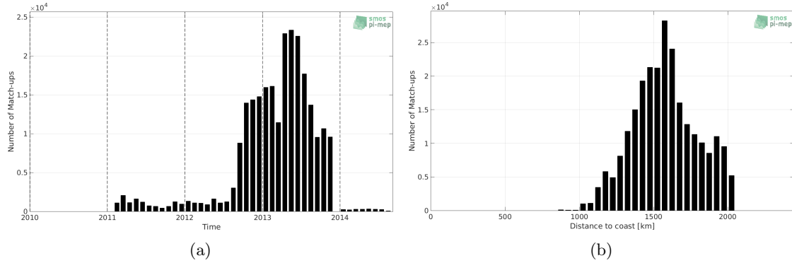
Figure 1: Number of match-ups between Surface drifters and SMOS L3 v2 - Daily - 0.5 Deg (CATDS-CECOS-IFREMER) SSS as a function of time (a) and as function of the distance to coast (b) over the SPURS 1 Pi-MEP region and for the full satellite product period.
