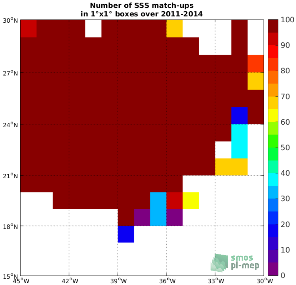
Figure 3: Number of SSS match-ups between Surface drifters SSS and the SMOS L3 v2 - Daily - 0.5 Deg (CATDS-CECOS-IFREMER) SSS product for the SPURS 1 Pi-MEP region over 1°x1° boxes and for the full satellite product period.
